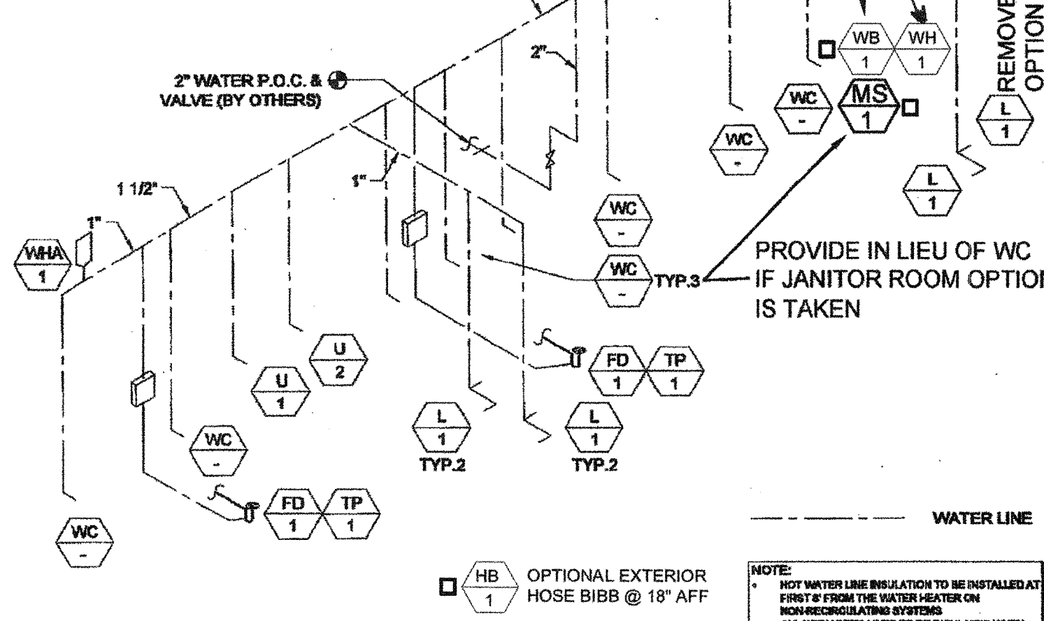
MODEL C-2 SUPPLY ISOMETRIC - FLOOR AND WALL MOUNT SCALE: N.T.S. 8
