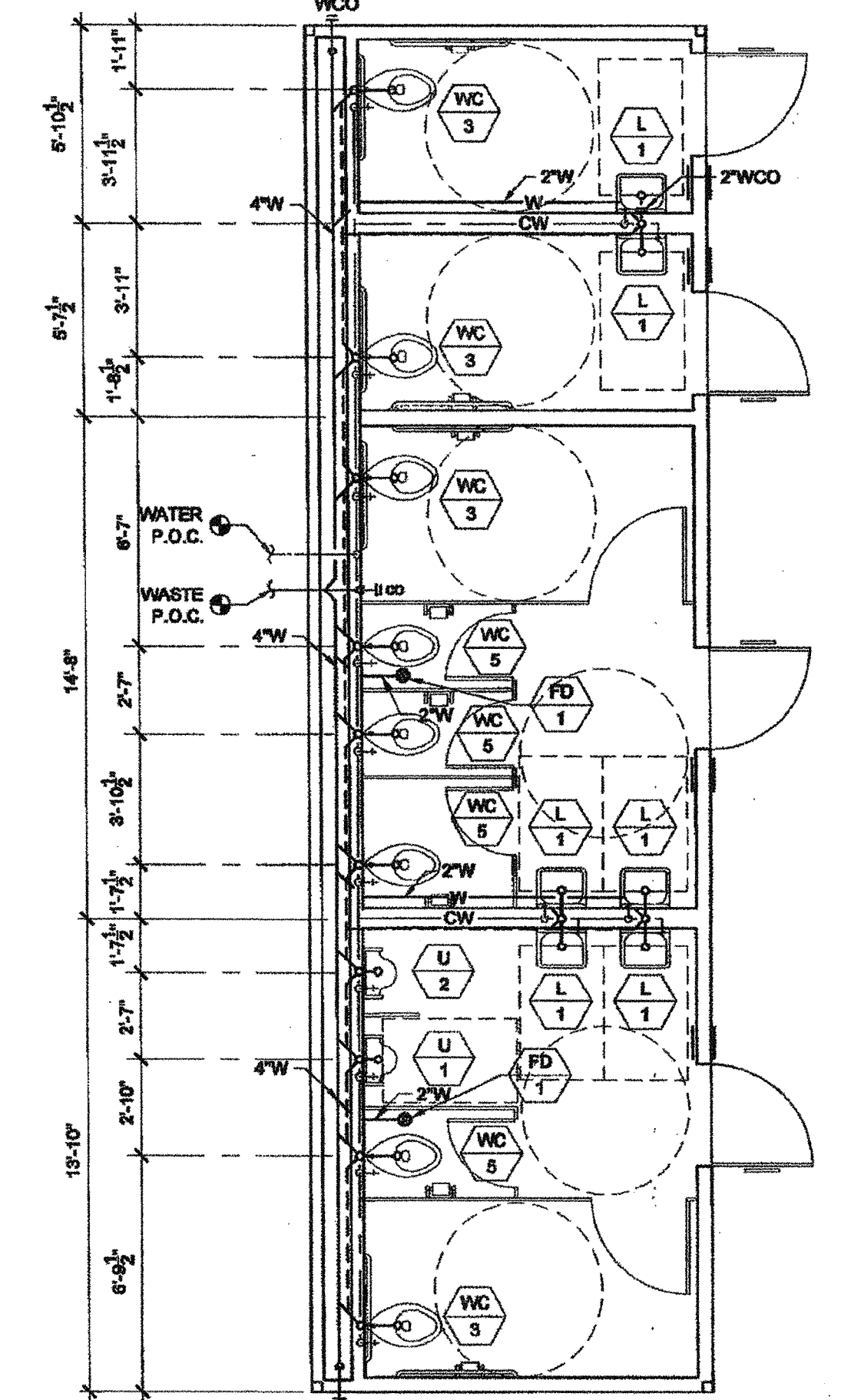
FLOOR MOUNT - MODEL C-2 PLUMBING PLAN SCALE: 1/4" = 1'-0" 7
