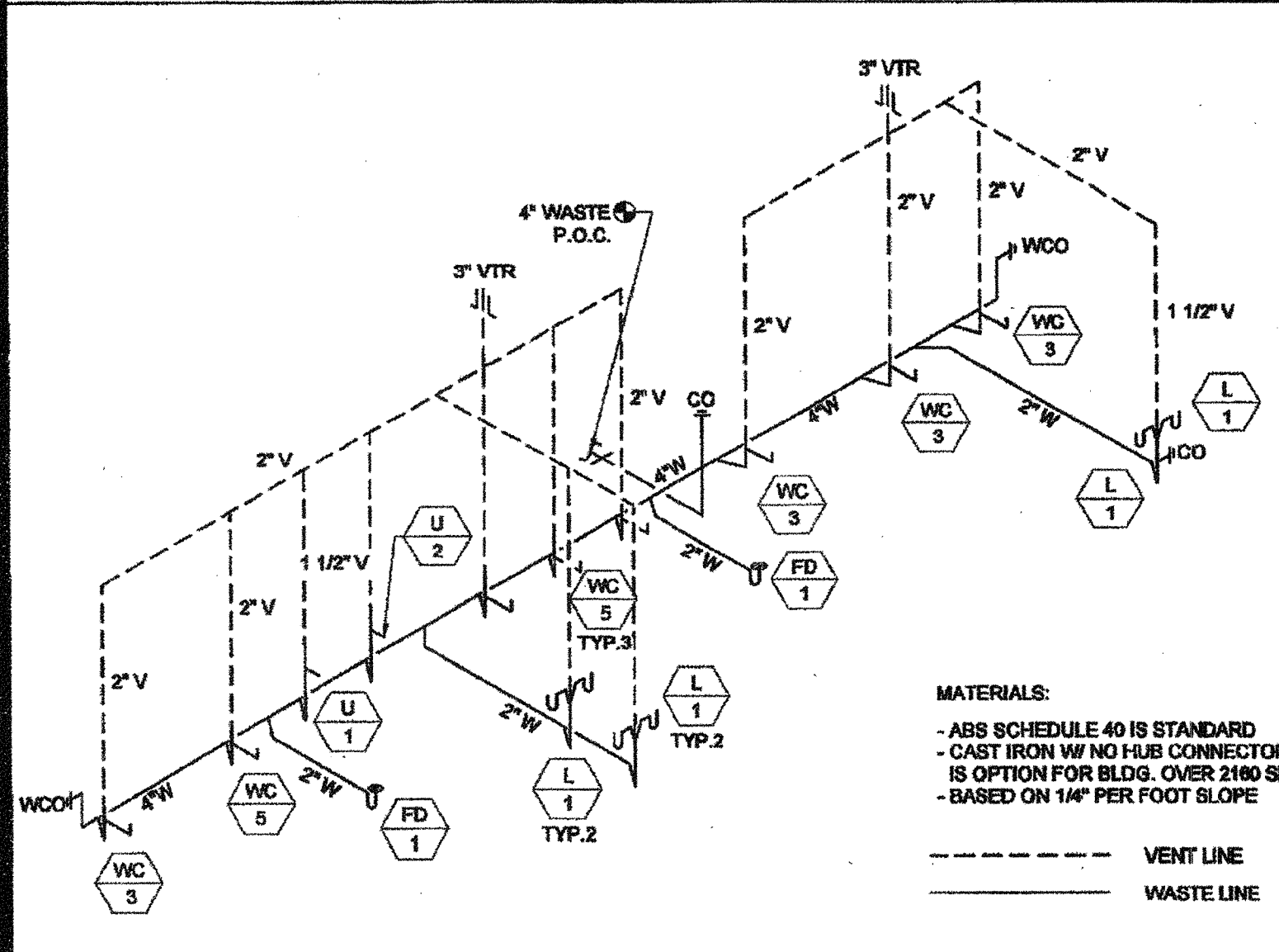
MODEL C-2 WASTE AND VENTING ISOMETRIC - FLOOR MOUNT SCALE: N.T.S. 10
