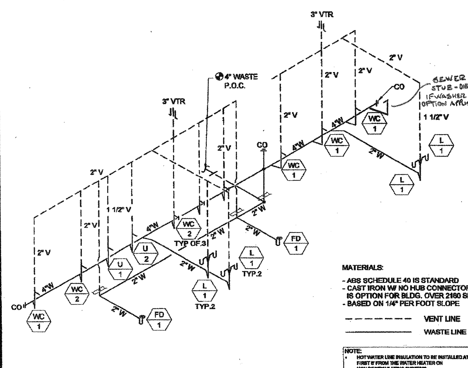
MODEL C-2 WASTE AND VENTING ISOMETRIC - WALL MOUNT SCALE: N.T.S. 9
