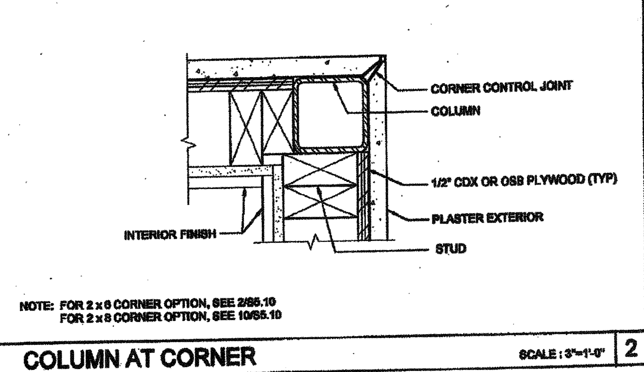
COLUMN AT CORNER SCALE: 3/4"=1'-0" 2
