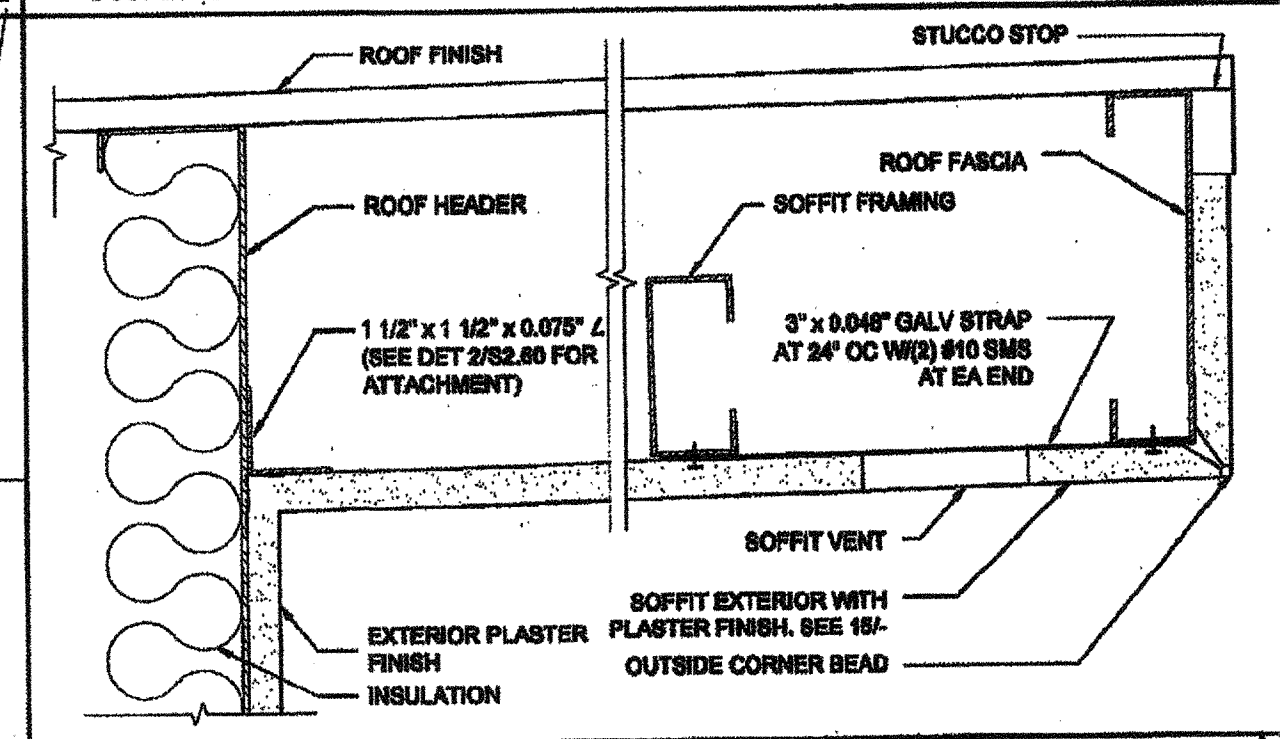
SOFFIT AT ROOF HEADER WITH VENT SCALE: 3/4"=1'-0" 14
