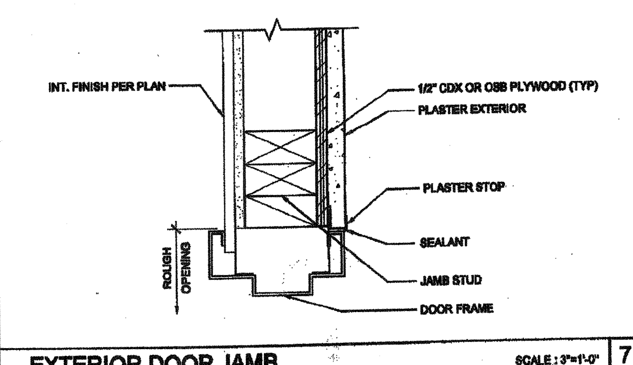
EXTERIOR DOOR JAMB SCALE: 3/4"=1'-0" 7
