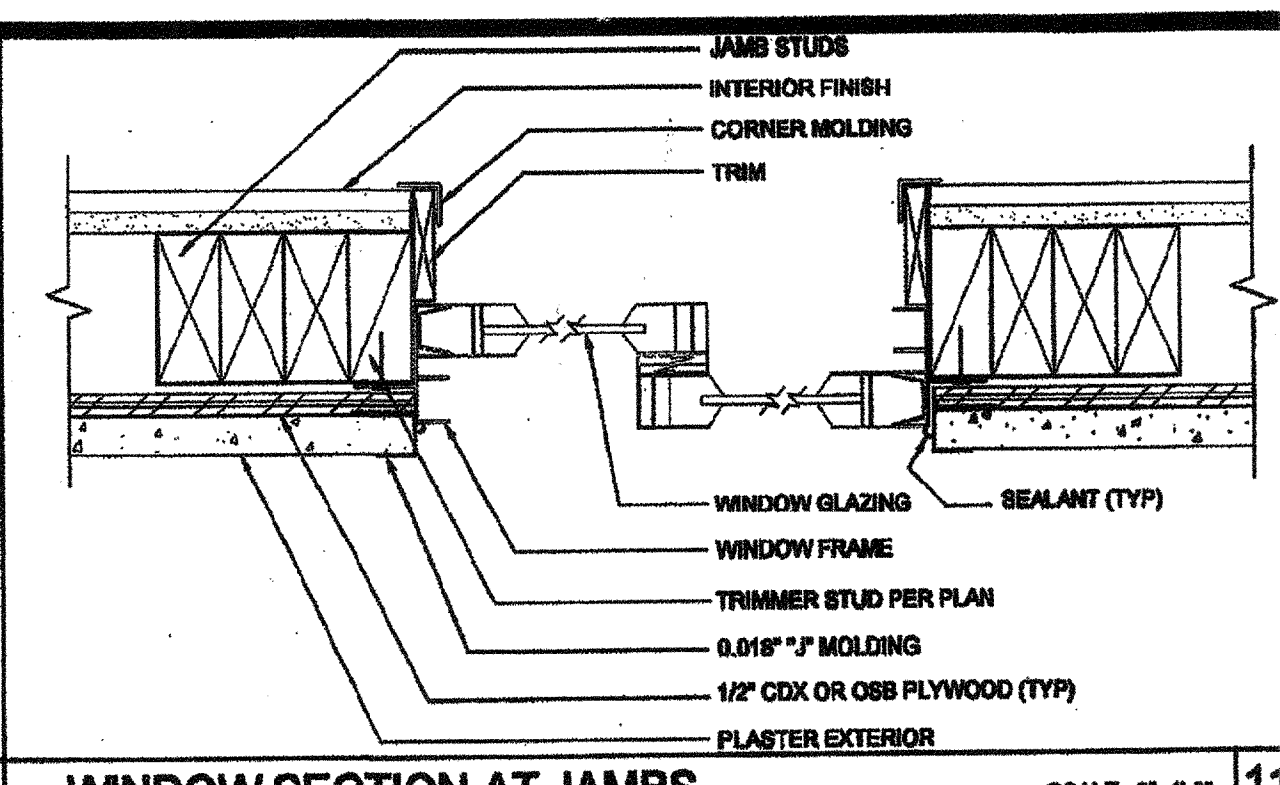
WINDOW SECTION AT JAMBS SCALE: 3/4"=1'-0" 11
