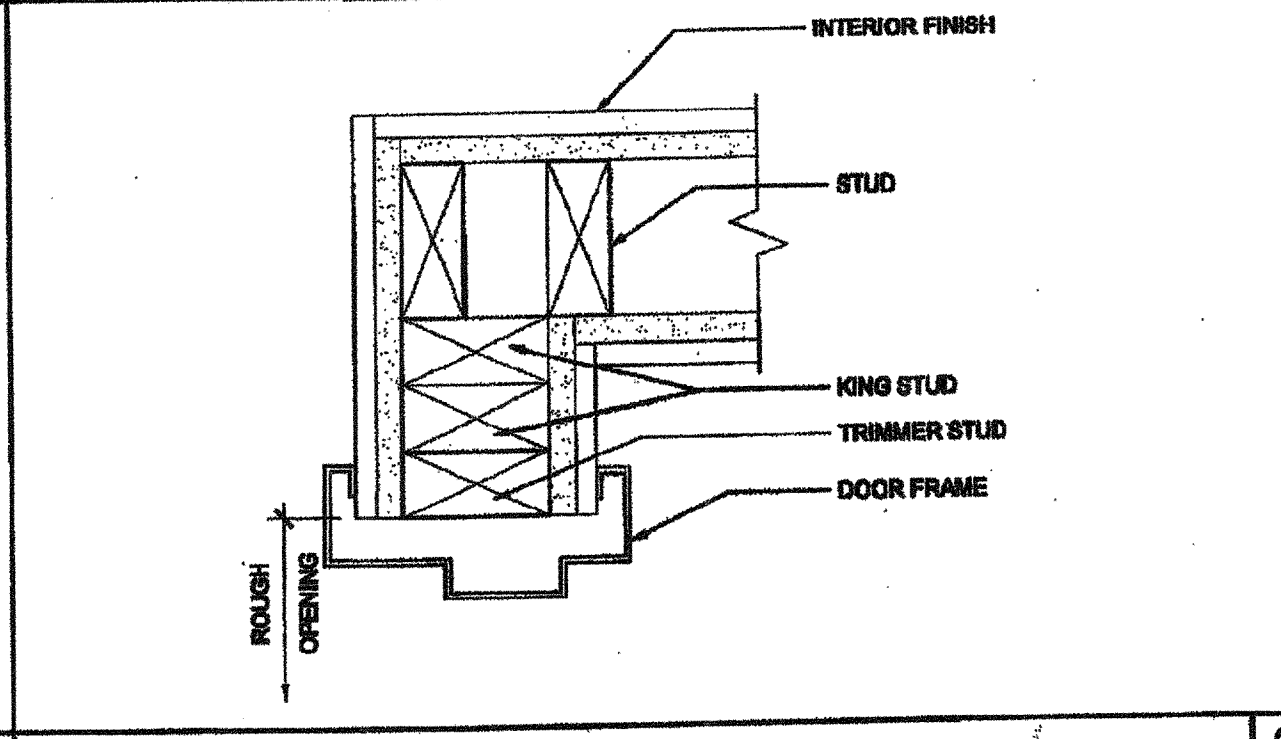
INTERIOR DOOR JAMB SCALE: 3/4"=1'-0" 9
