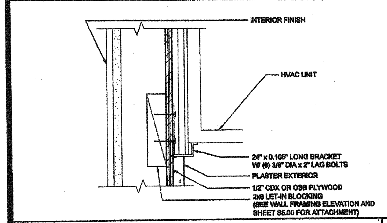
HVAC UNIT AT BOTTOM SCALE: 3/4"=1'-0" 17
