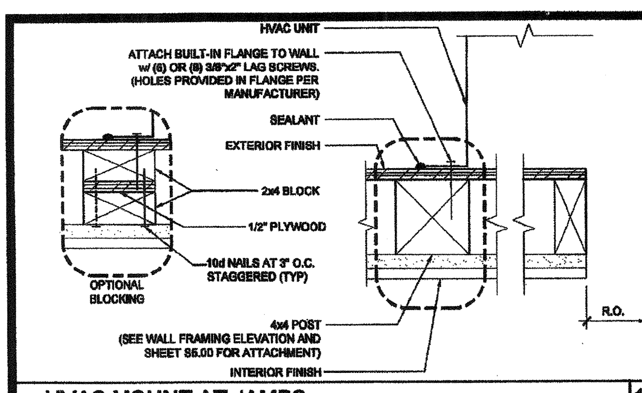
HVAC MOUNT AT JAMBS SCALE: 3/4"=1'-0" 16
