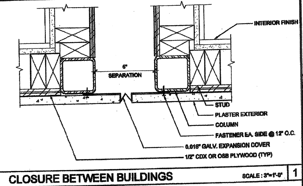
CLOSURE BETWEEN BUILDINGS SCALE: 3/4"=1'-0" 1
