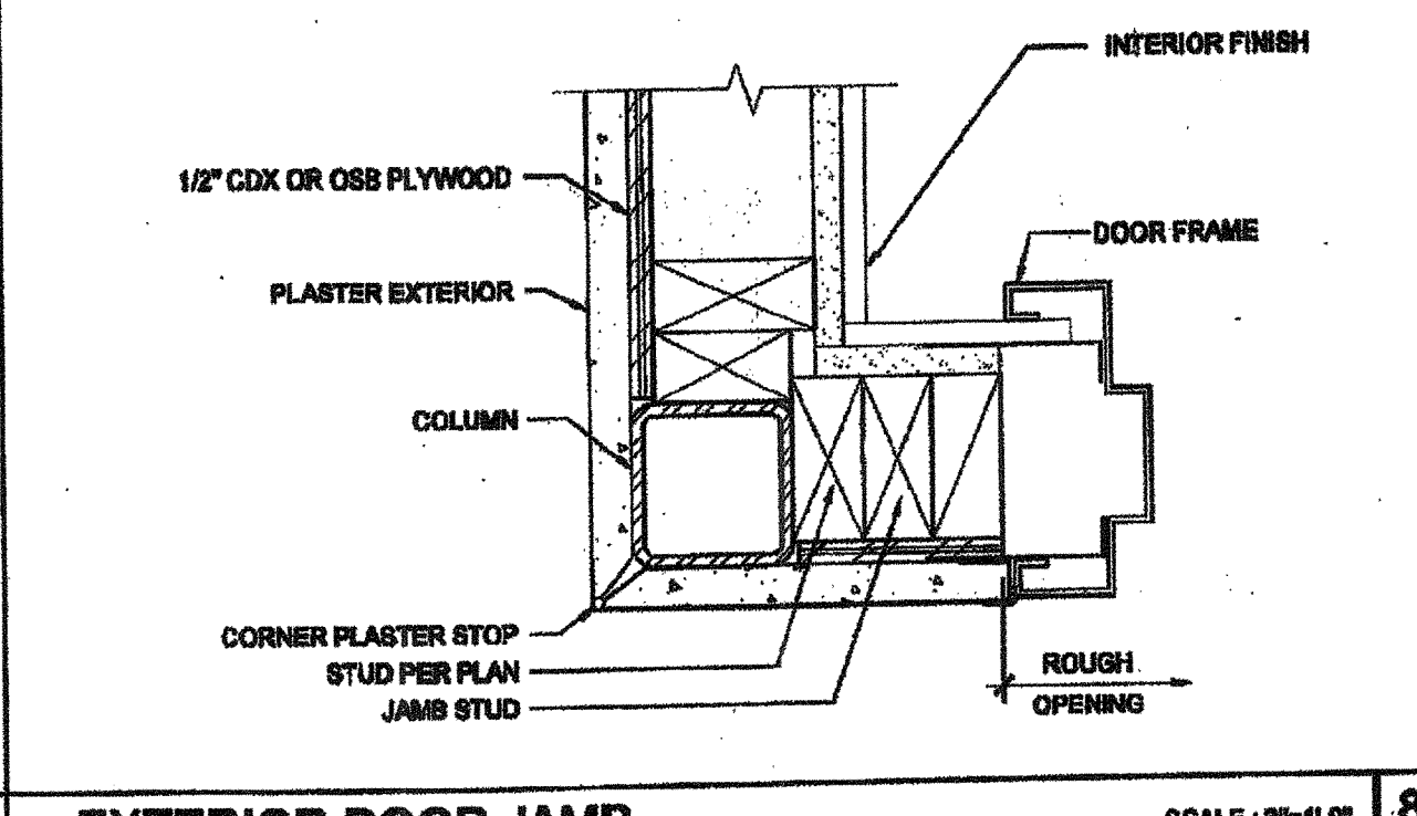
EXTERIOR DOOR JAMB SCALE: 3/4"=1'-0" 8
