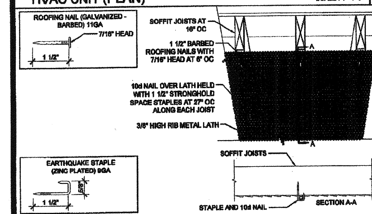
METAL LATH ATTACHMENT TO WOOD JOIST SCALE: 1/2"=1'-0" 19
