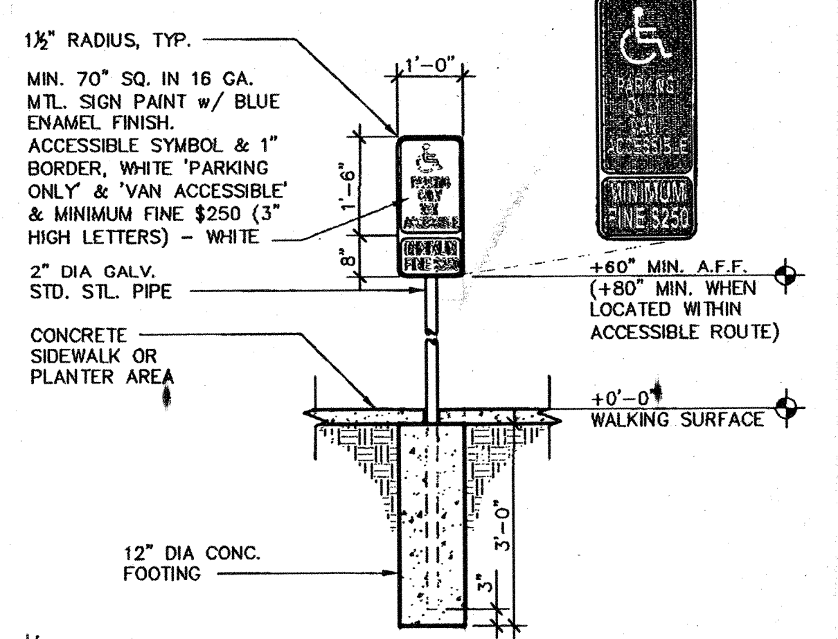
16 VAN ACCESSIBLE PARKING SIGNAGE A1.04 ADA100-50
