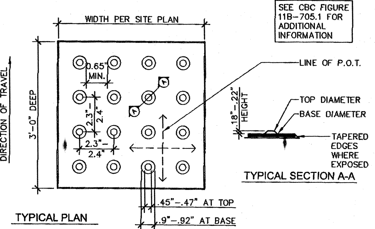
15 TRUNCATED DOMES A1.04 ADA100-23
