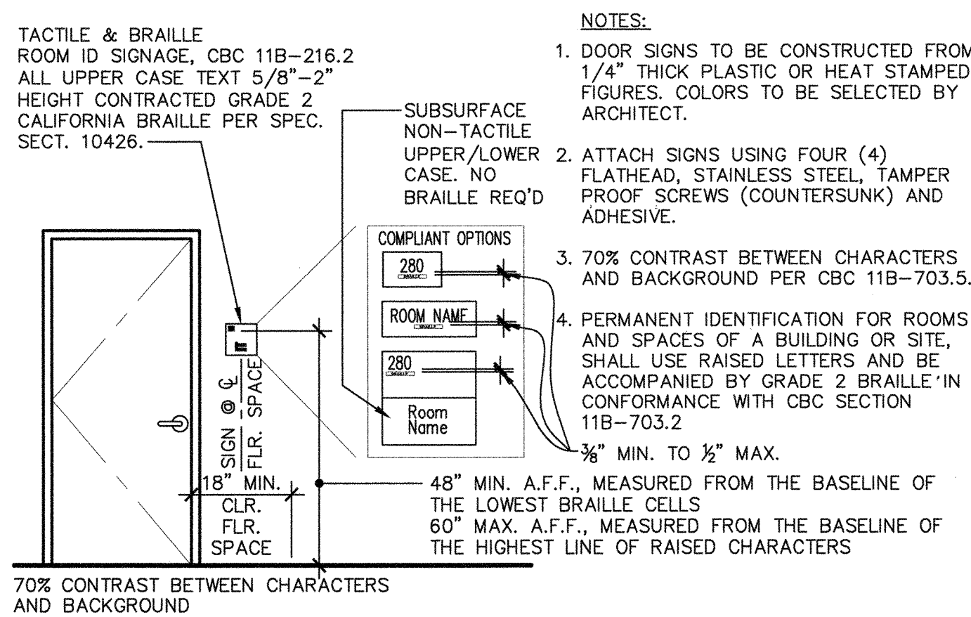
2 ROOM ID SIGNAGE A1.04 ADX100-01
