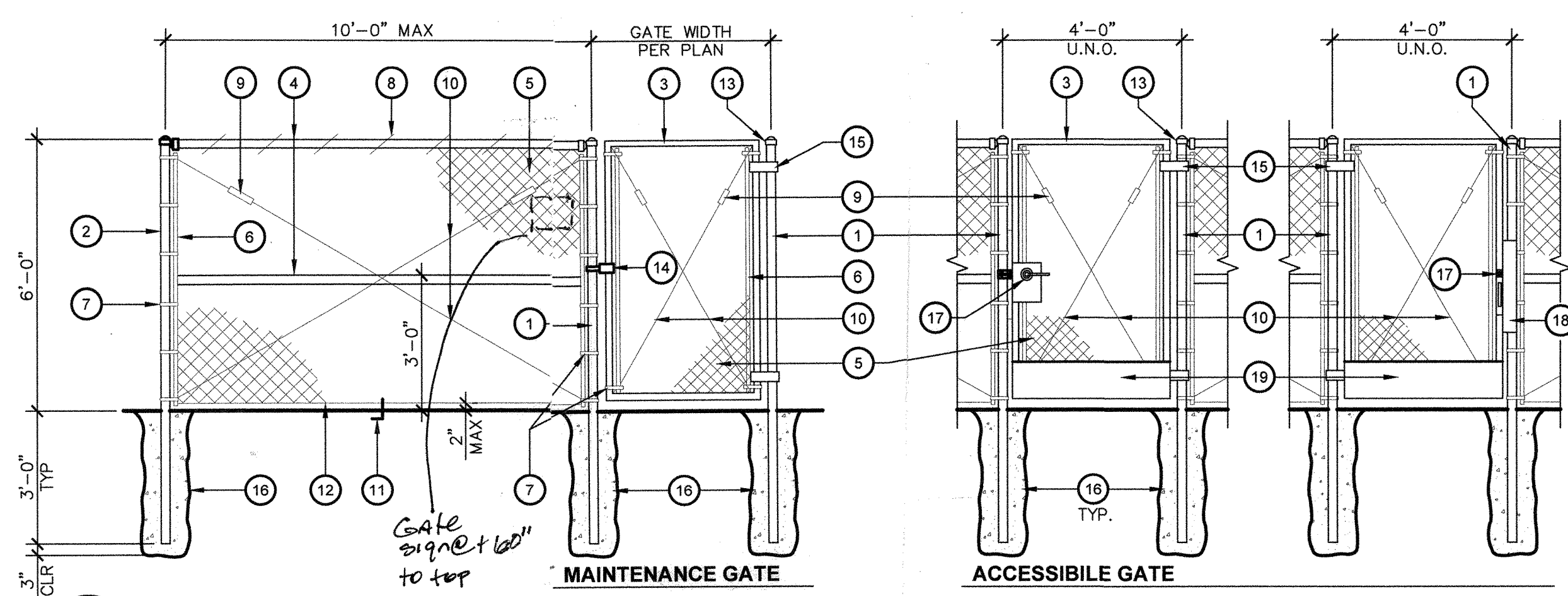
13 TYPICAL CHAIN LINK FENCE AND GATES A1.04 ADA100-01
