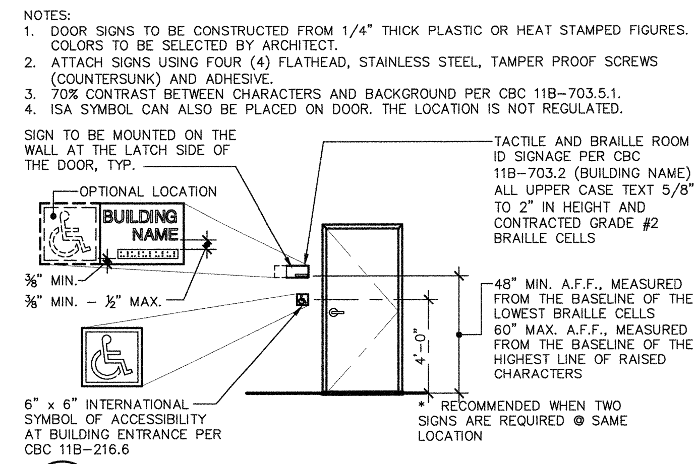
1 BUILDING ENTRANCE/I.S.A. SIGNAGE A1.04 ADA100-01
