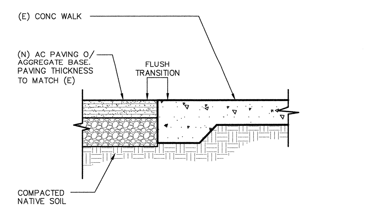
8 (E) CONC WALK TO (N) AC PAVING A1.04 ADS100-27
