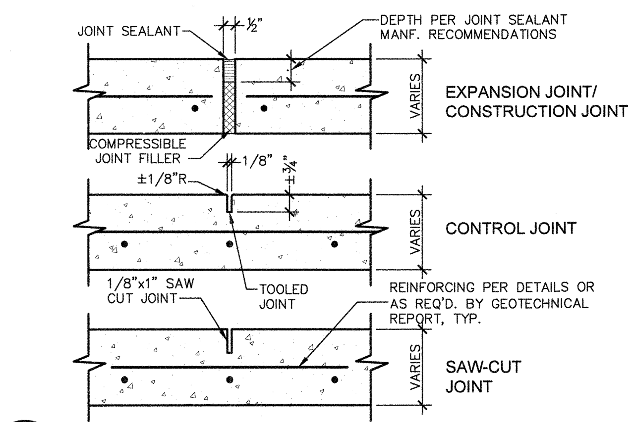
7 CONCRETE JOINTS A1.04 ADS110-01
