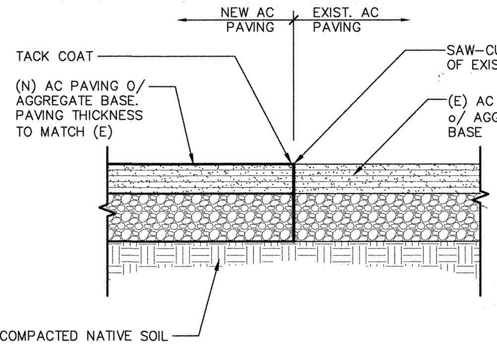
11 (N) AC PAVING TO (E) AC PAVING A1.04 ADS100-07
