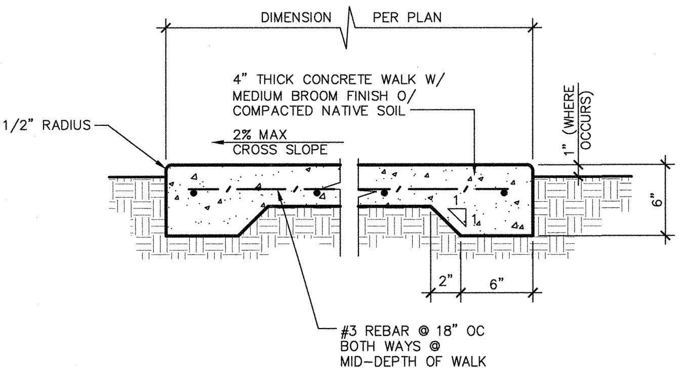
6 TYPICAL CONCRETE WALK A1.04 ADS100-03
