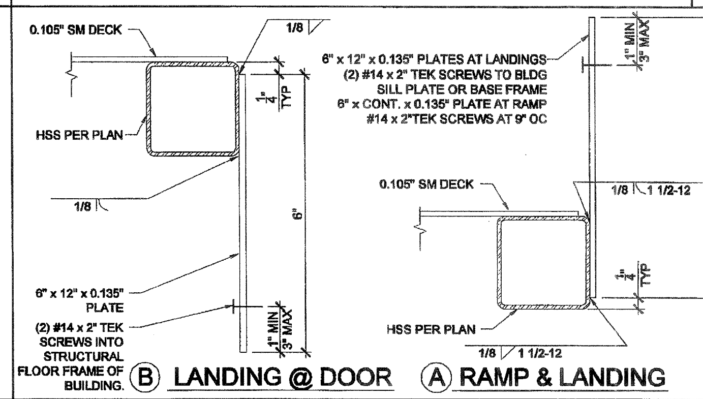
RAMP AT LANDING SCALE: 6" = 1'-0" 12
