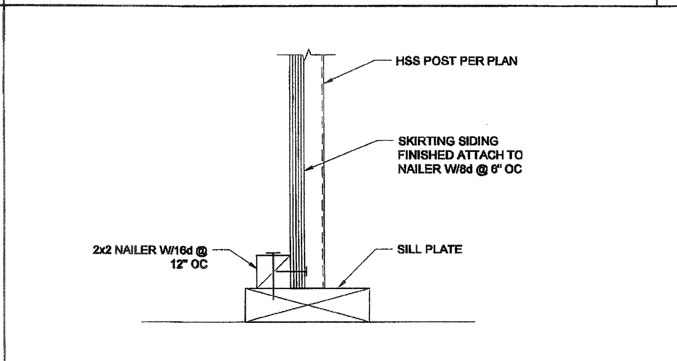
SKIRT FLASHING AT SILL PLATE SCALE: 3" = 1'-0" 6
