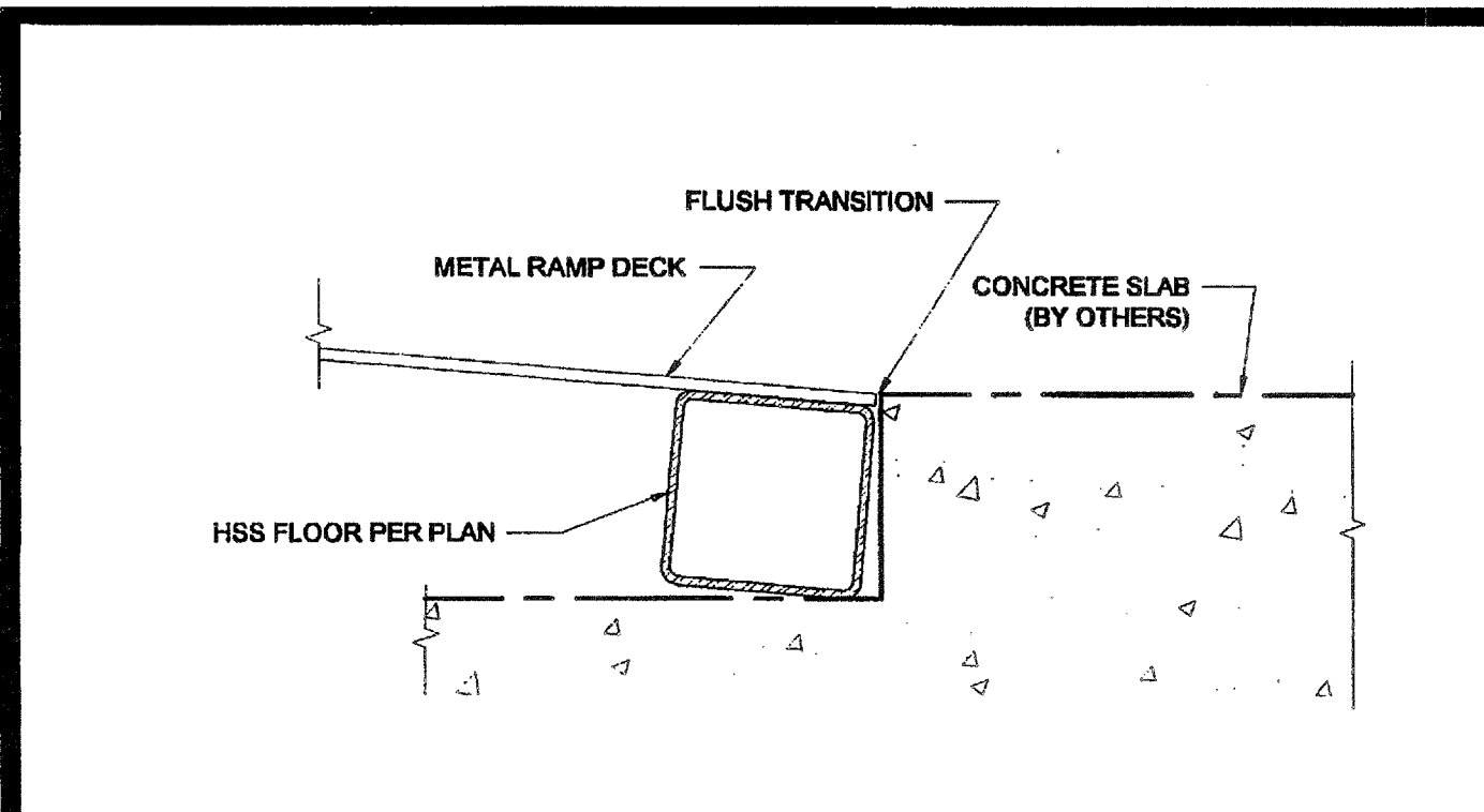
FLUSH TRANSITION AT BOTTOM OF RAMP SCALE: 6" = 1'-0" 15
