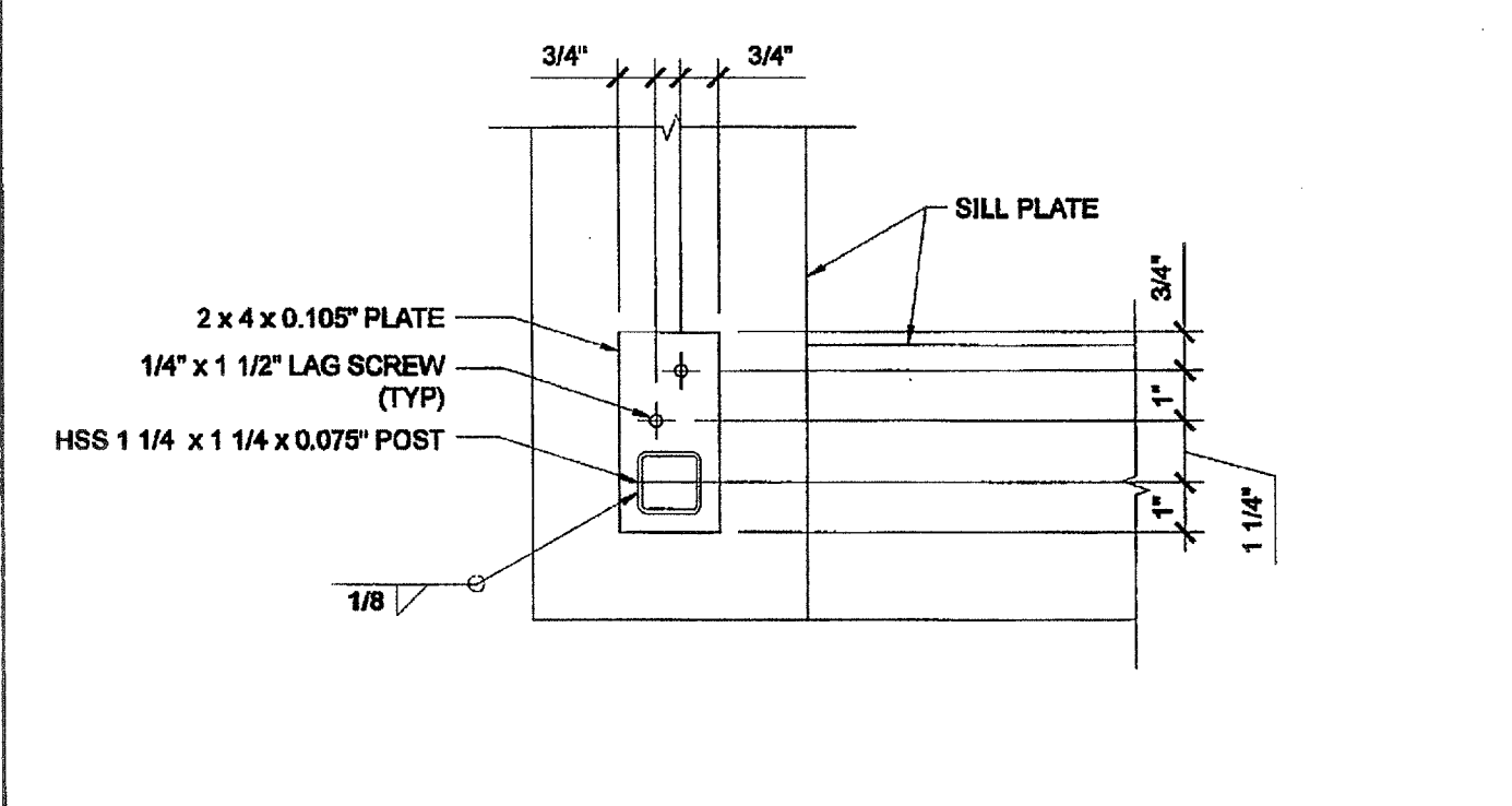
GUARDRAIL POST ATTACHMENT SCALE: 6" = 1'-0" 4
