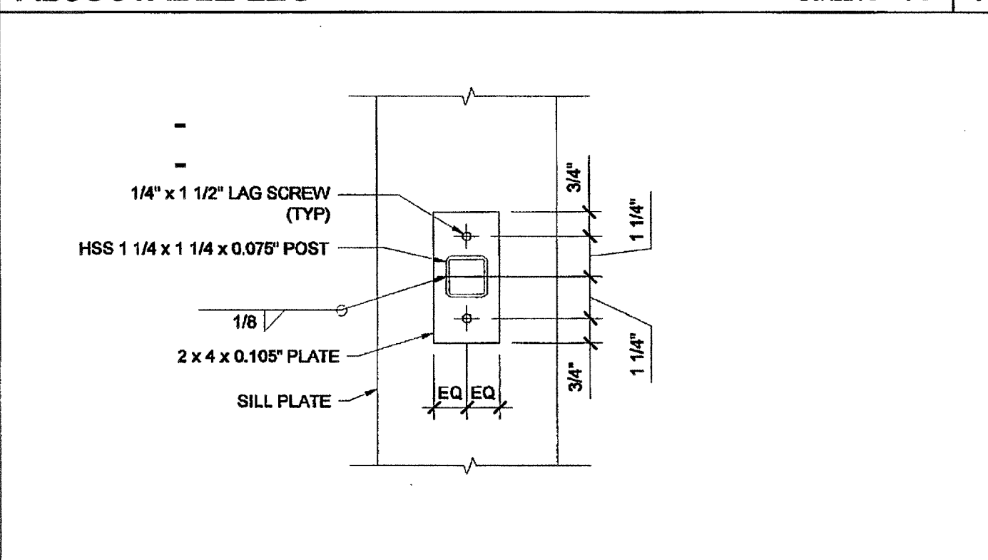
ADJUSTABLE LEG BASE PLATE SCALE: 3" = 1'-0" 3
