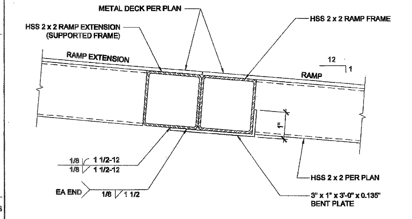
ADJUSTABLE LEG BASE PLATE SCALE: 3" = 1'-0" 3
