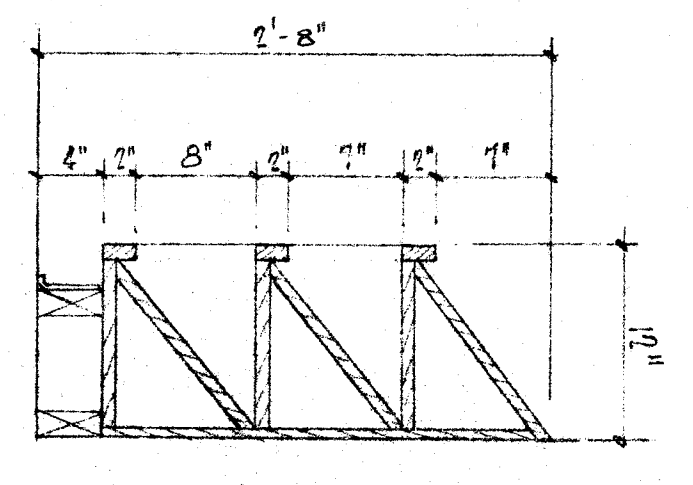
2. SLANTING BOOK SHELVES SCALE: 1/4" = 1'-0"
