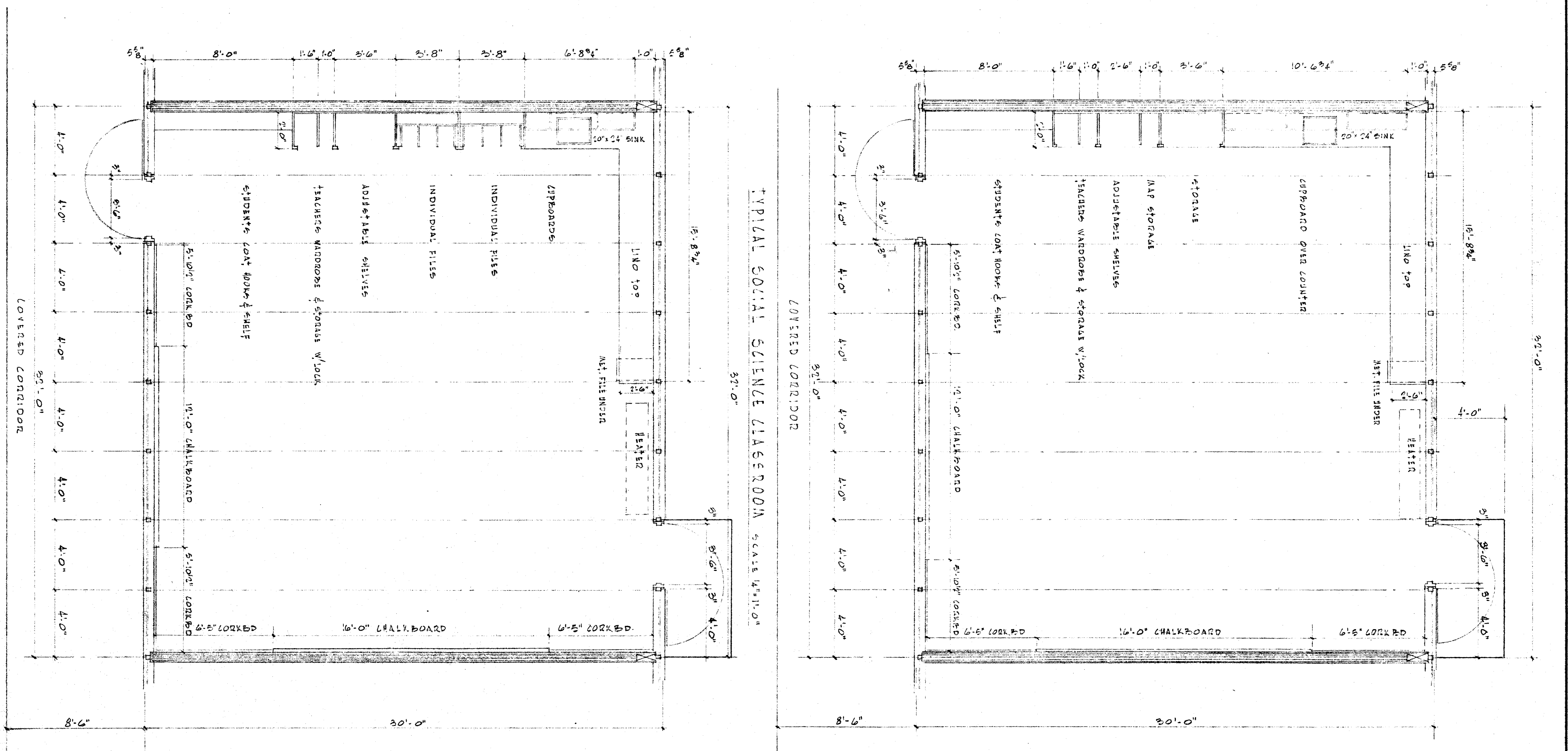
TYPICAL ENGLISH CLASSROOM SCALE 1/4" = 1'-0"
