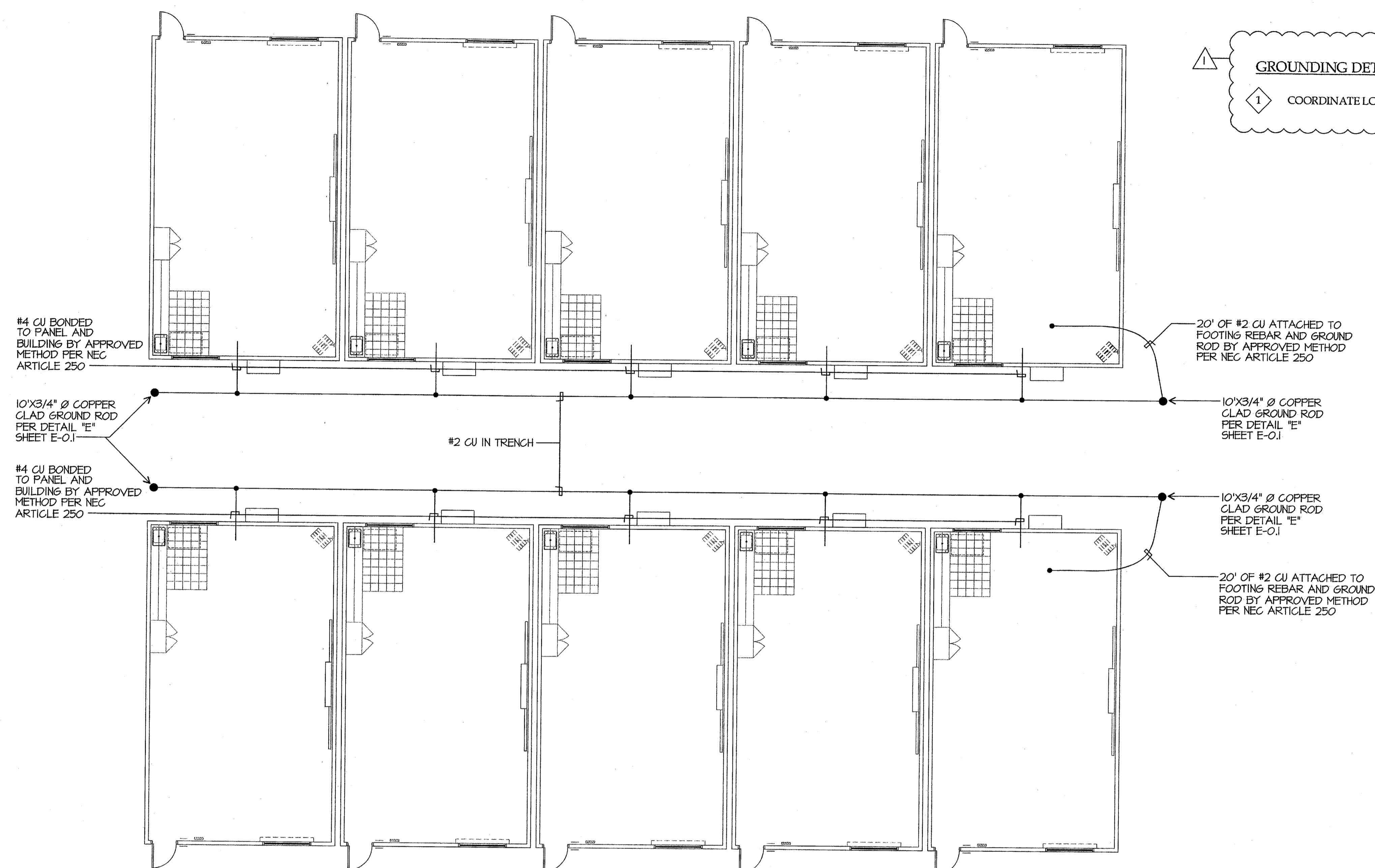
GROUNDING DETAIL
