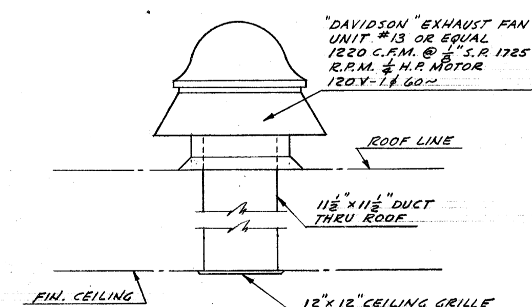
SECTION - P - P SCALE 3/8" = 1'-0"
