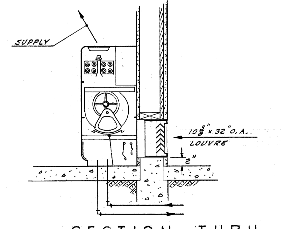
SECTION THRU UNIT VENTILATOR SCALE 3/8" = 1'-0"
