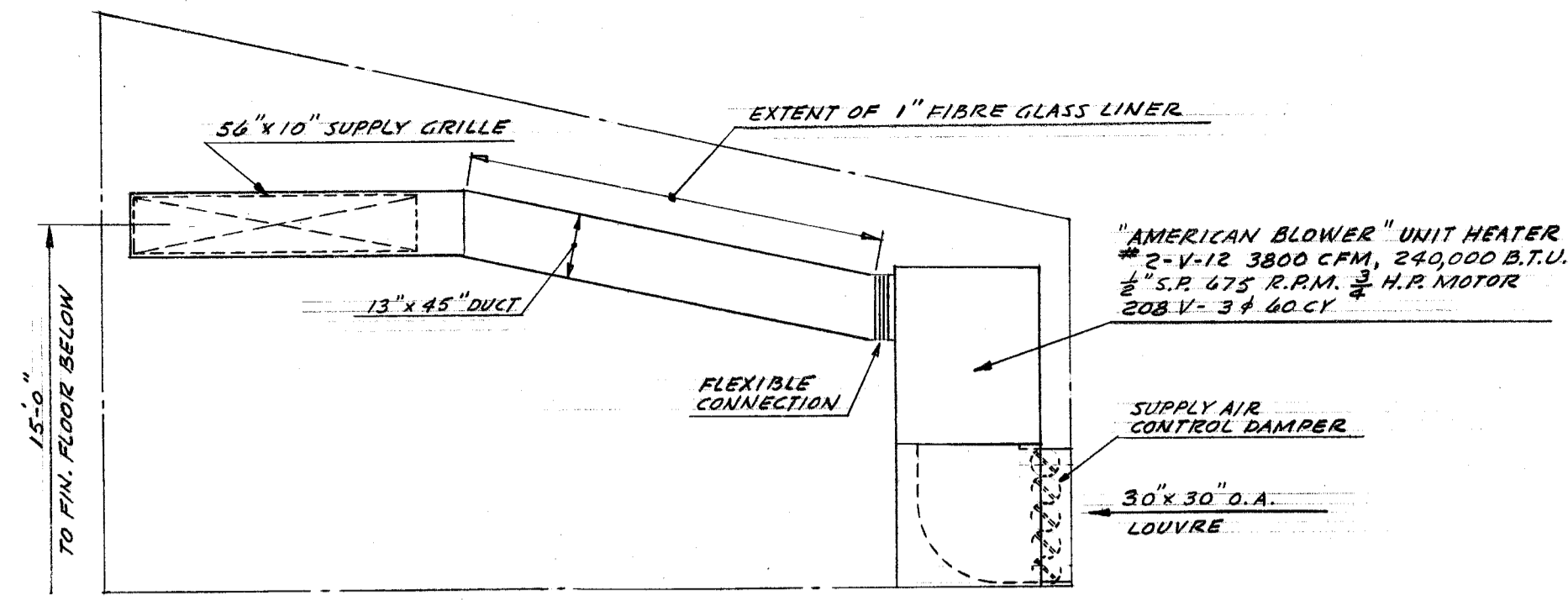
SECTION - I - I SCALE 3/8" = 1'-0"
