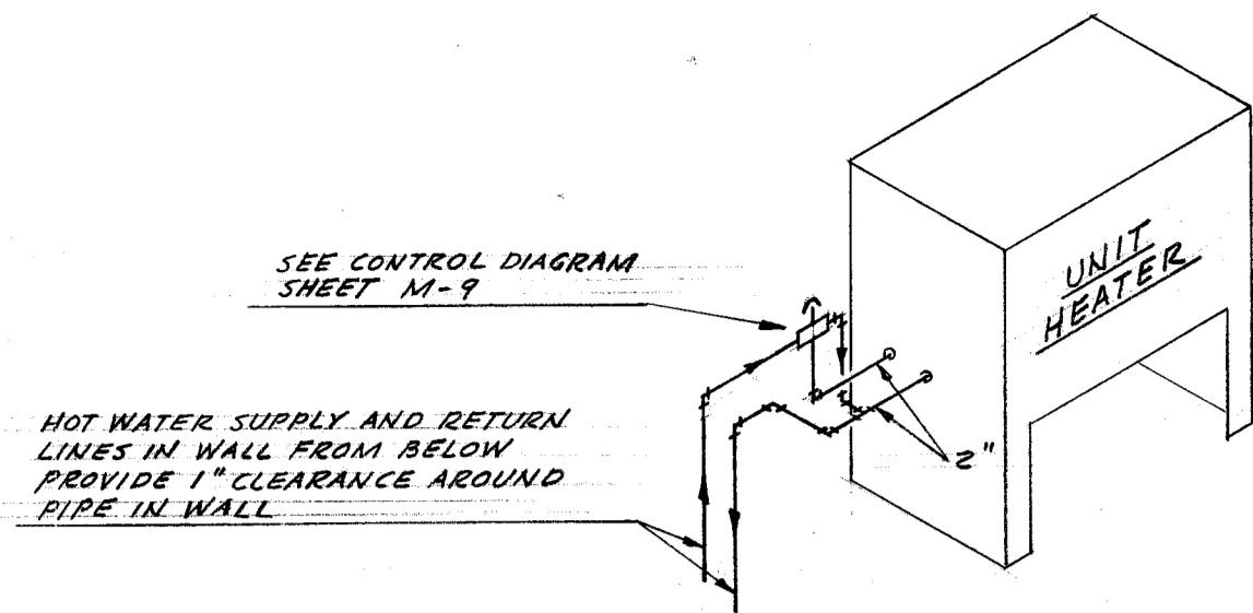
ISOMETRIC SHOWING PIPE CONNECTIONS @ UNIT HEATER NO SCALE
