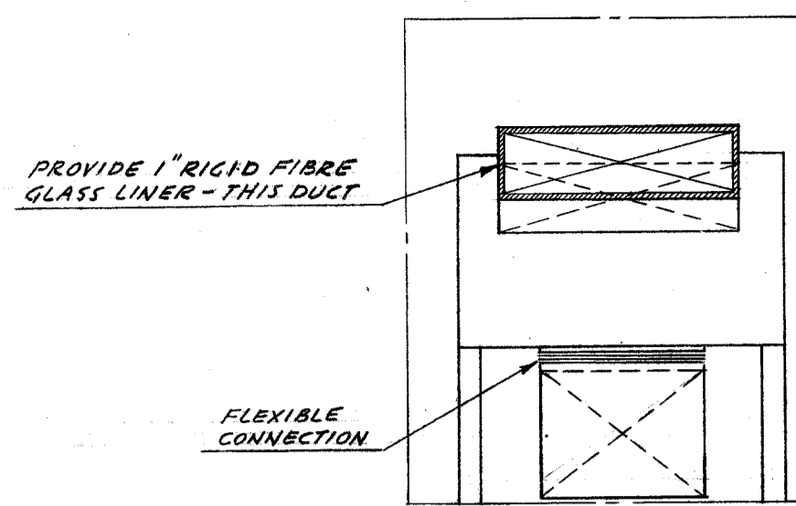
SECTION - J - J SCALE 3/8" = 1'-0"
