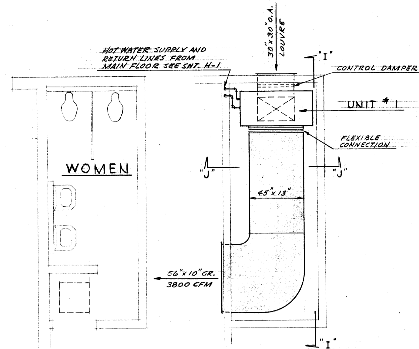
PLAN OF HEATER ROOM ABOVE TOILET ROOM SCALE 1/4" = 1'-0"
