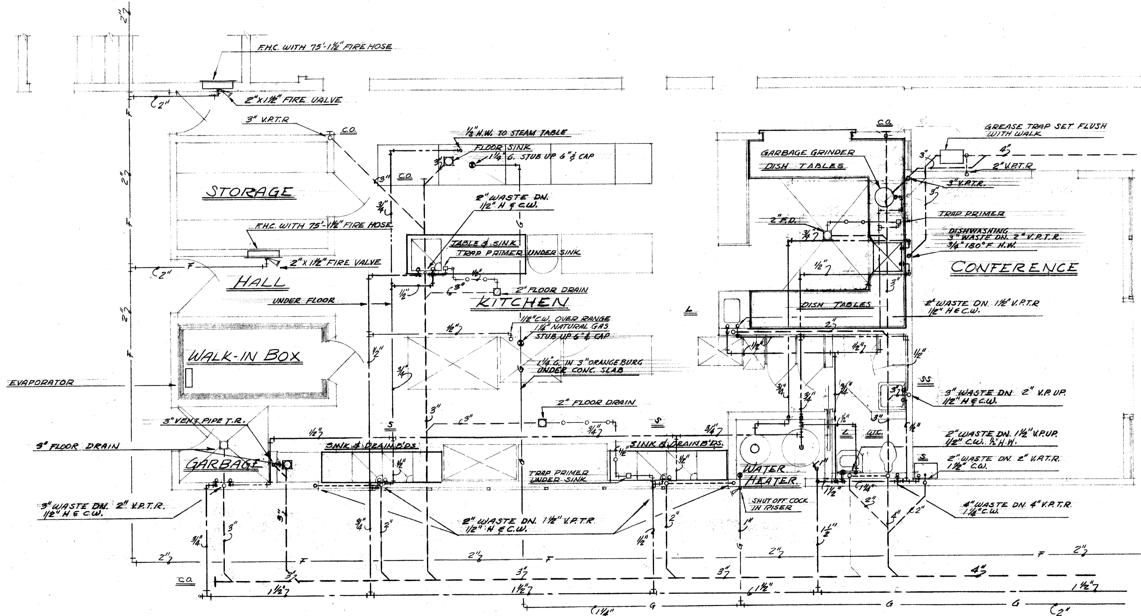
FLOOR PLAN KITCHEN - UNIT-1 SCALE 1/4" = 1'-0"
