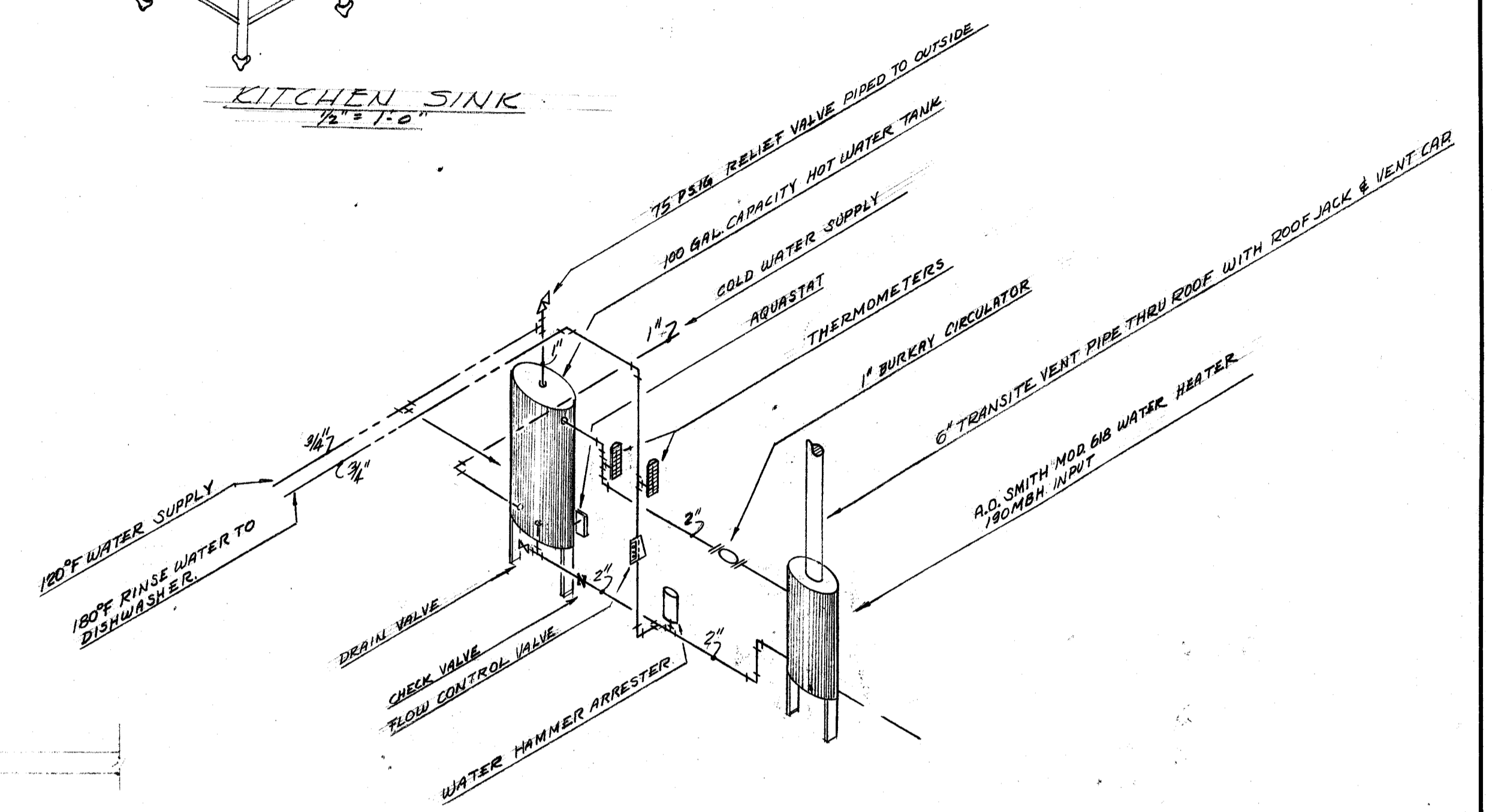
SCHEMATIC PIPING LAYOUT OF A.O. SMITH TWO TEMPERATURE WATER HEATING SYSTEM. NOT TO SCALE
