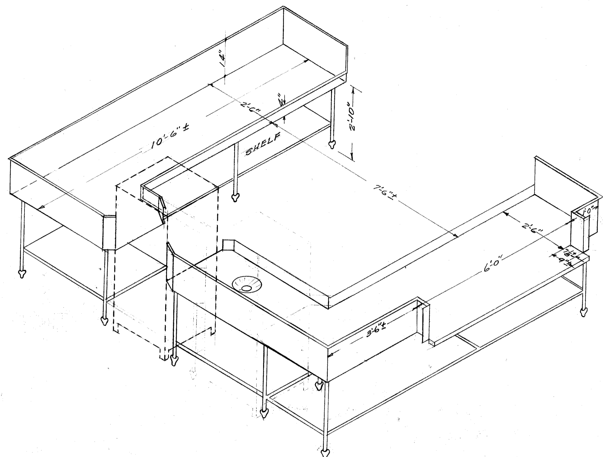
DISH TABLES 1/4" = 1'-0"
