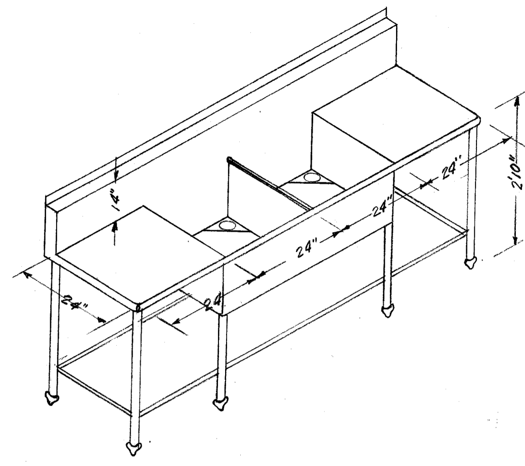
KITCHEN SINK 1/4" = 1'-0"
