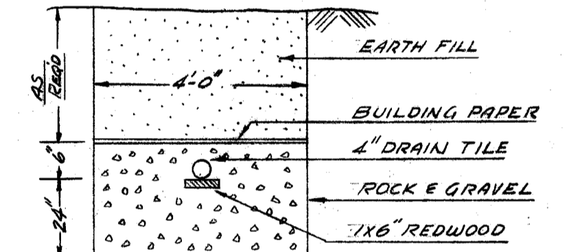
SECTION I-I THRU LEECHING LINES
