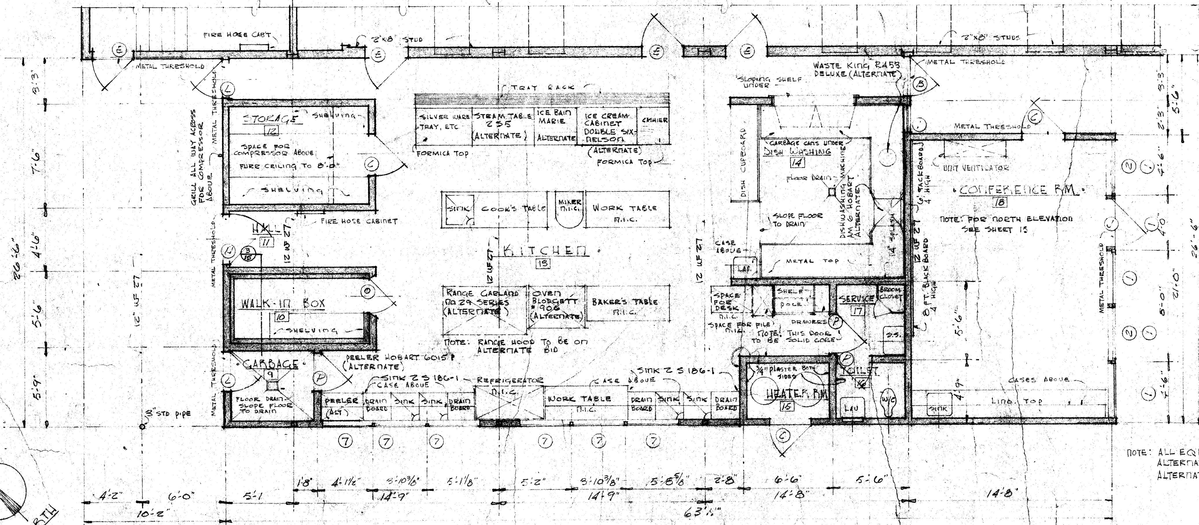
FLOOR PLAN SCALE 1/4" = 1'-0" NOTE: ALL STUD 2"x4" UNLESS OTHERWISE SHOWN
