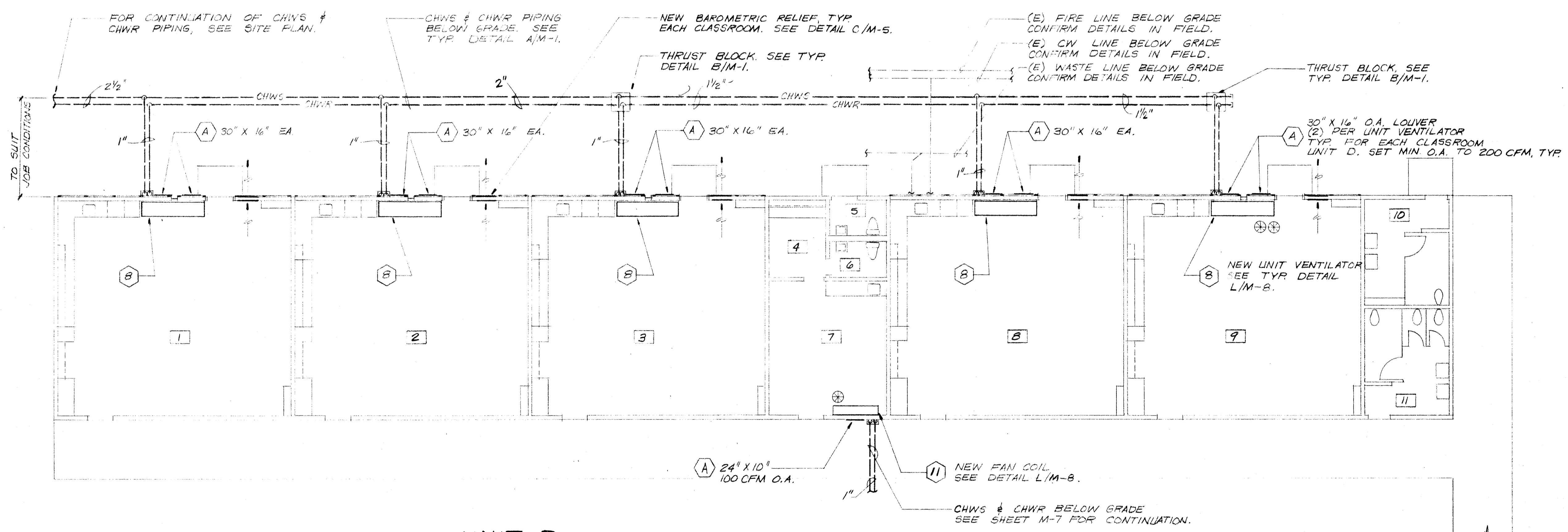
UNIT D AIR CONDITIONING PLAN SCALE: 1/8" = 1'-0"
