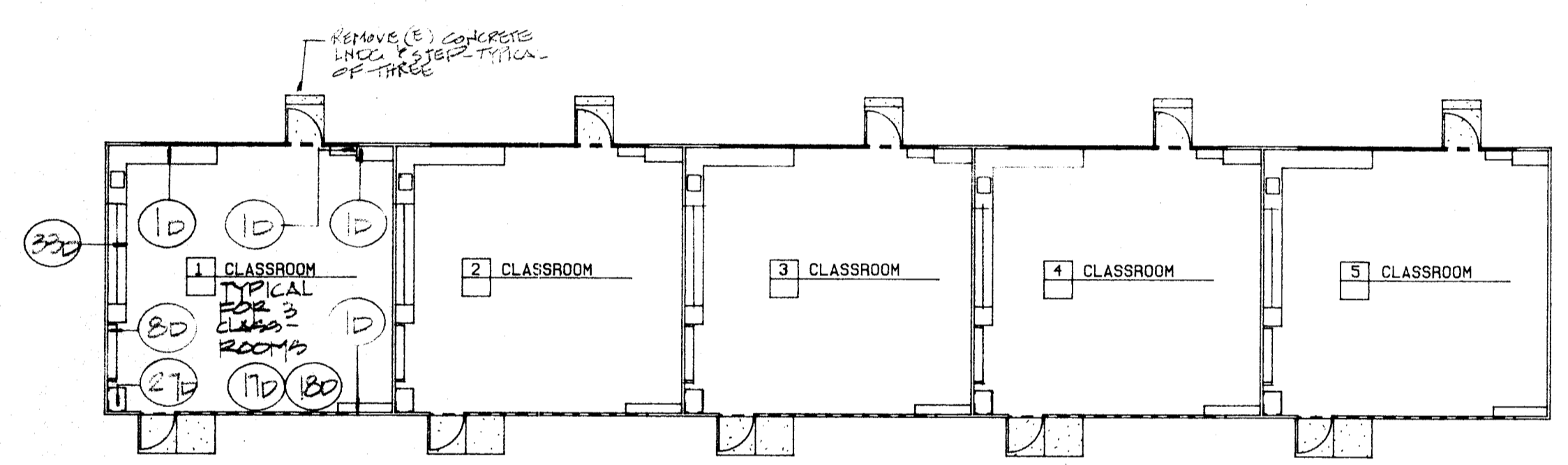
FLOOR PLAN - UNIT R5 (DEMOLITION/EXISTING PLAN) 1/16" = 1'-0"
