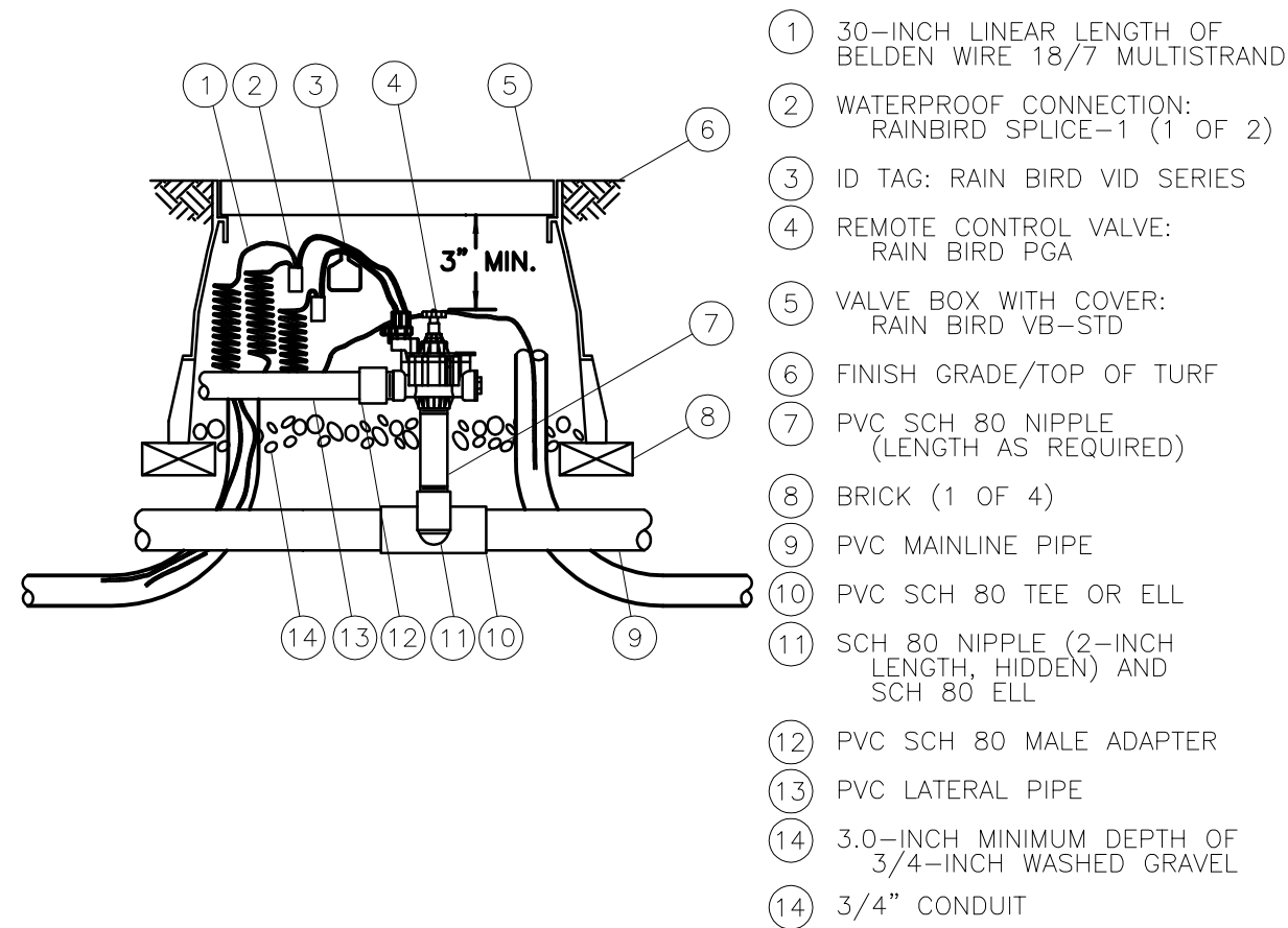
D ELECTRIC REMOTE CONTROL VALVE 1-23-04 REVISED NTS PGA-BI-PRSD-2000
