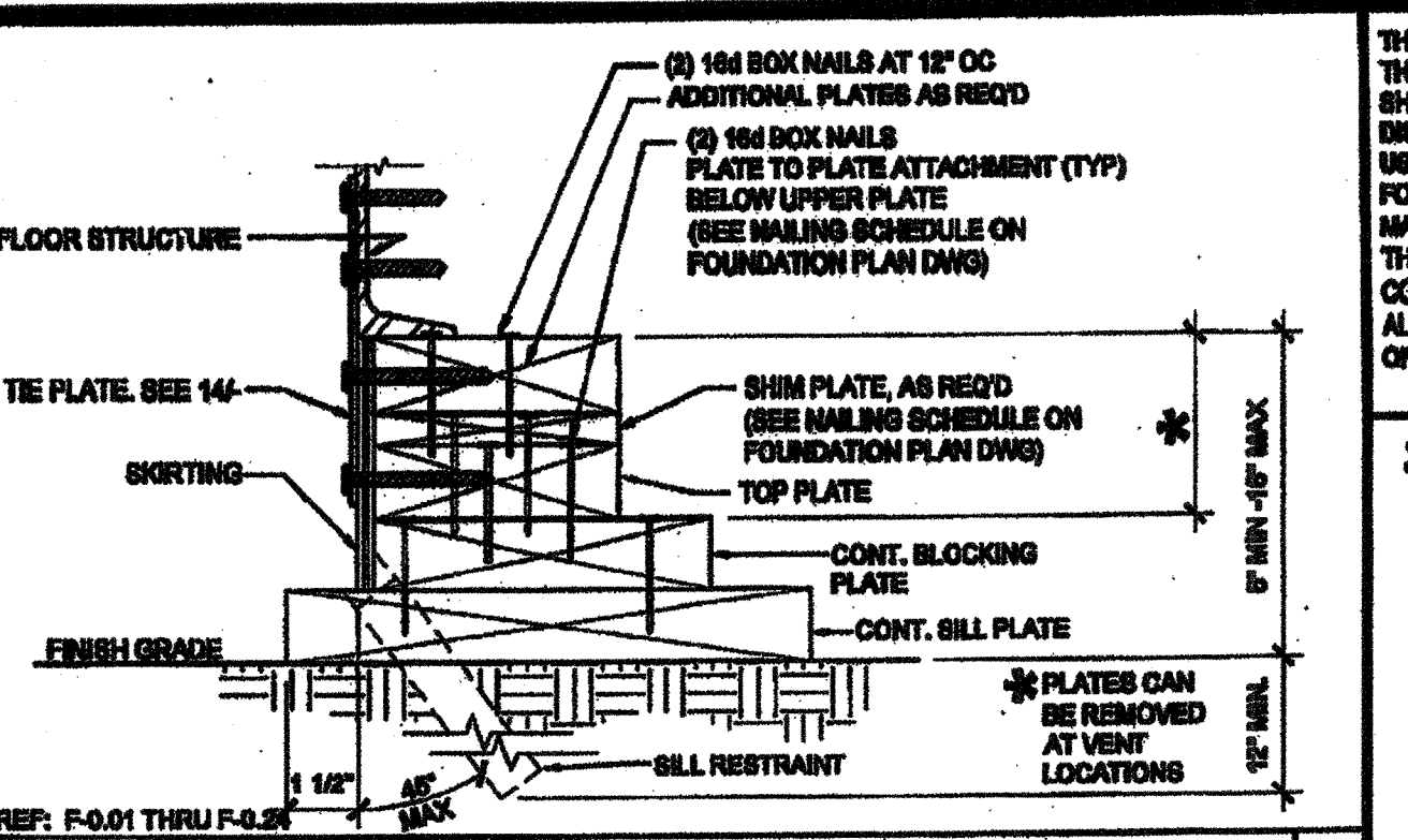
6 FOUNDATION AT END WALL SCALE: 3/4"=1'-0"
