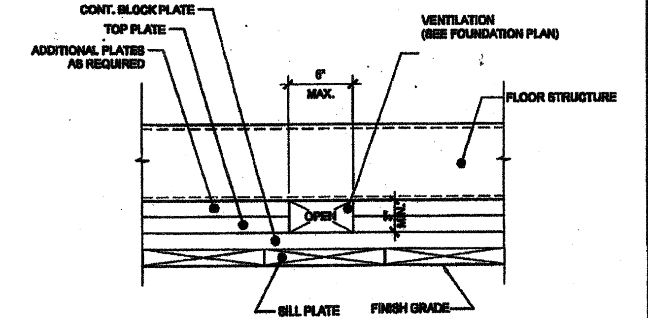
12 VENT ELEV. AT MODLINE & SEP FOR 150 PSF SCALE: 3/4"=1'-0"
