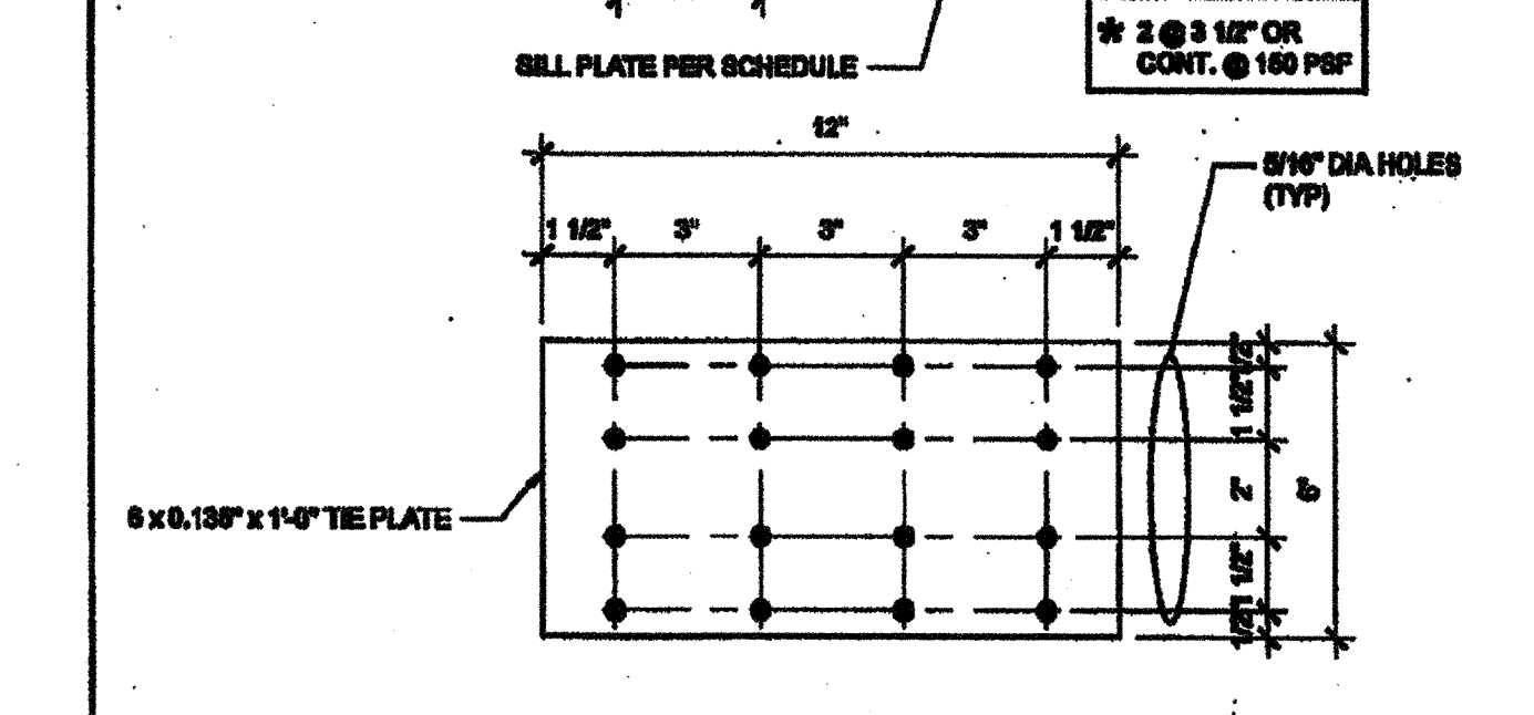
18 TIE PLATE SCALE: 3/4"=1'-0"
