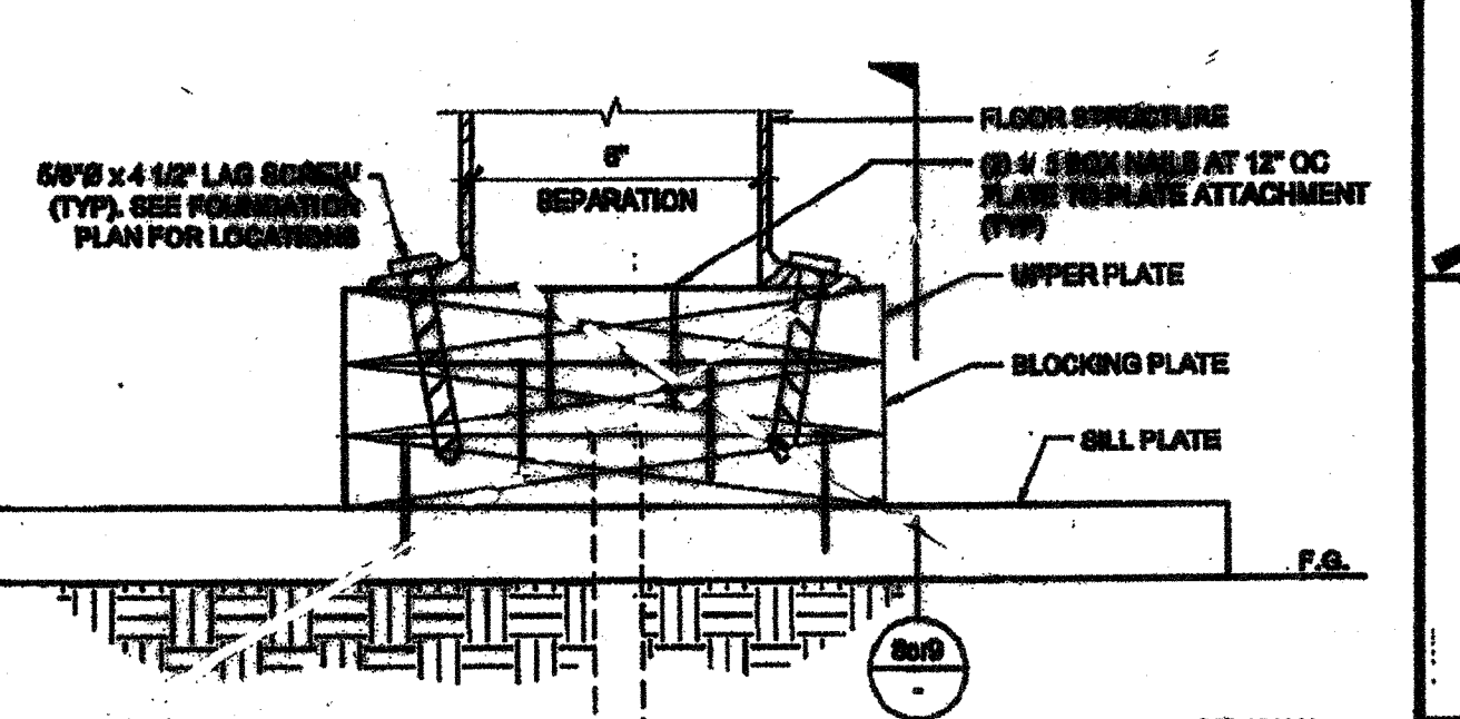
7 FOUNDATION AT ADJACENT BUILDING SCALE: 3/4"=1'-0"
