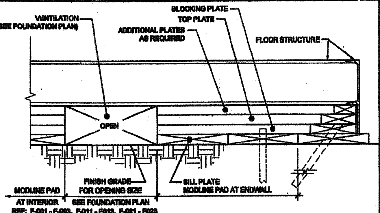
12 FOUNDATION AT MODLINE & SEPARATION SCALE: 1 1/2"=1'-0"
