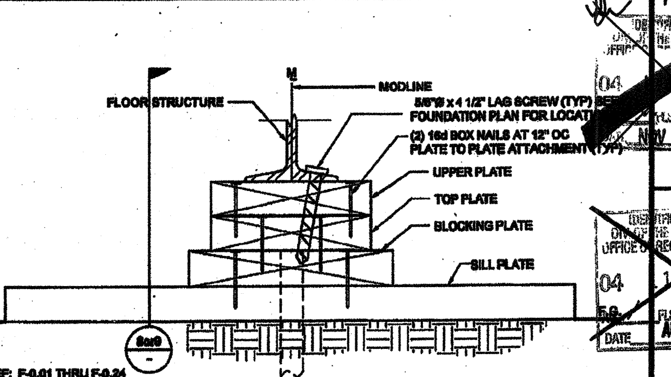
7 FOUNDATION AT MODLINE SCALE: 3/4"=1'-0"
