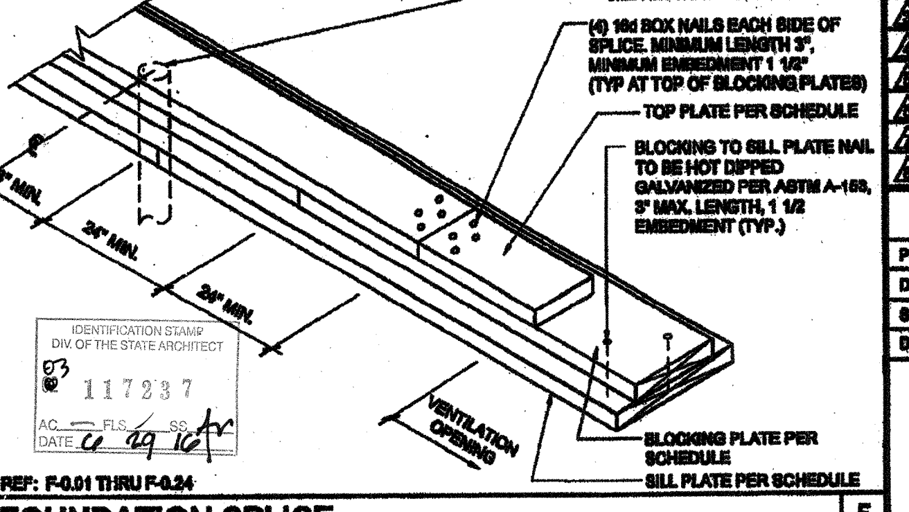
7 FOUNDATION SPLICE SCALE: NTS
