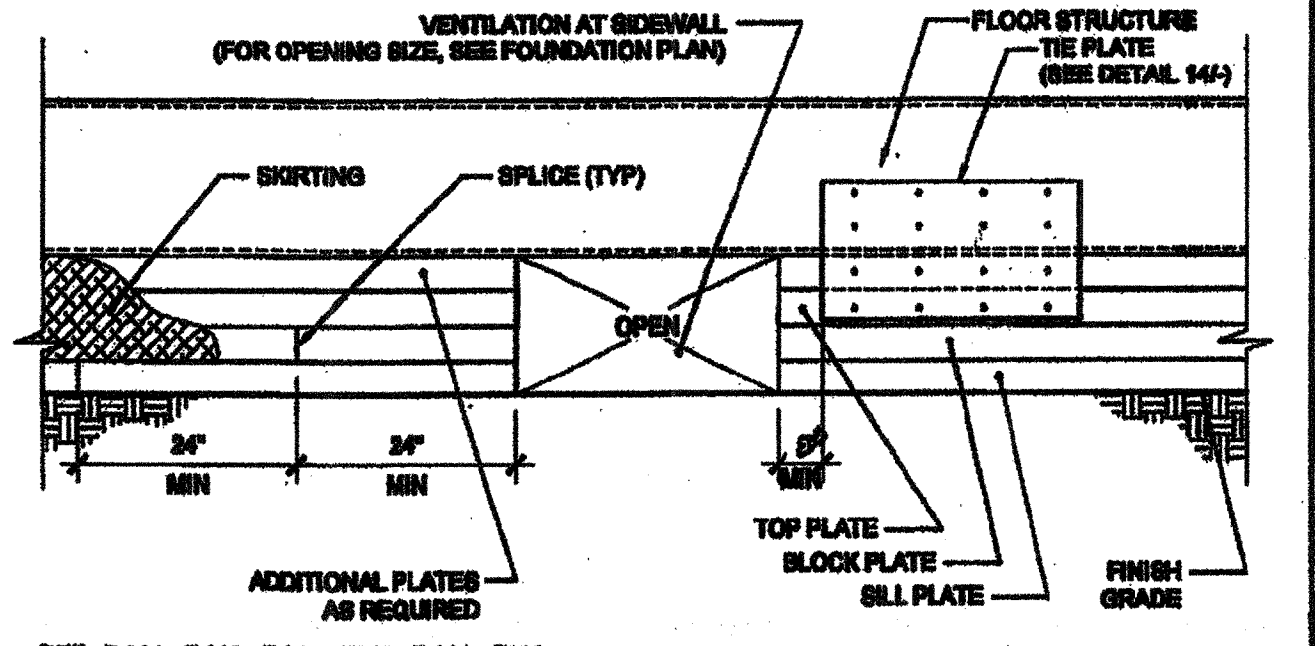
12 FOUNDATION ASSEMBLY SIDEWALL ELEVATION SCALE: 1 1/2"=1'-0"
