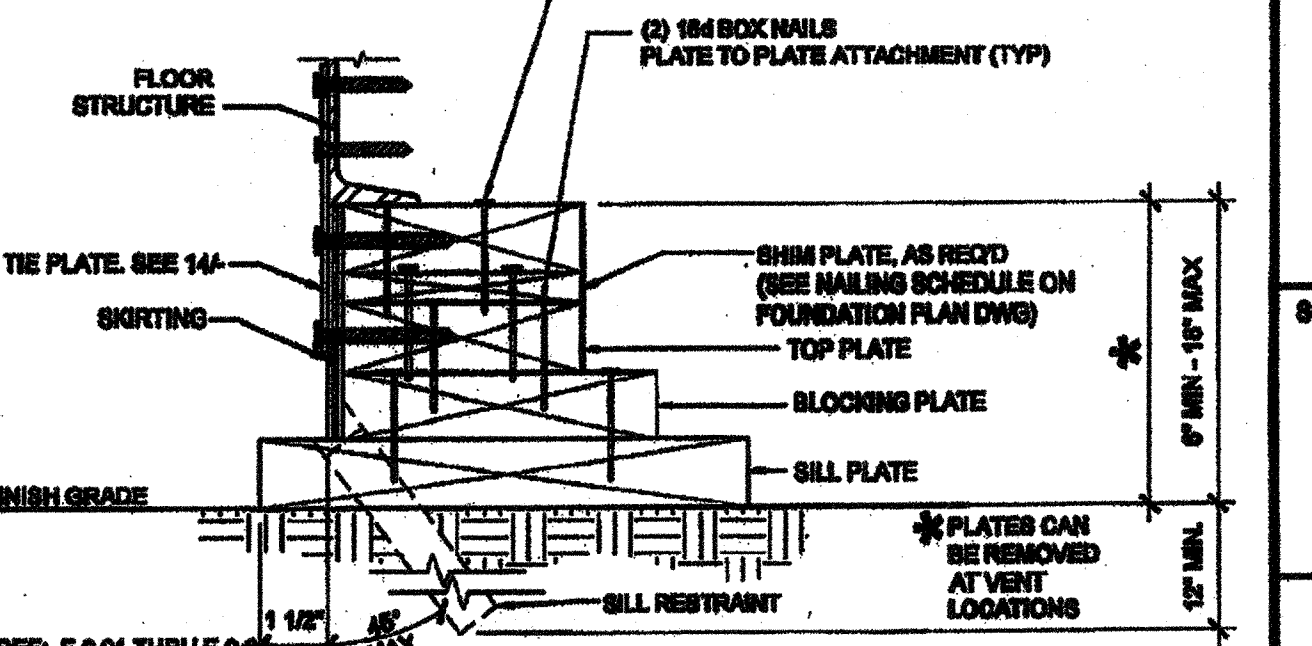
7 FOUNDATION AT SIDE WALL SCALE: 3/4"=1'-0"
