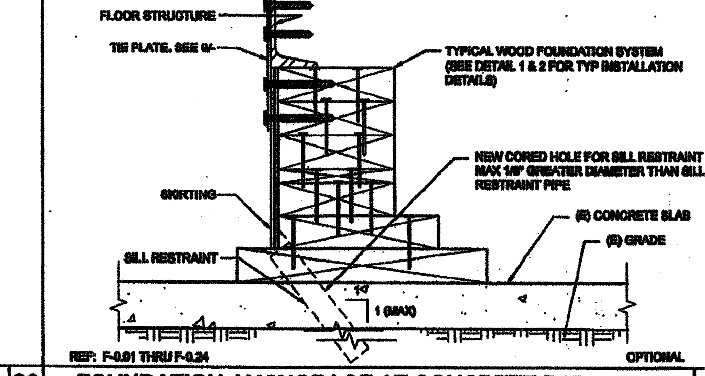
20 FOUNDATION ANCHORAGE AT CONCRETE PAD SCALE: 3/4"=1'-0"
