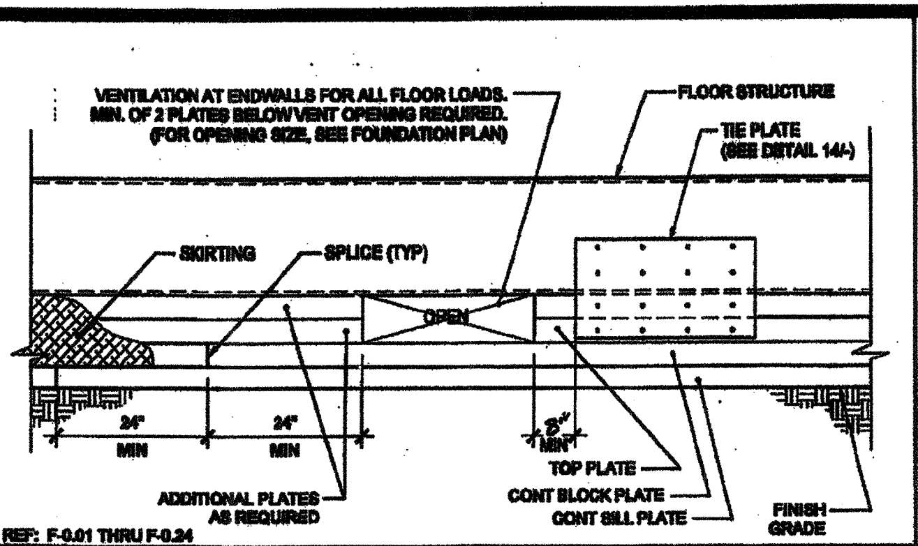
11 FOUNDATION ASSEMBLY END WALL ELEVATION SCALE: 1 1/2"=1'-0"
