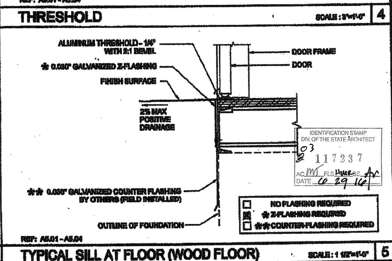
REF: A5.01 - A5.04 TYPICAL SILL AT FLOOR (WOOD FLOOR) SCALE: 1/12"=1'-0" 5
