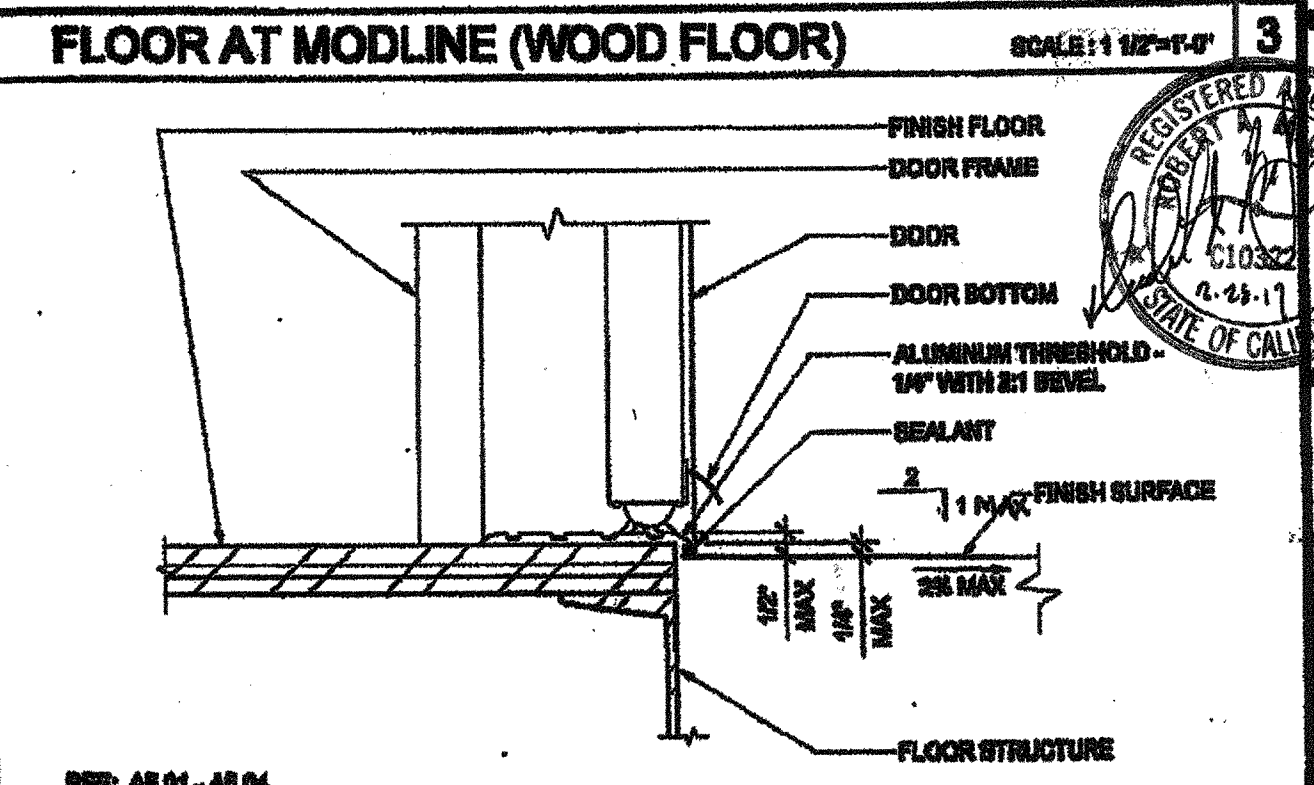
REF: A5.01 - A5.04 THRESHOLD SCALE: 3/8"=1'-0" 4
