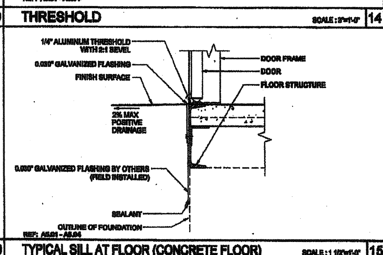
REF: A5.01 - A5.04 TYPICAL SILL AT FLOOR (CONCRETE FLOOR) SCALE: 1/12"=1'-0" 15
