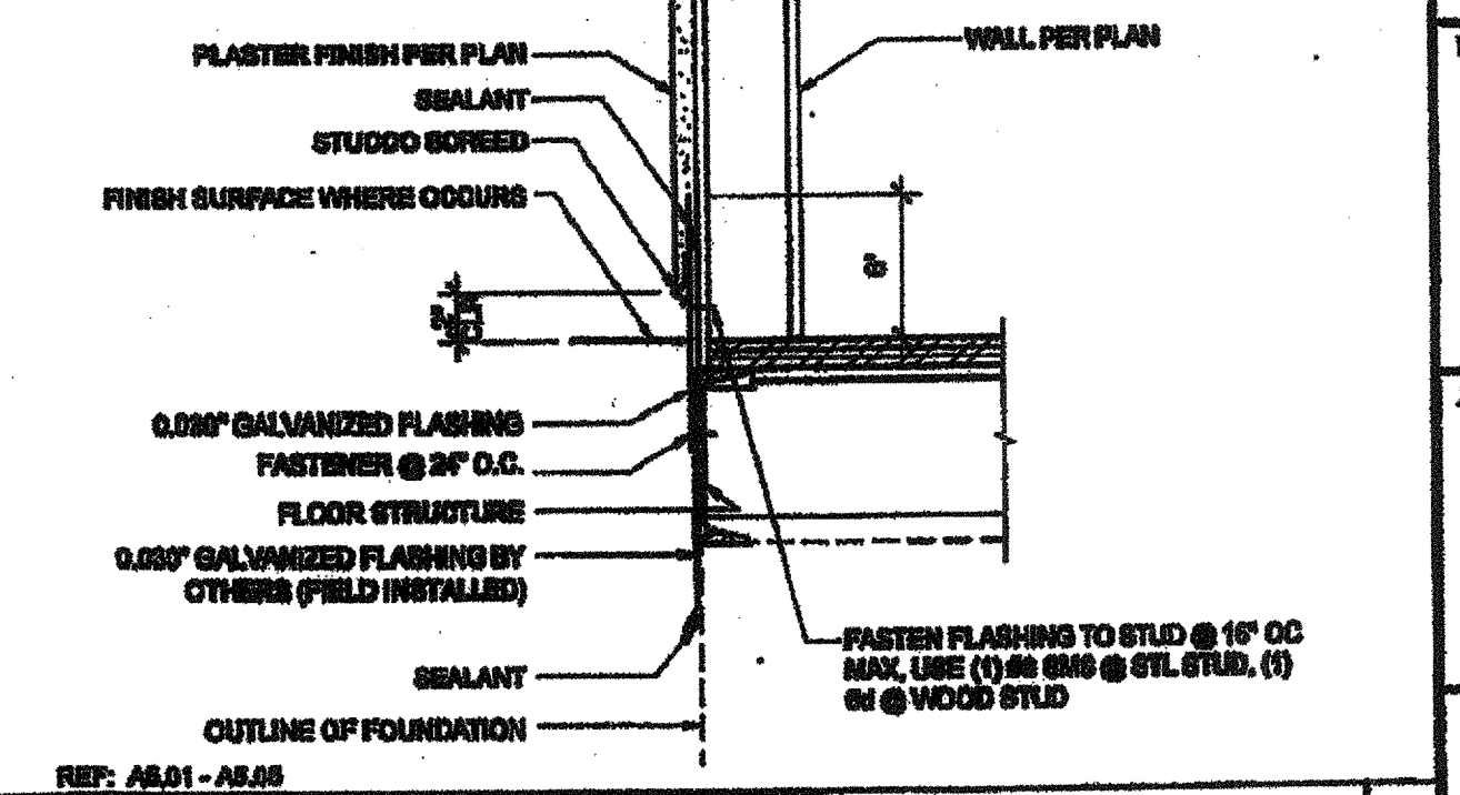
REF: A5.01 - A5.05 SKIRT FLASHING (WOOD FLOOR) SCALE: 1/12"=1'-0" 2
