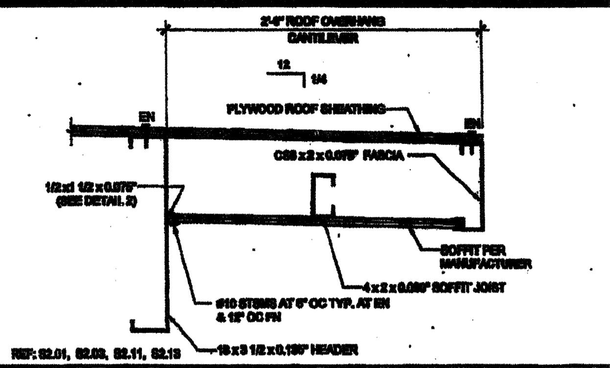
REAR OVERHANG SECTION SCALE: 1 1/2" = 1'-0" 11
