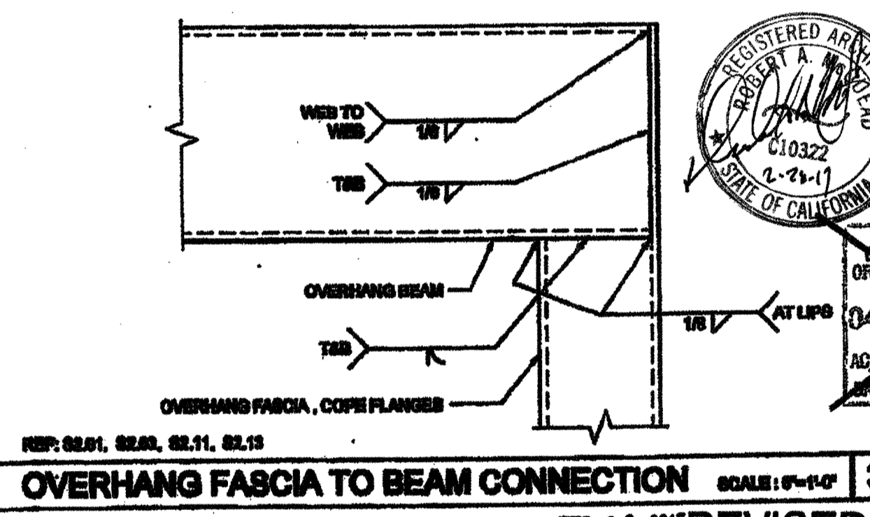
OVERHANG FASCIA TO BEAM CONNECTION SCALE: 3/4" = 1'-0" 3
