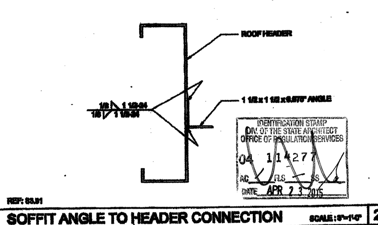
SOFFIT ANGLE TO HEADER CONNECTION SCALE: 3/4" = 1'-0" 2
