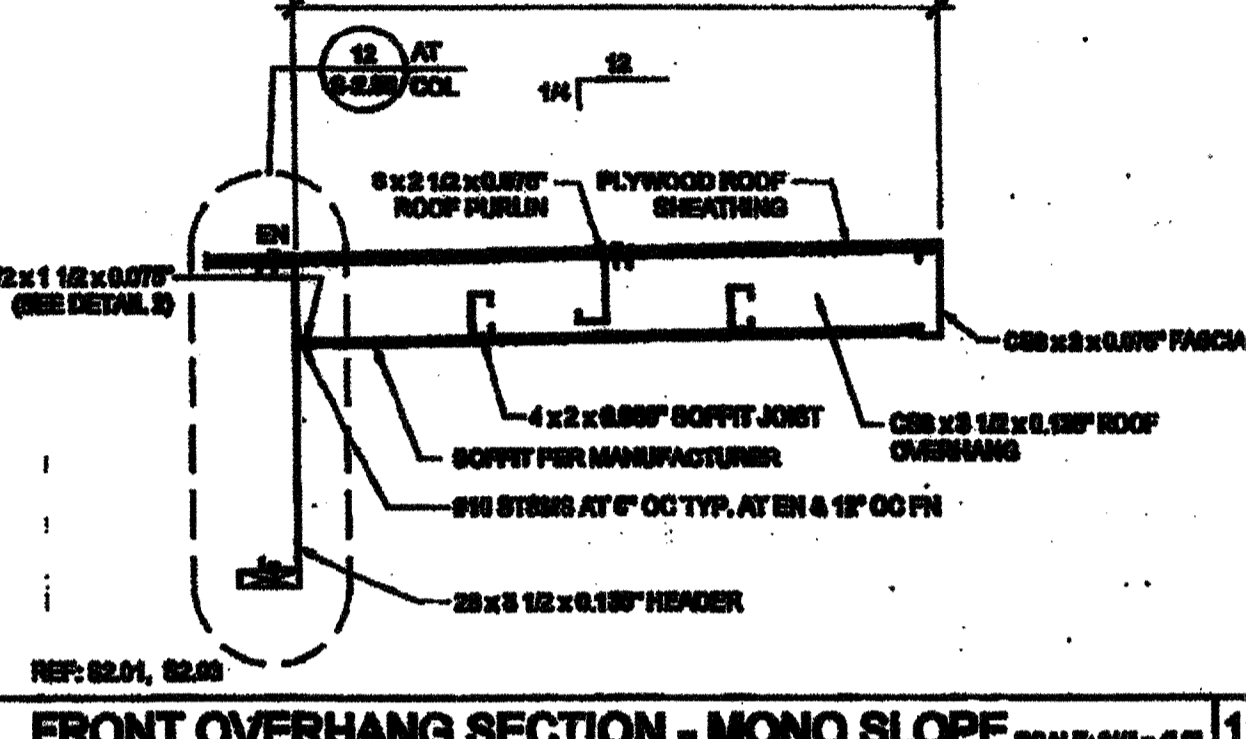
FRONT OVERHANG SECTION - MONO SLOPE SCALE: 3/4" = 1'-0" 12
