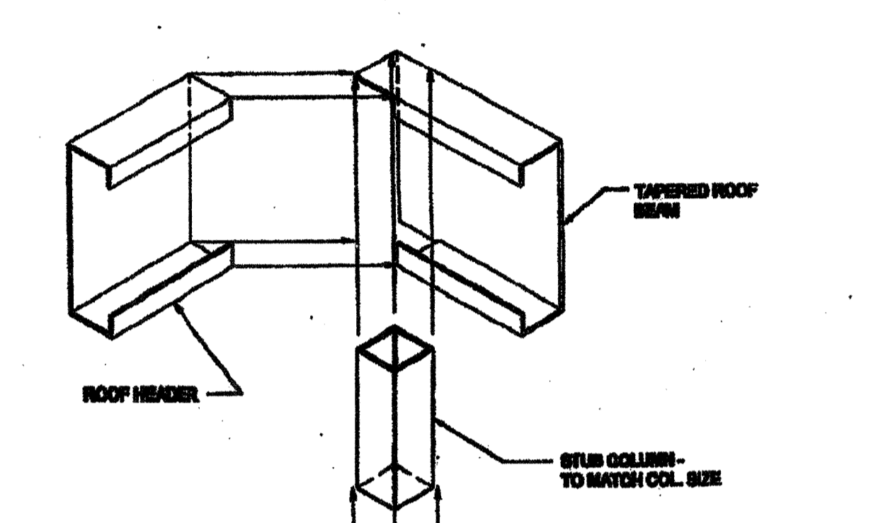
COLUMN CONNECTION AT ROOF SCALE: 1/8" = 1'-0" 8
