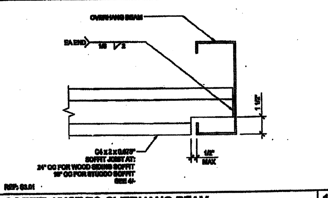
SOFFIT JOIST TO OVERHANG BEAM SCALE: 3/4" = 1'-0" 1
