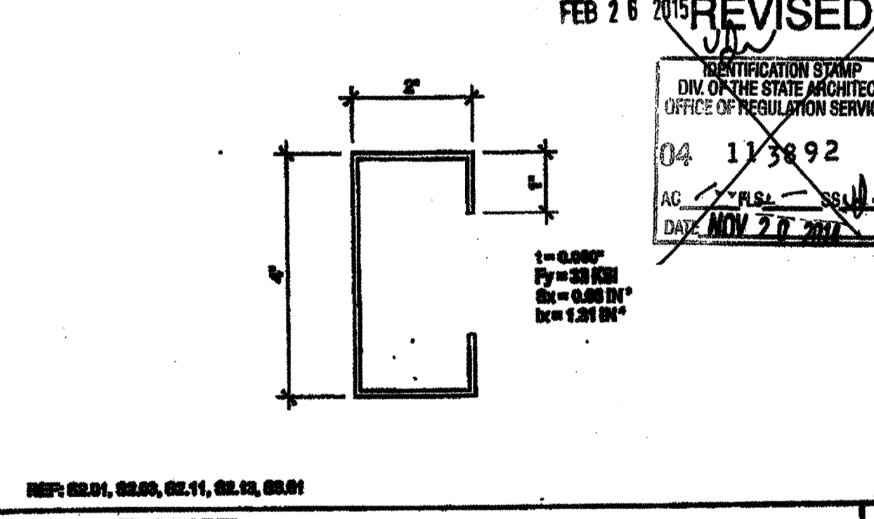
OVERHANG SUPPORT TO ROOF HDR @ STIFFENER SCALE: 3/4" = 1'-0" 10
