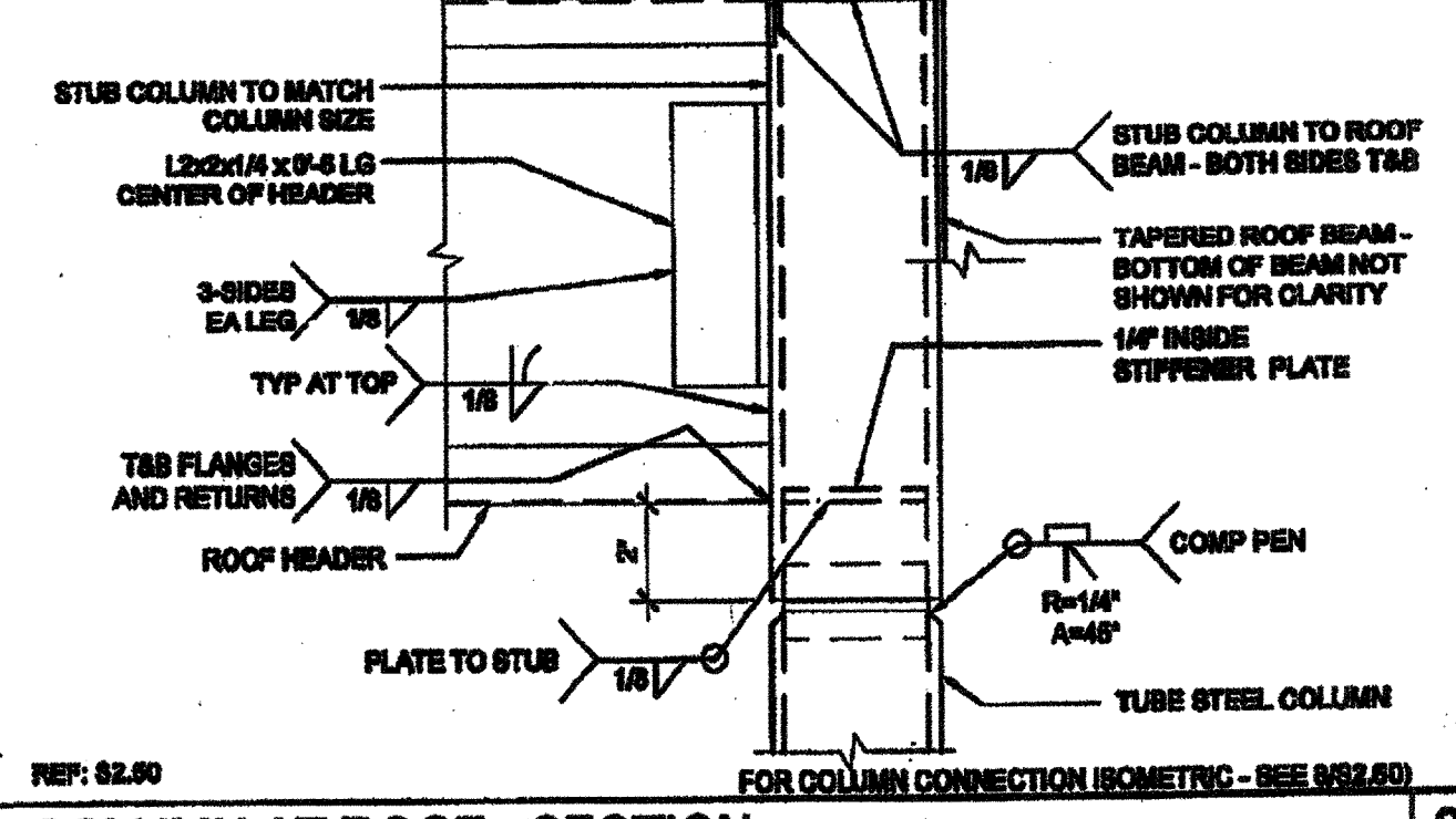
REF: S2.01 COLUMN AT ROOF - SECTION SCALE: 3"=1'-0" 2
