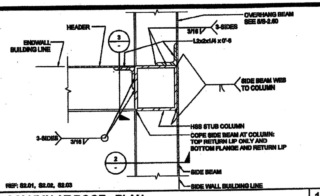
REF: S2.01, S2.02, S2.03 COLUMN AT ROOF - PLAN SCALE: 3"=1'-0" 1
