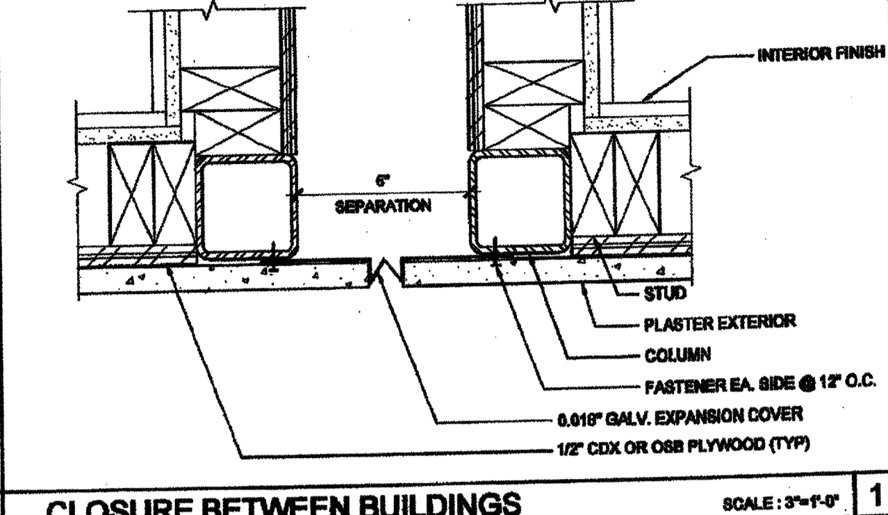
CLOSURE BETWEEN BUILDINGS SCALE: 3/4"=1'-0" 1
