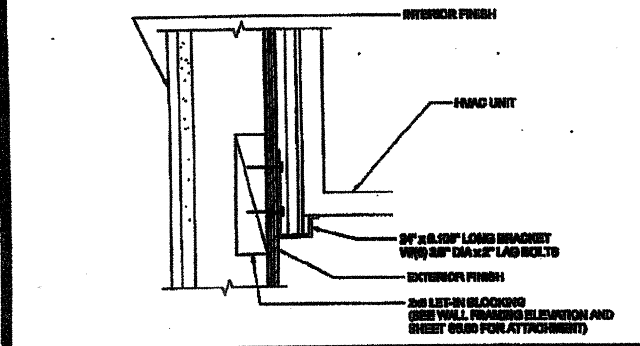
HVAC UNIT AT BOTTOM SCALE: 1/2"=1'-0" 17
