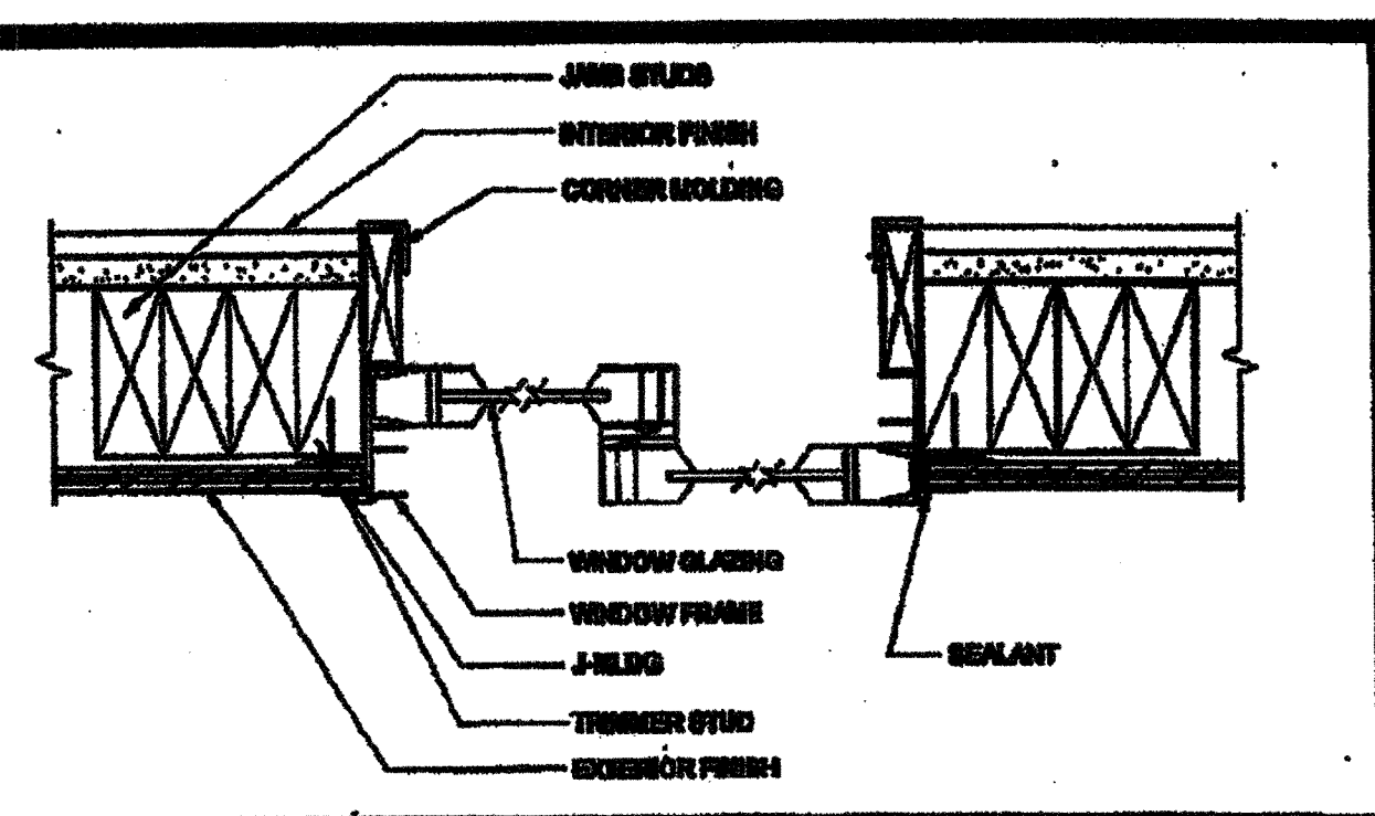
WINDOW SECTION AT JAMBS SCALE: 1/2"=1'-0" 11
