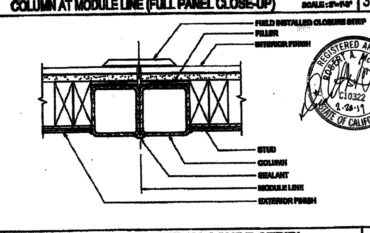
COLUMN AT MODULE LINE (CLOSURE STRIP) SCALE: 1/2"=1'-0" 4
