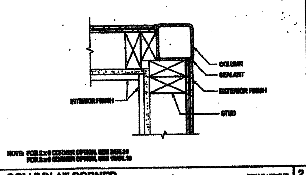
COLUMN AT CORNER SCALE: 1/2"=1'-0" 2
