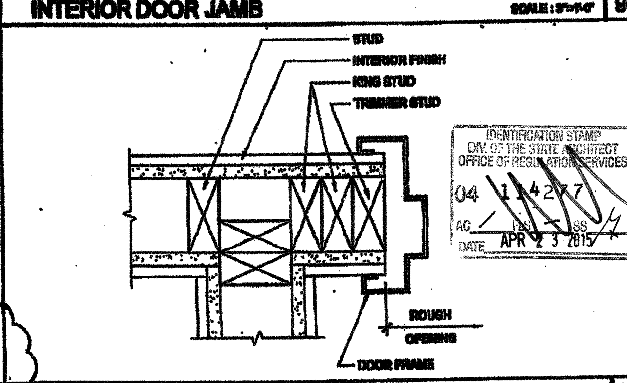
INTERIOR DOOR JAMBS SCALE: 1/2"=1'-0" 10
