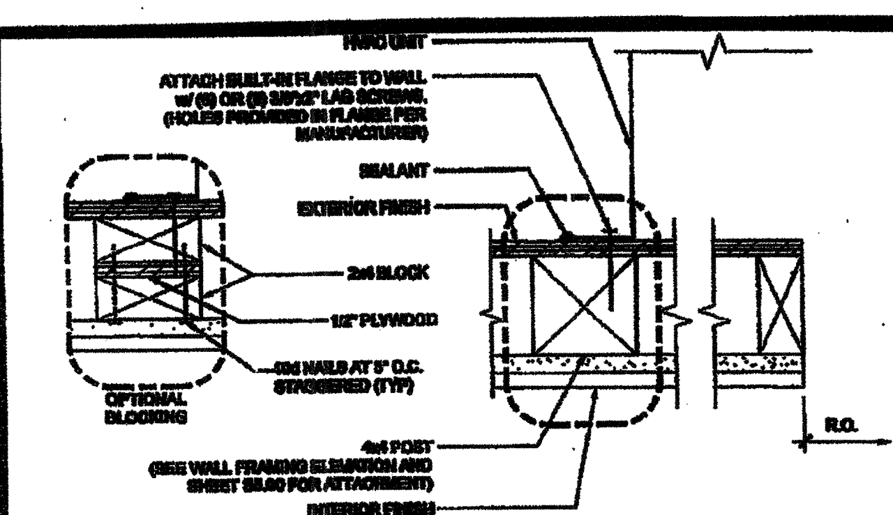
HVAC MOUNT AT JAMBS SCALE: 1/2"=1'-0" 16
