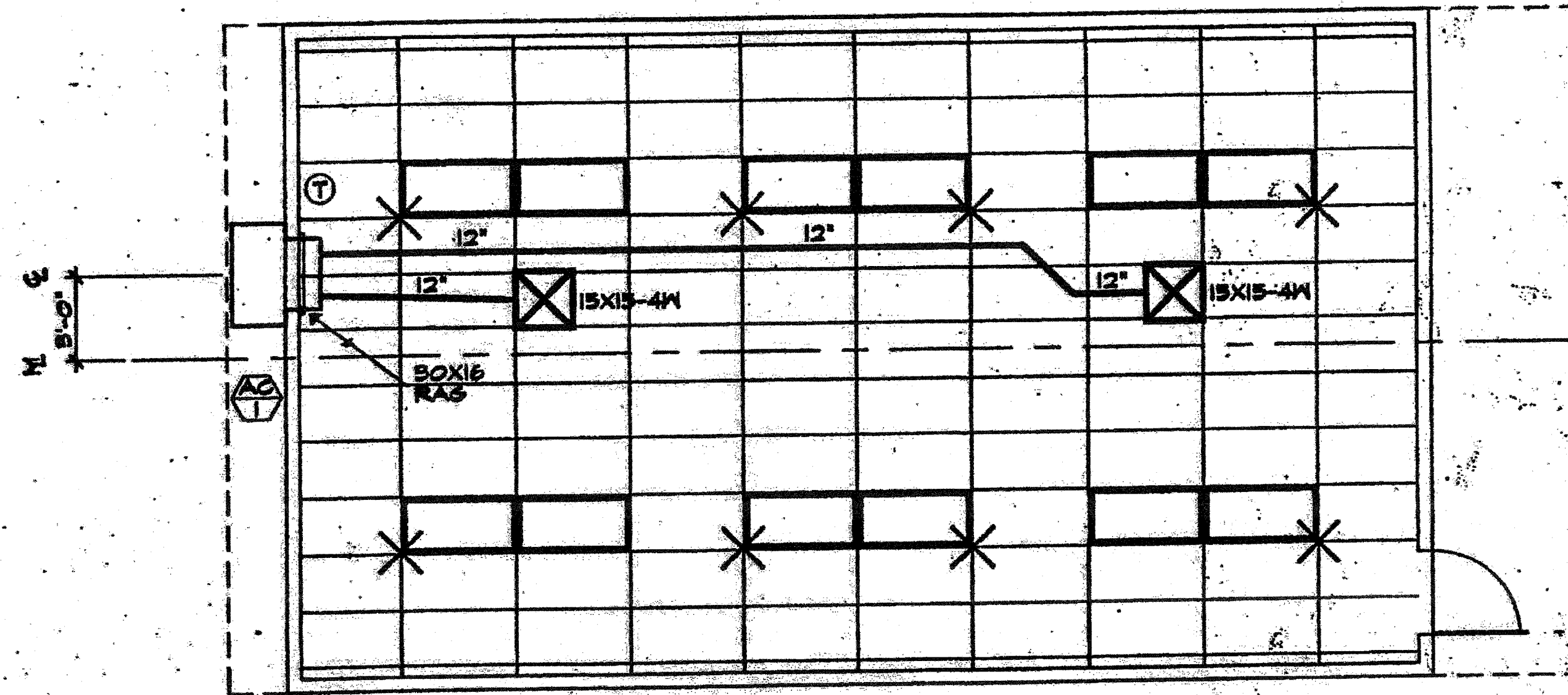
AIR CONDITIONING PLAN VIEW 24'X40' BUILDING SCALE 1/4"=1'-0"
