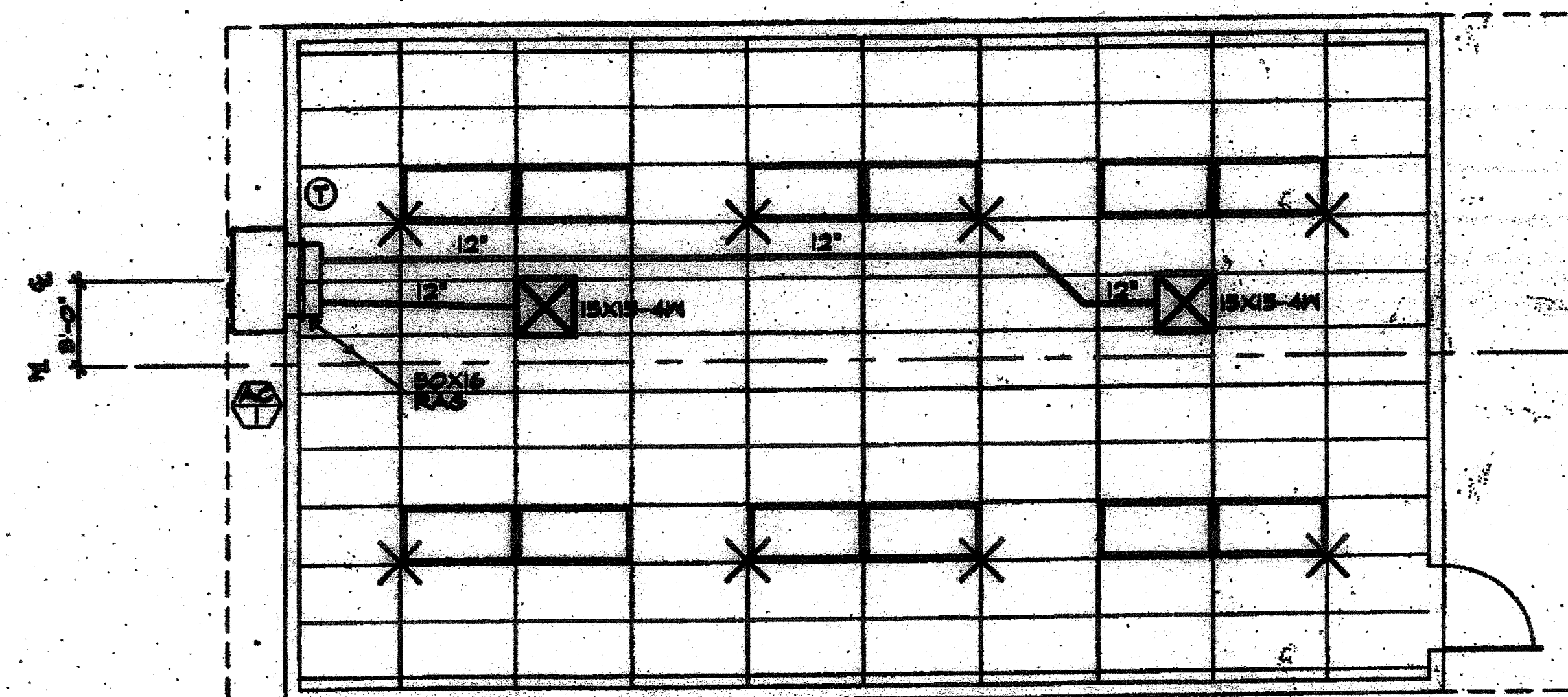
AIR CONDITIONING PLAN VIEW 24'X40' BUILDING
