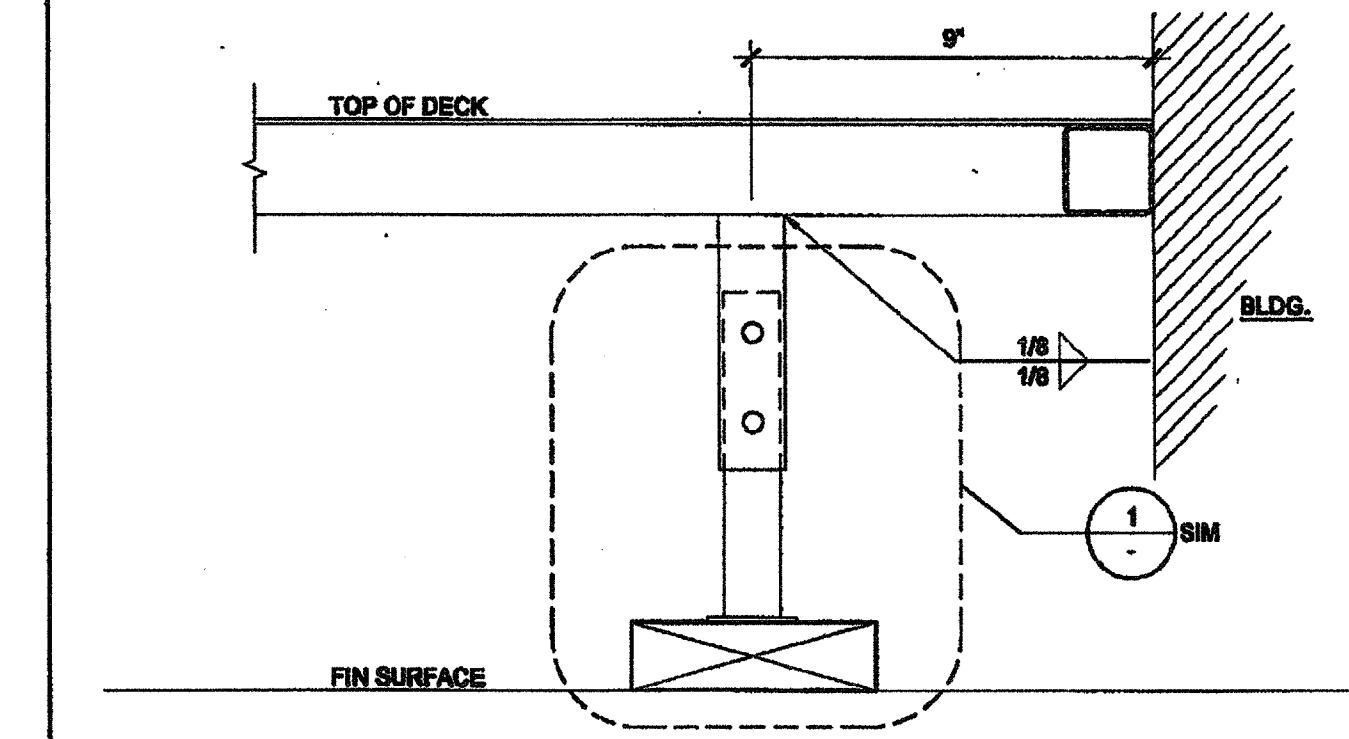
INTERIOR LANDING LEG SECTION SCALE: 3\"/>
