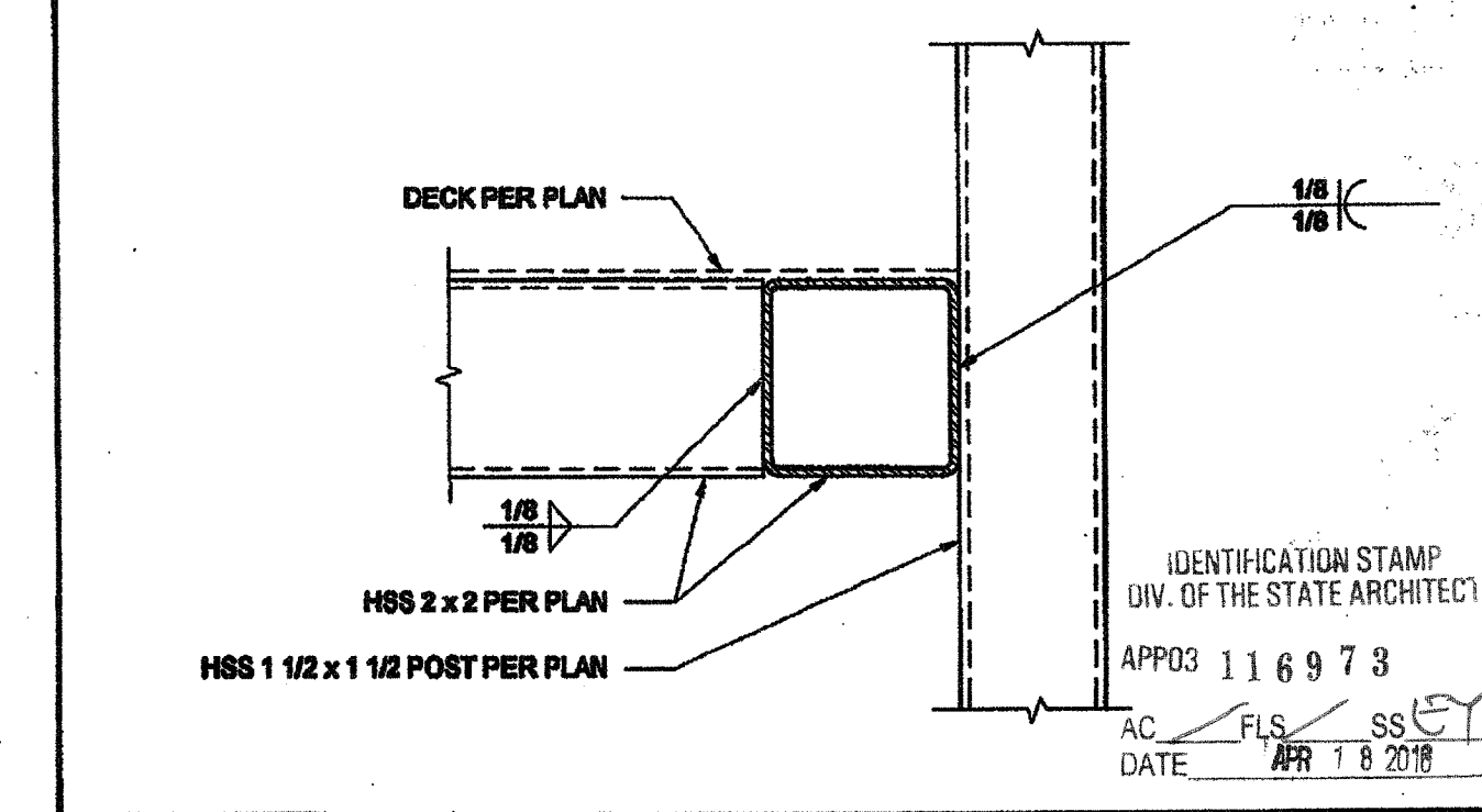
GUARDRAIL POST ATTACHMENT SCALE: 6\"/>
