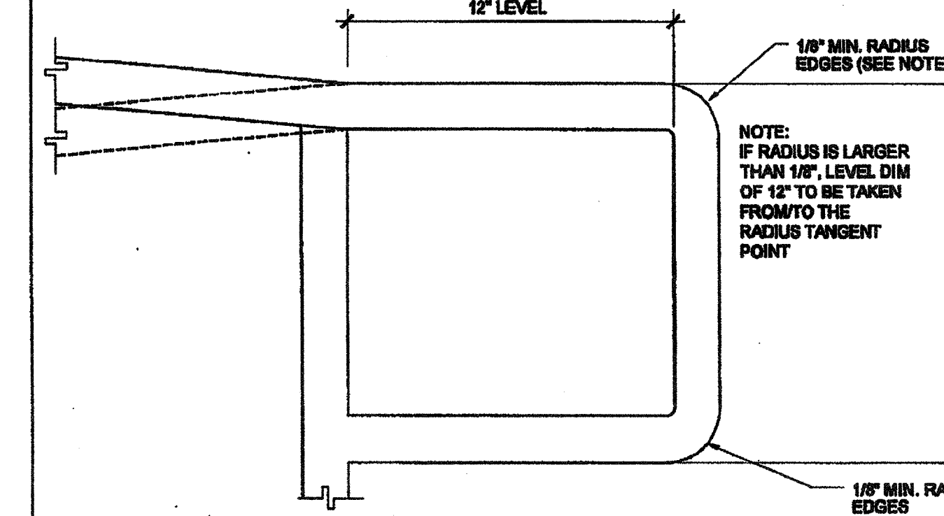
EXTEND HANDRAIL @ TOP OR BOTT. ENDS SCALE: 3\"/>
