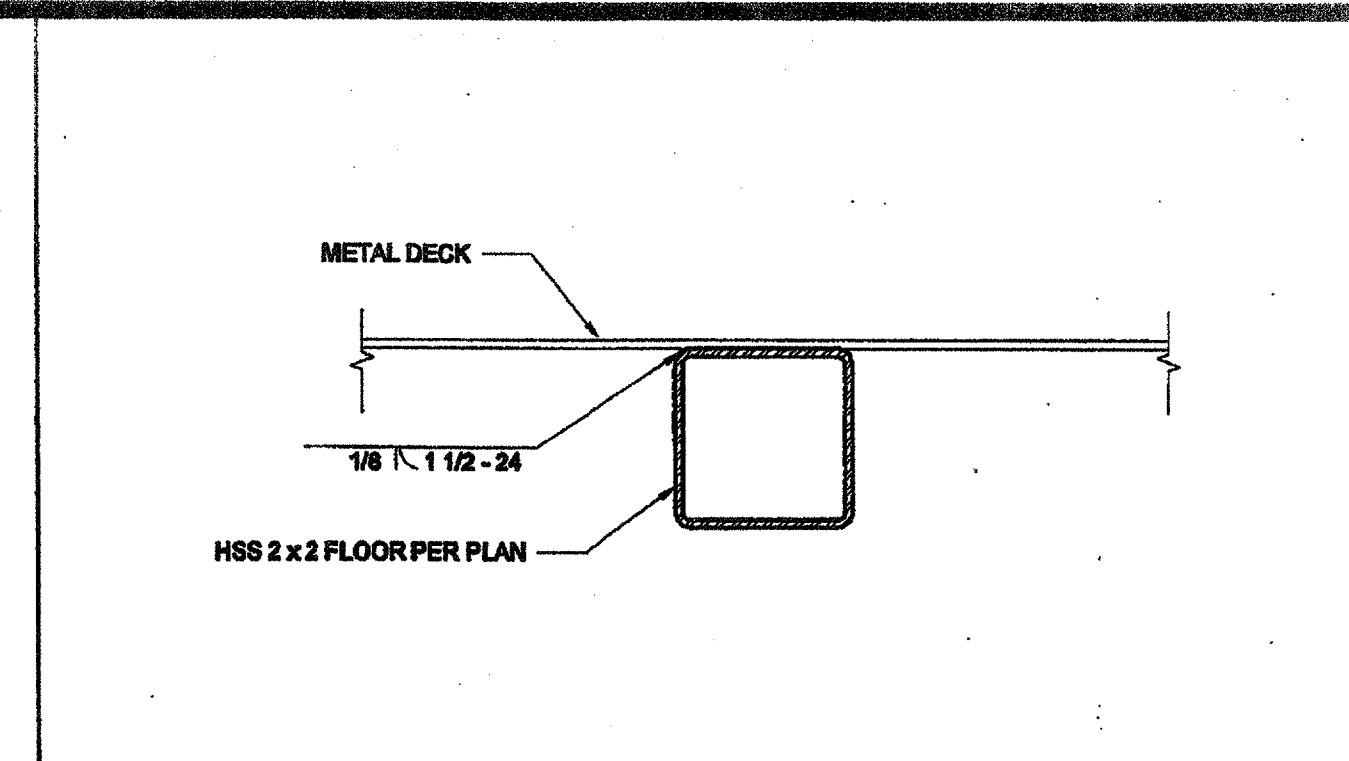
DECK TO FRAME SCALE: 6\"/>
