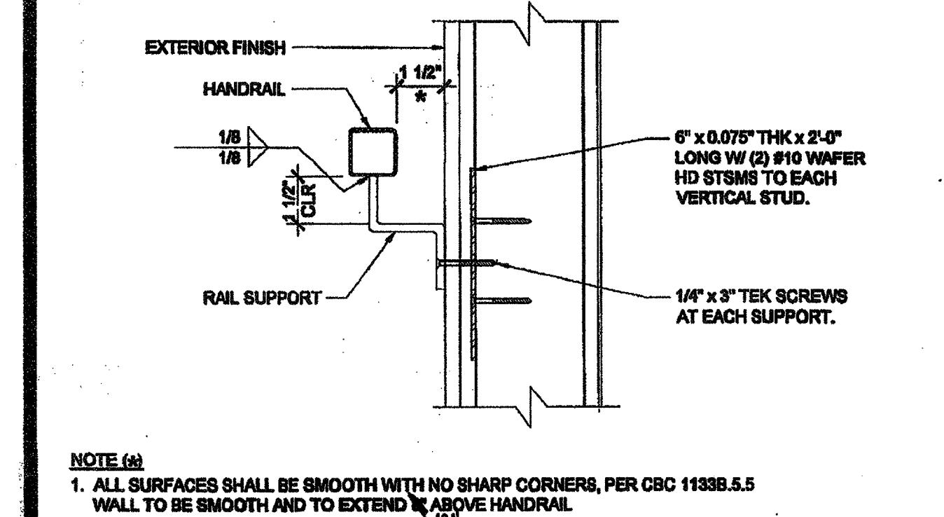
HANDRAIL CONNECTION AT SHEETMETAL BLKG SCALE: 3\"/>
