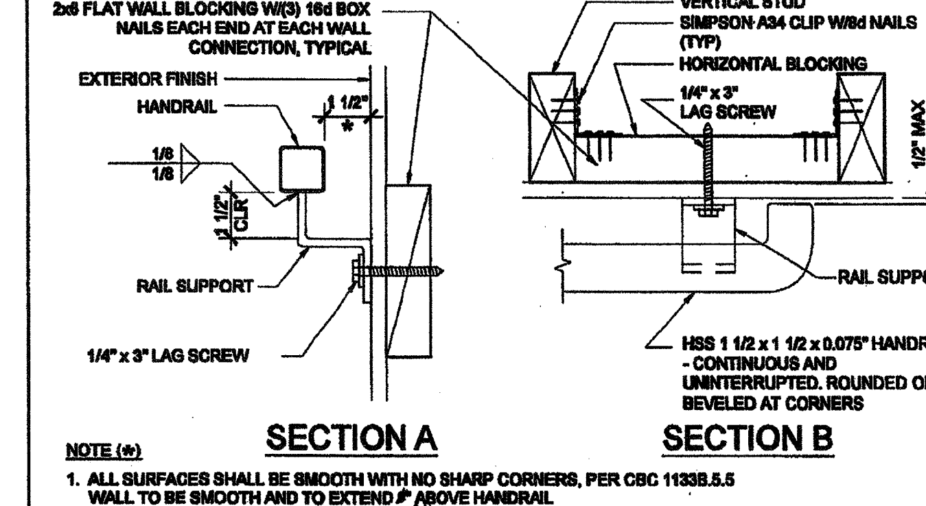
HANDRAIL CONNECTION AT WOOD BLOCKING SCALE: 3\"/>
