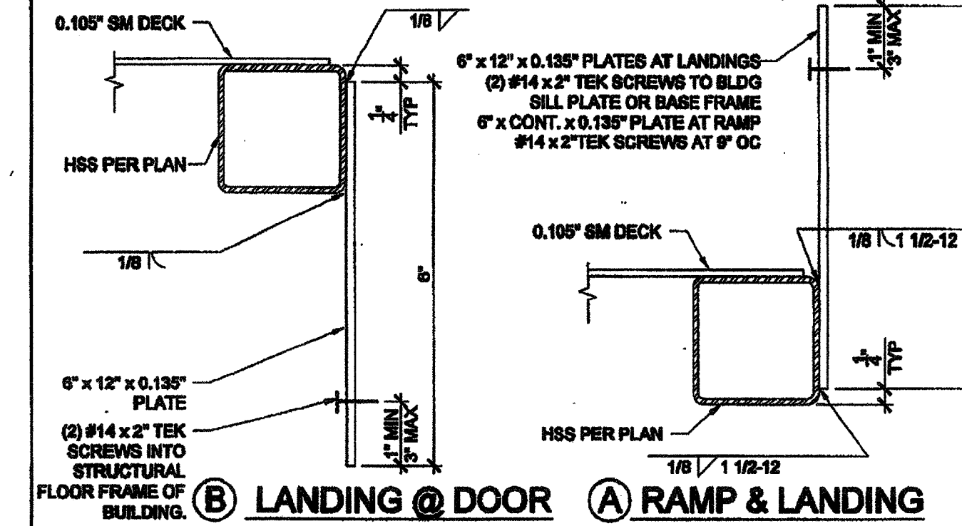
SECTION AT PLATE SCALE: 6\"/>
