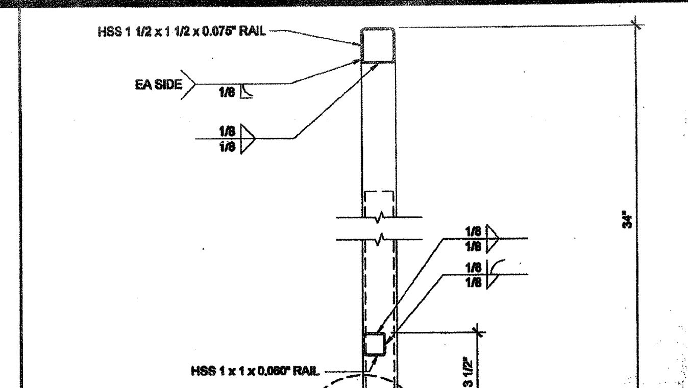
ADJUSTABLE LEG SCALE: 3\"/>
