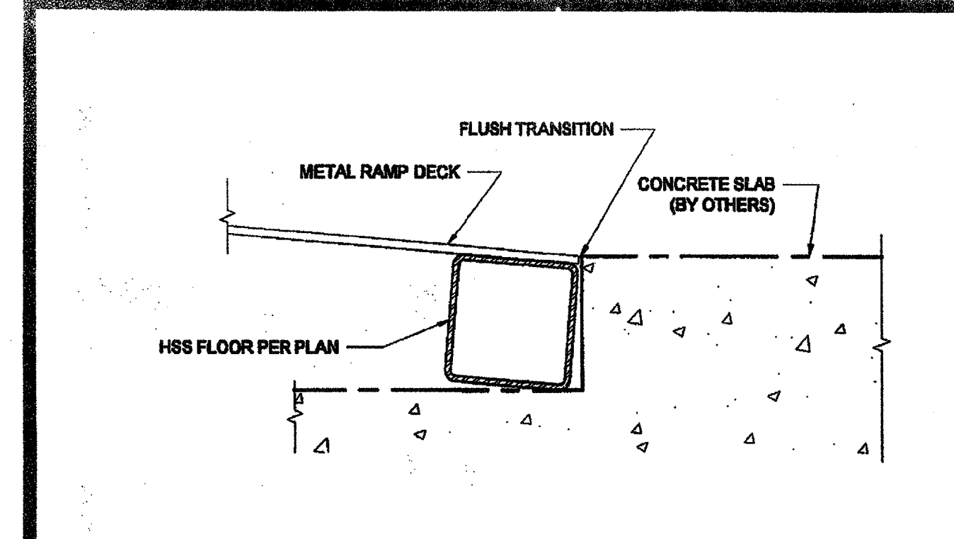
FLUSH TRANSITION AT BOTTOM OF RAMP SCALE: 6\"/>
