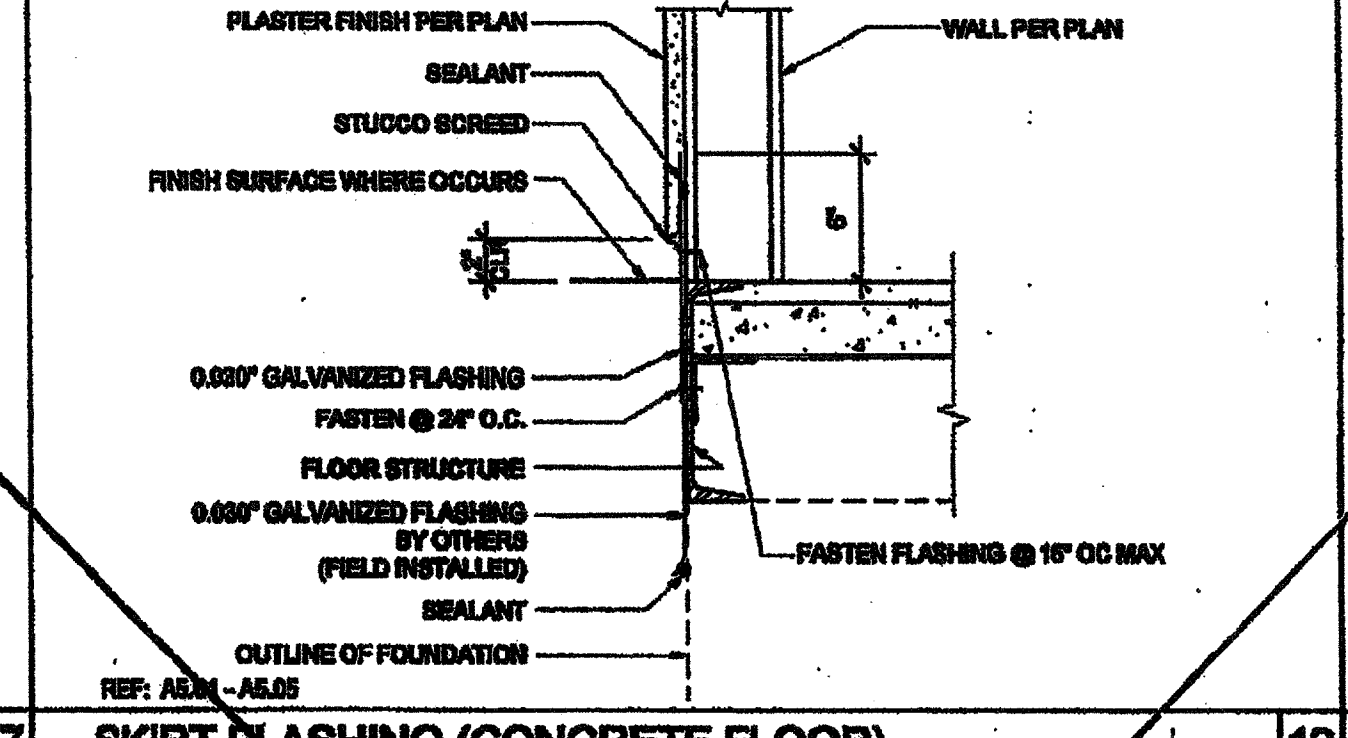
REF: AS.01 - AS.05 SKIRT FLASHING (WOOD FLOOR) SCALE: 1/12"=1'-0" 7
