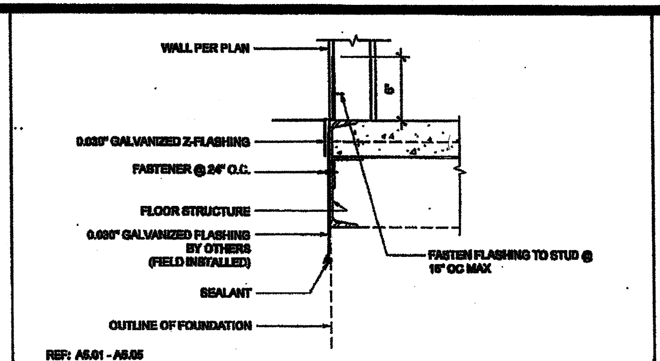
REF: AS.01 - AS.05 SKIRT FLASHING (CONCRETE FLOOR) SCALE: 1/12"=1'-0" 11
