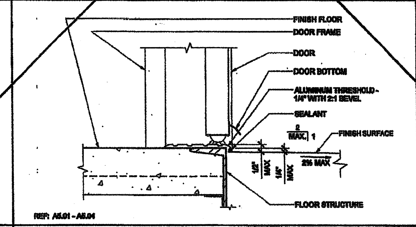
REF: AS.01 - AS.04 THRESHOLD SCALE: 3/8"=1'-0" 14
