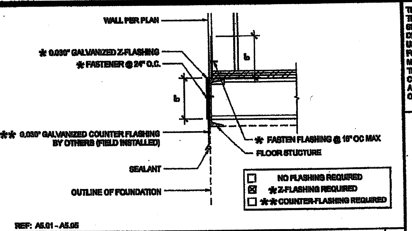
REF: AS.01 - AS.05 SKIRT FLASHING (WOOD FLOOR) SCALE: 1/12"=1'-0" 1
