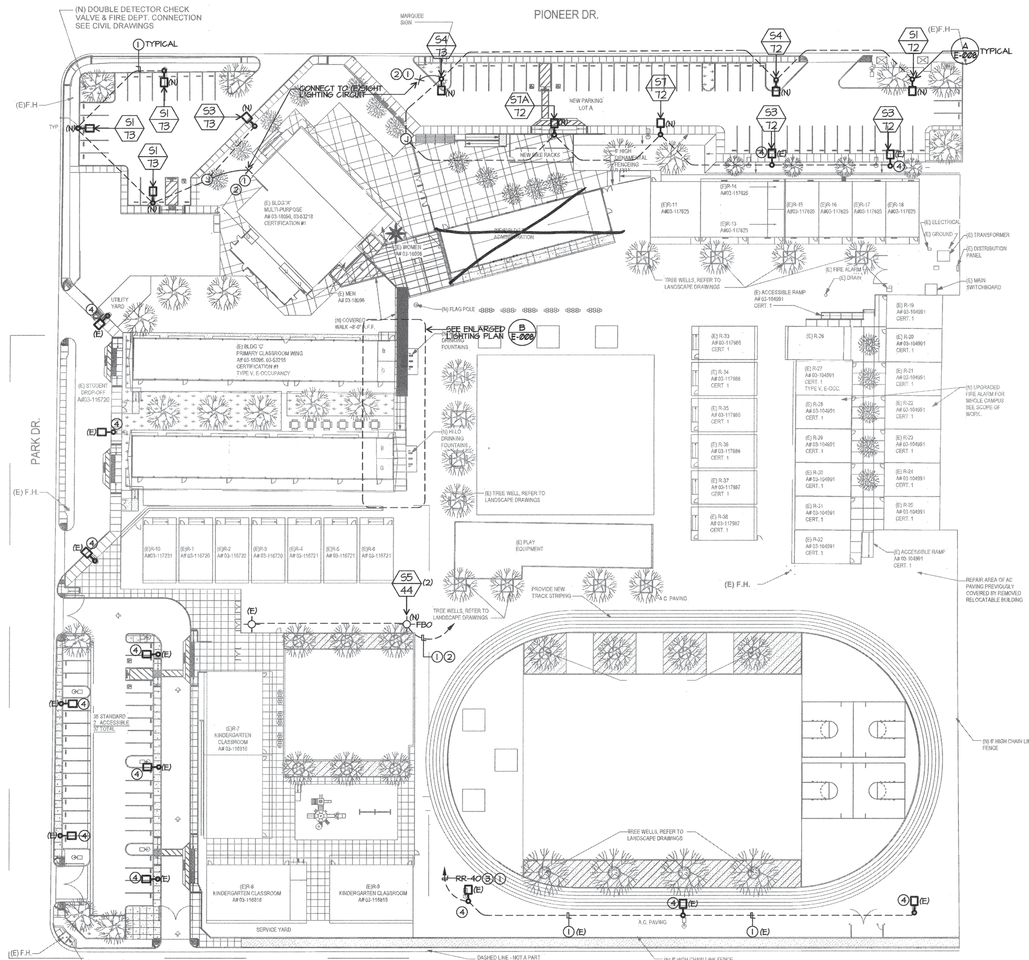
SITE LIGHTING PLAN SCALE: 1"=40'-0"
