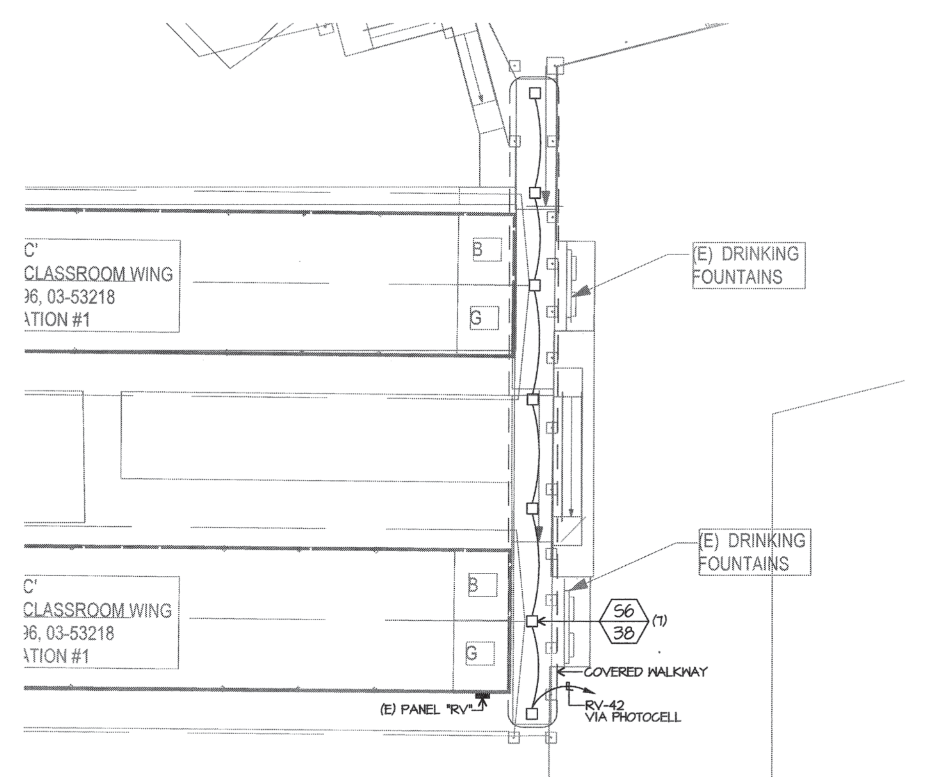
ENLARGED LIGHTING PLAN SCALE: 1"=20'-0"
