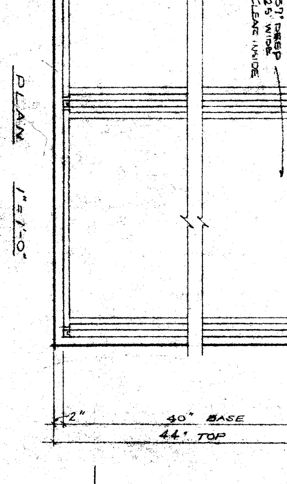
13 PLAN OF WORK TABLE
