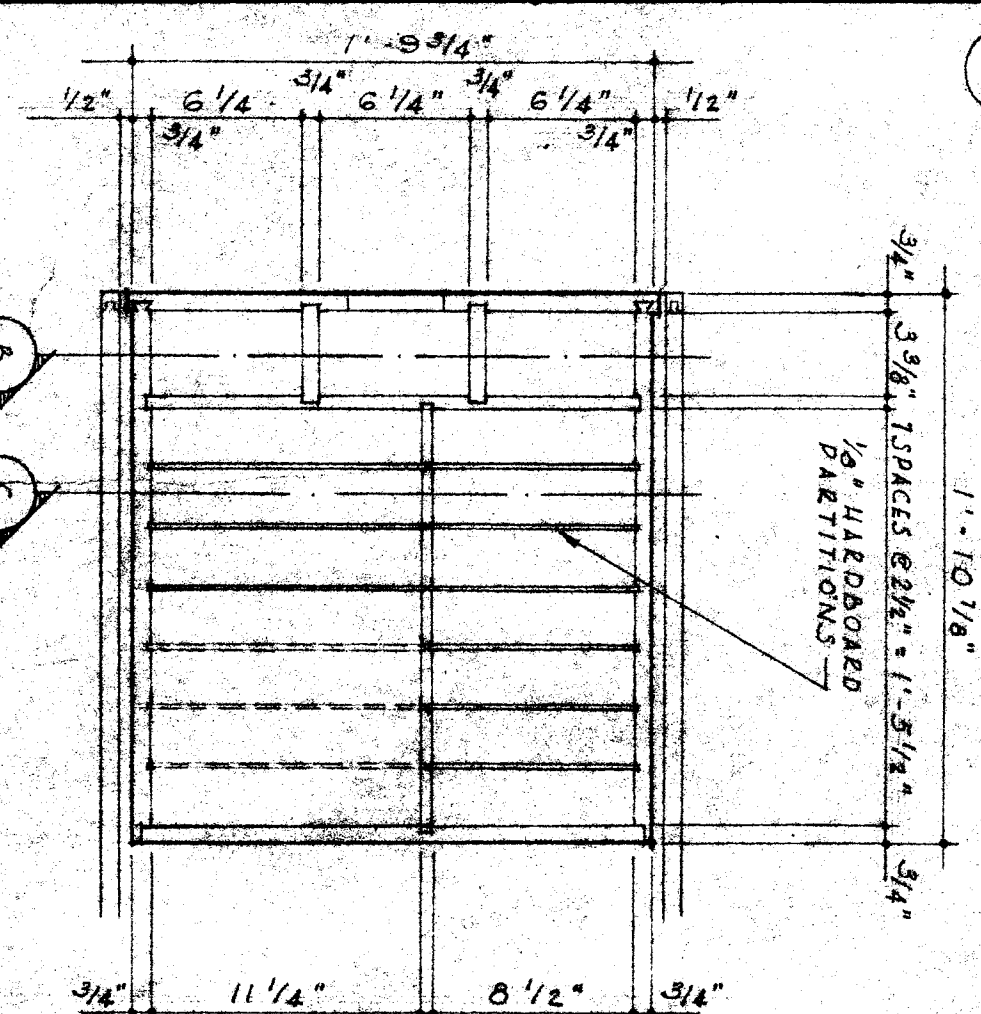
5 PLAN OF CARD FILE DRAWER - 1/2 x 1'-0"
