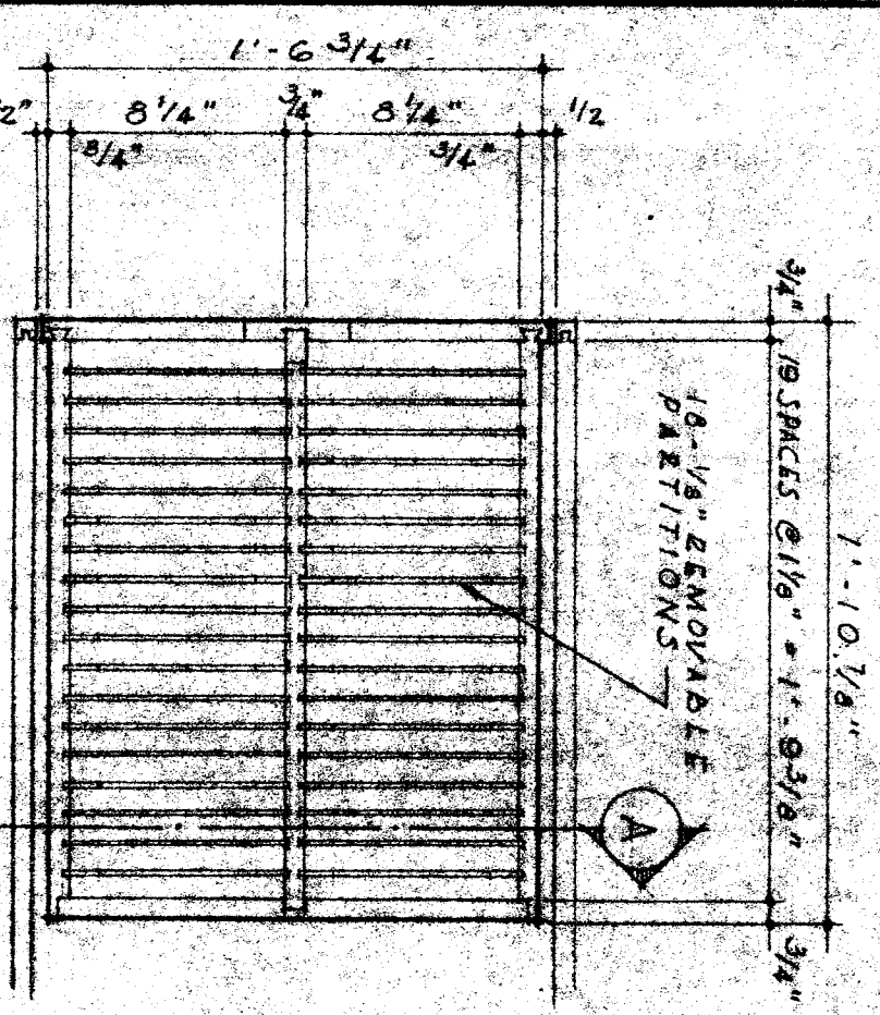
5 PLAN OF CARD FILE DRAWER - 1/2 x 1'-0"
