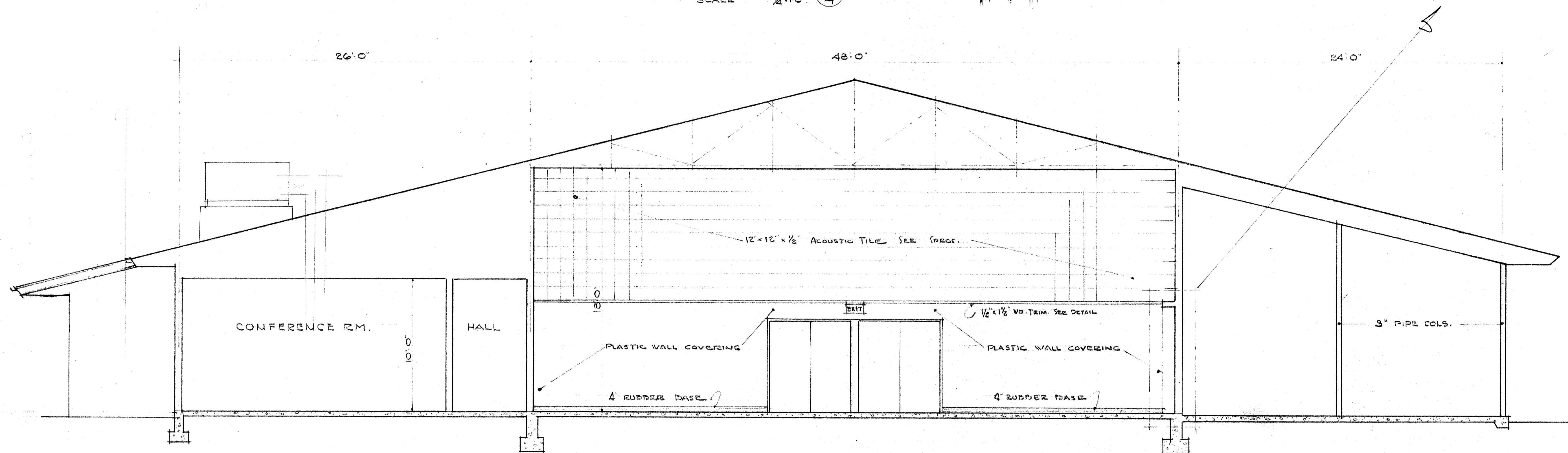
SECTION B SCALE 1/4" = 1'-0" 4
