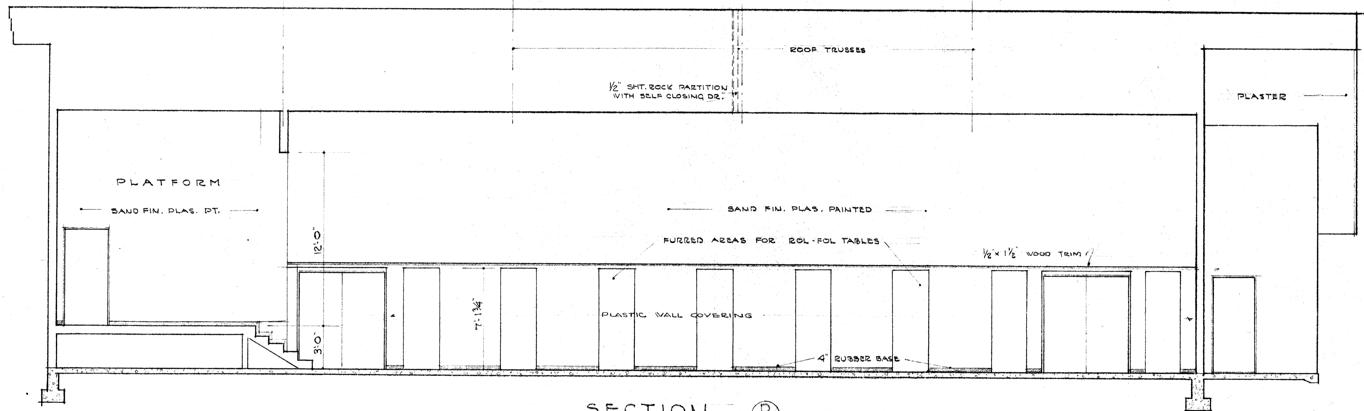
SECTION D SCALE 1/4" = 1'-0"
