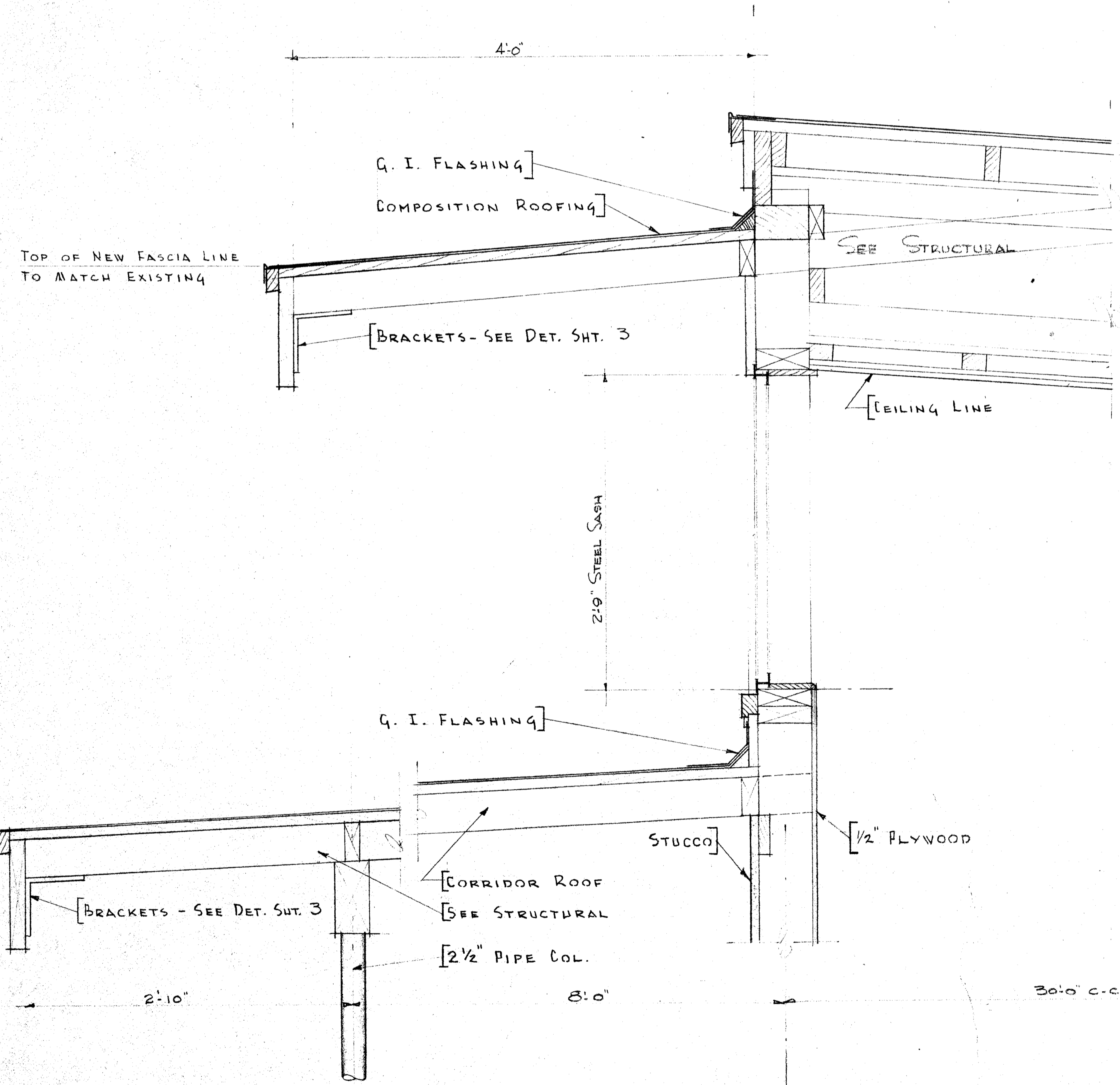
TYPICAL SECTION THRU CLASS ROOM & KINDERGARTEN SCALE 1/2" = 1'-0"
