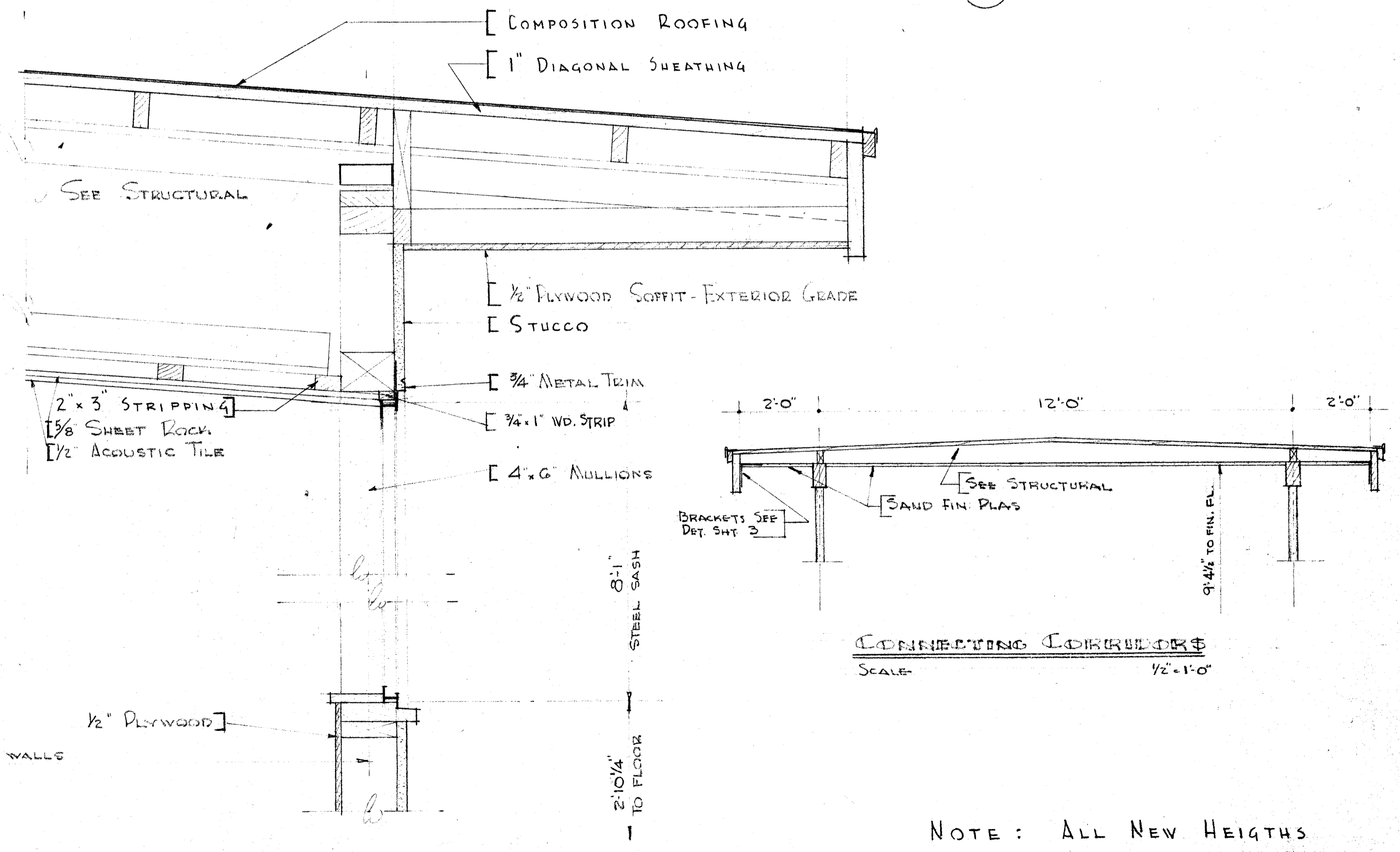
TYPICAL SECTION THRU CLASS ROOM & KINDERGARTEN SCALE 1/2" = 1'-0"
