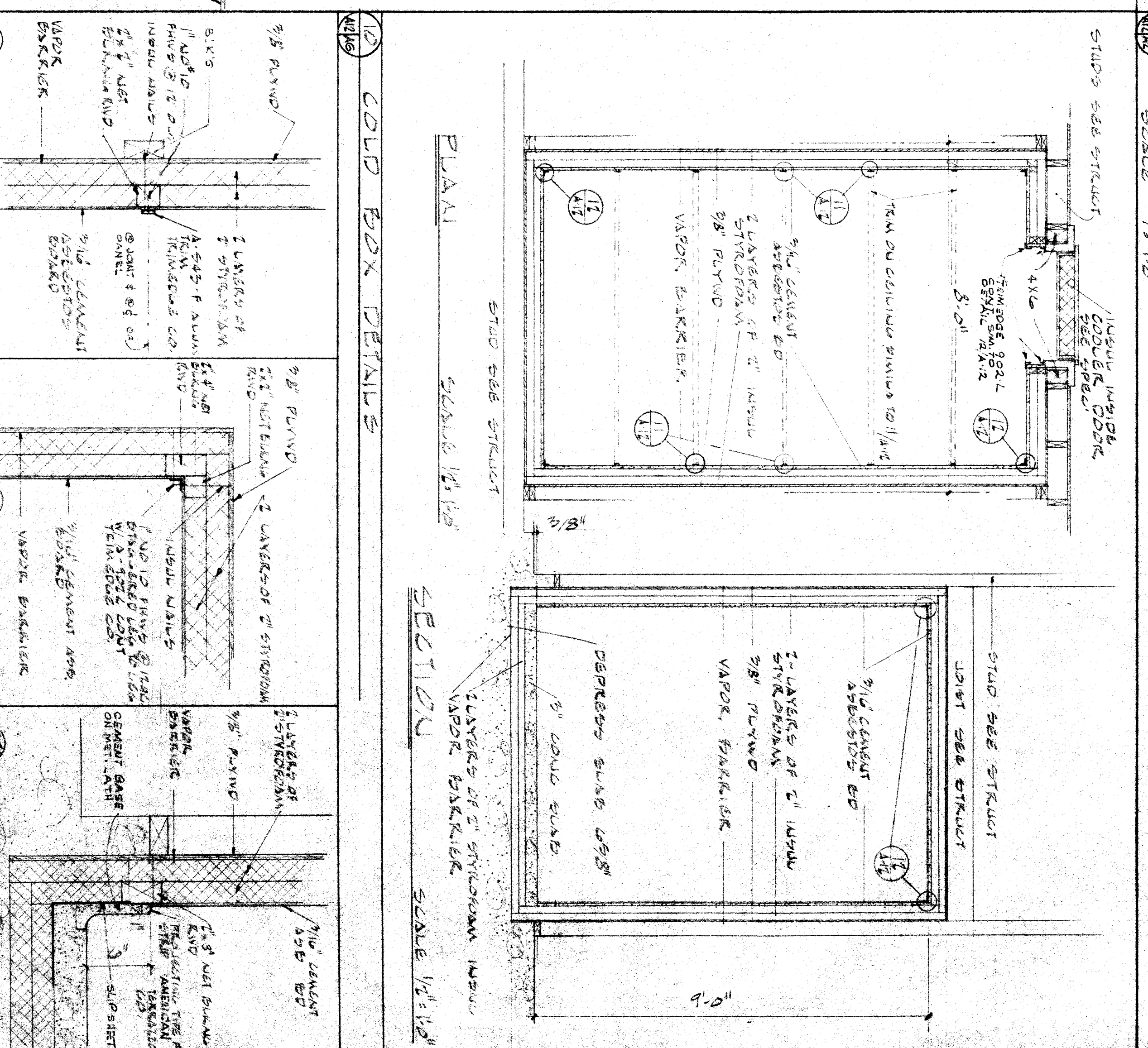
10 COLD BOX DETAILS SCALE 1/4\"/>
