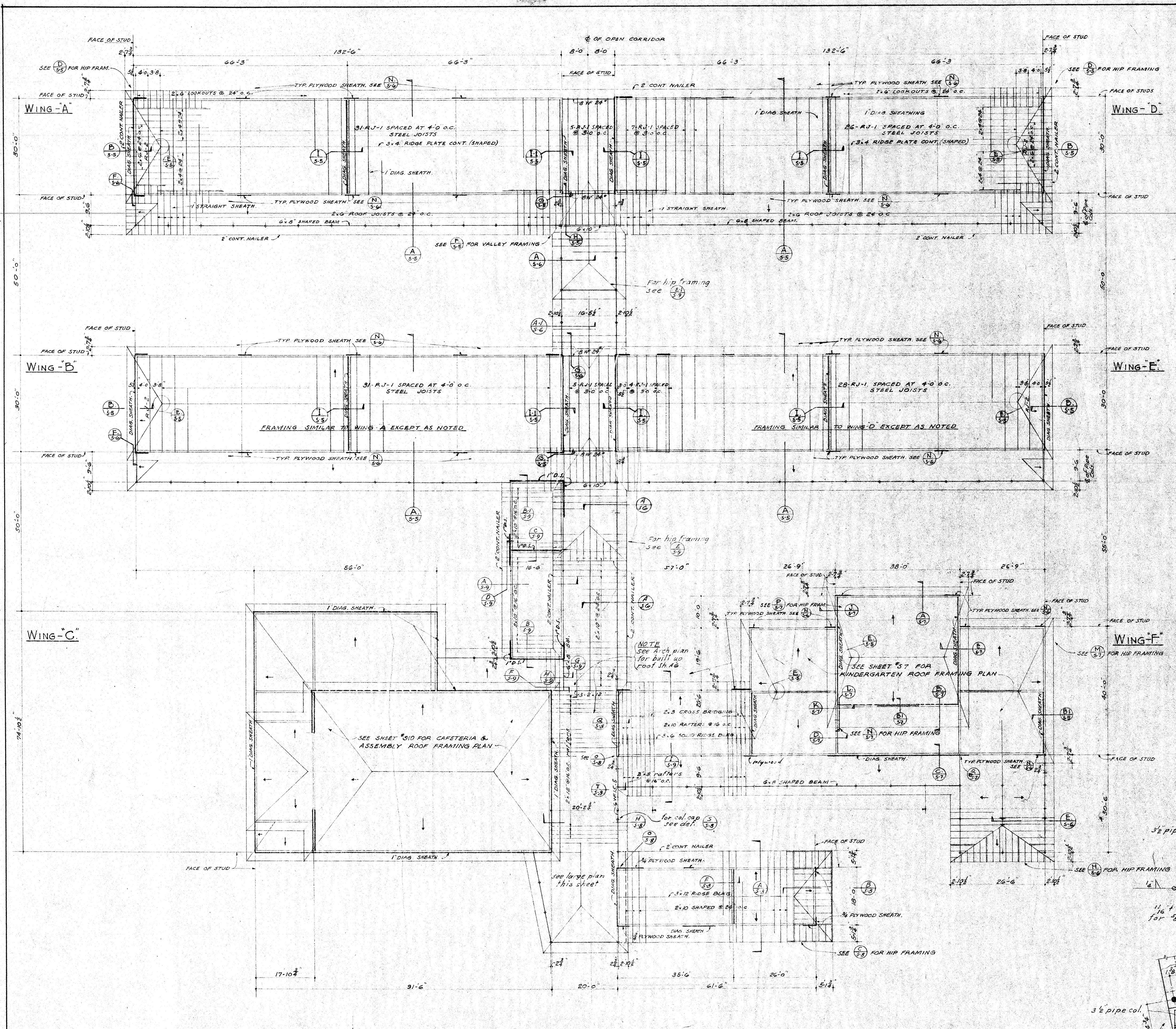
ROOF FRAMING PLAN SCALE - 1/2" = 1'-0"
