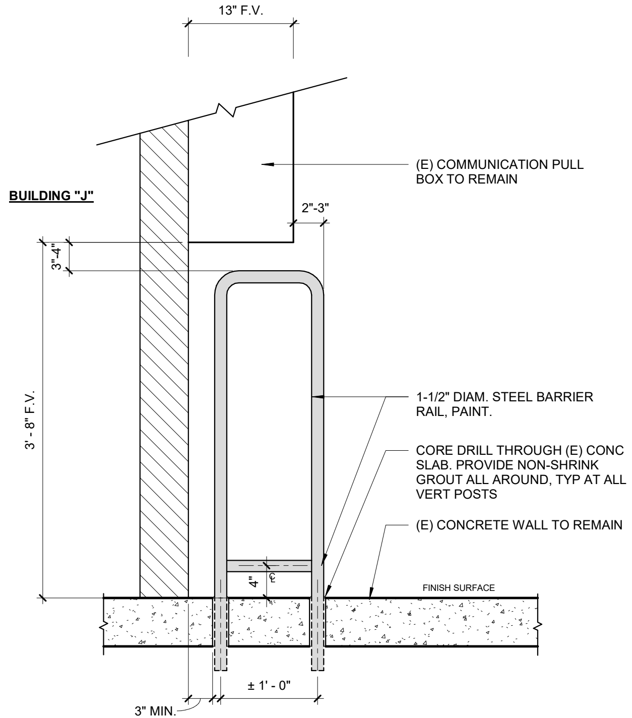
① BUILDING 'J' - BARRIER RAIL 1" = 1'-0"
