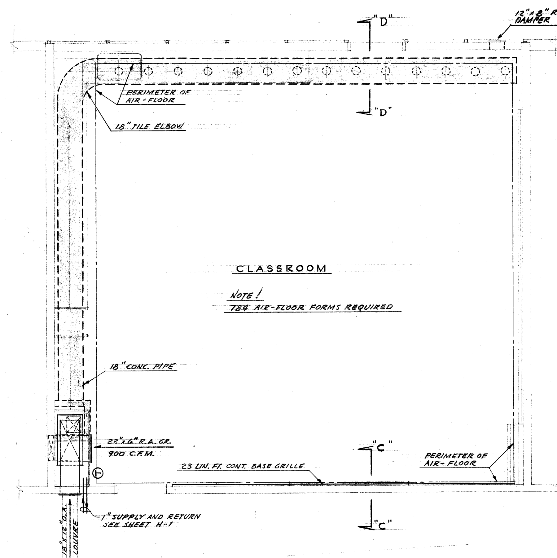
TYPICAL PLAN-PRIMARY GRADES SCALE 1/4" = 1'-0"
