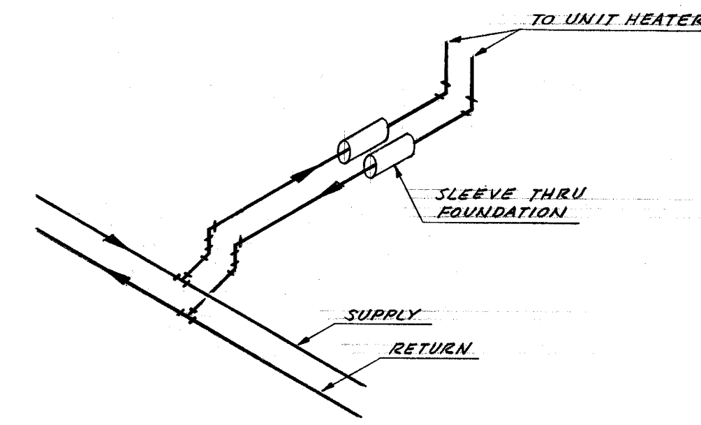
ISOMETRIC SHOWING TYPICAL PIPE CONNECTIONS @ UNIT HEATERS
