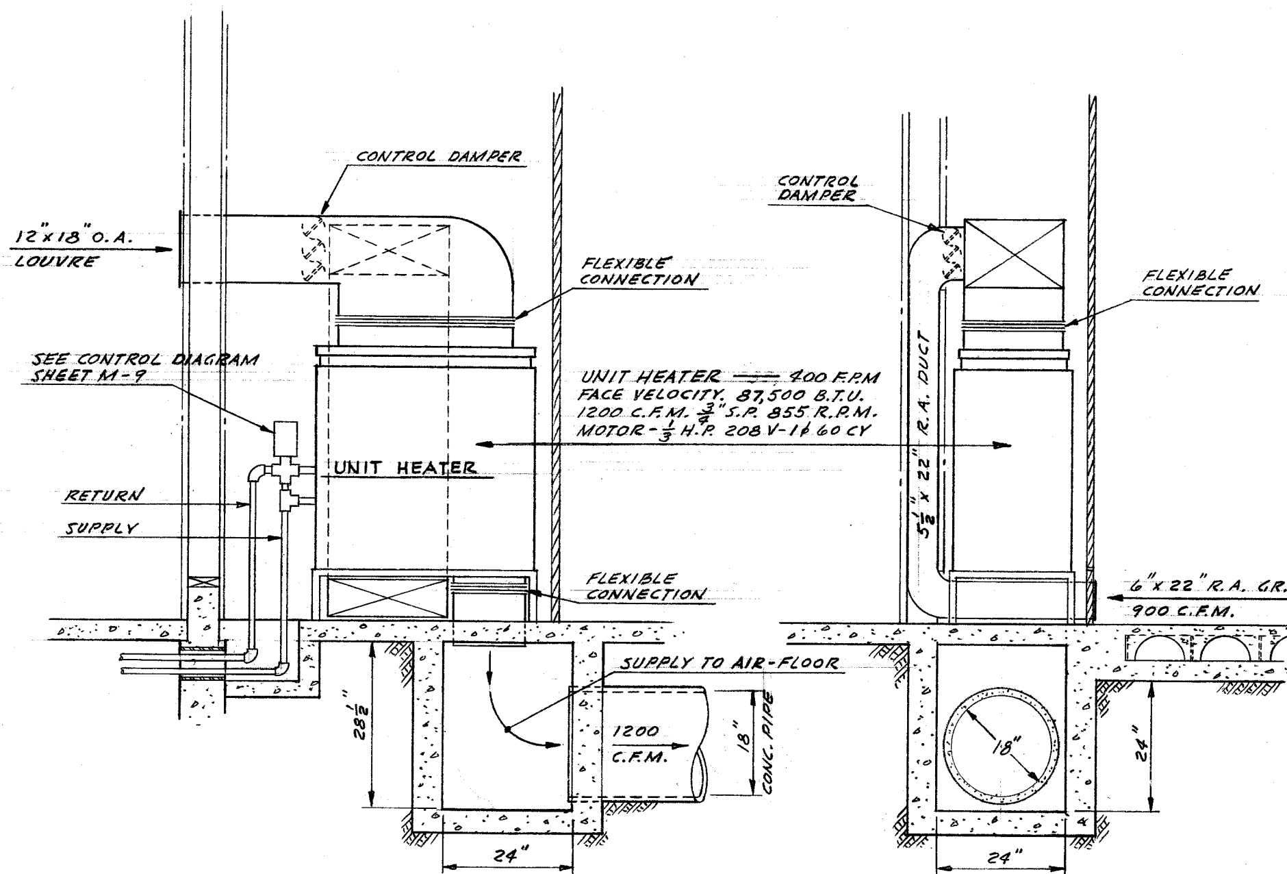
SECTION - "A" - "A" SECTION - "B" - "B" SCALE 1/2" = 1'-0"
