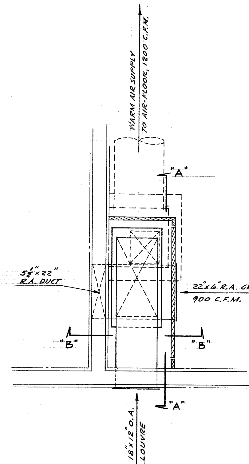
PLAN - HEATER UNIT TYPICAL CLASSROOM SCALE 1/2" = 1'-0"
