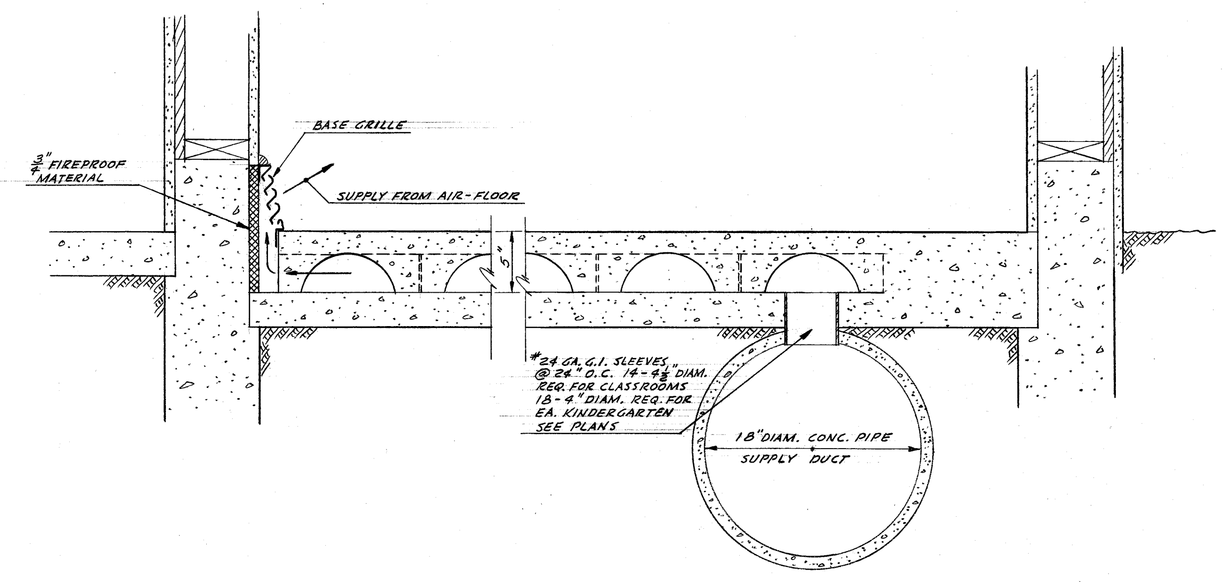
SECTION - "C" - "C" SECTION - "D" - "D" SCALE 1/2" = 1'-0"
