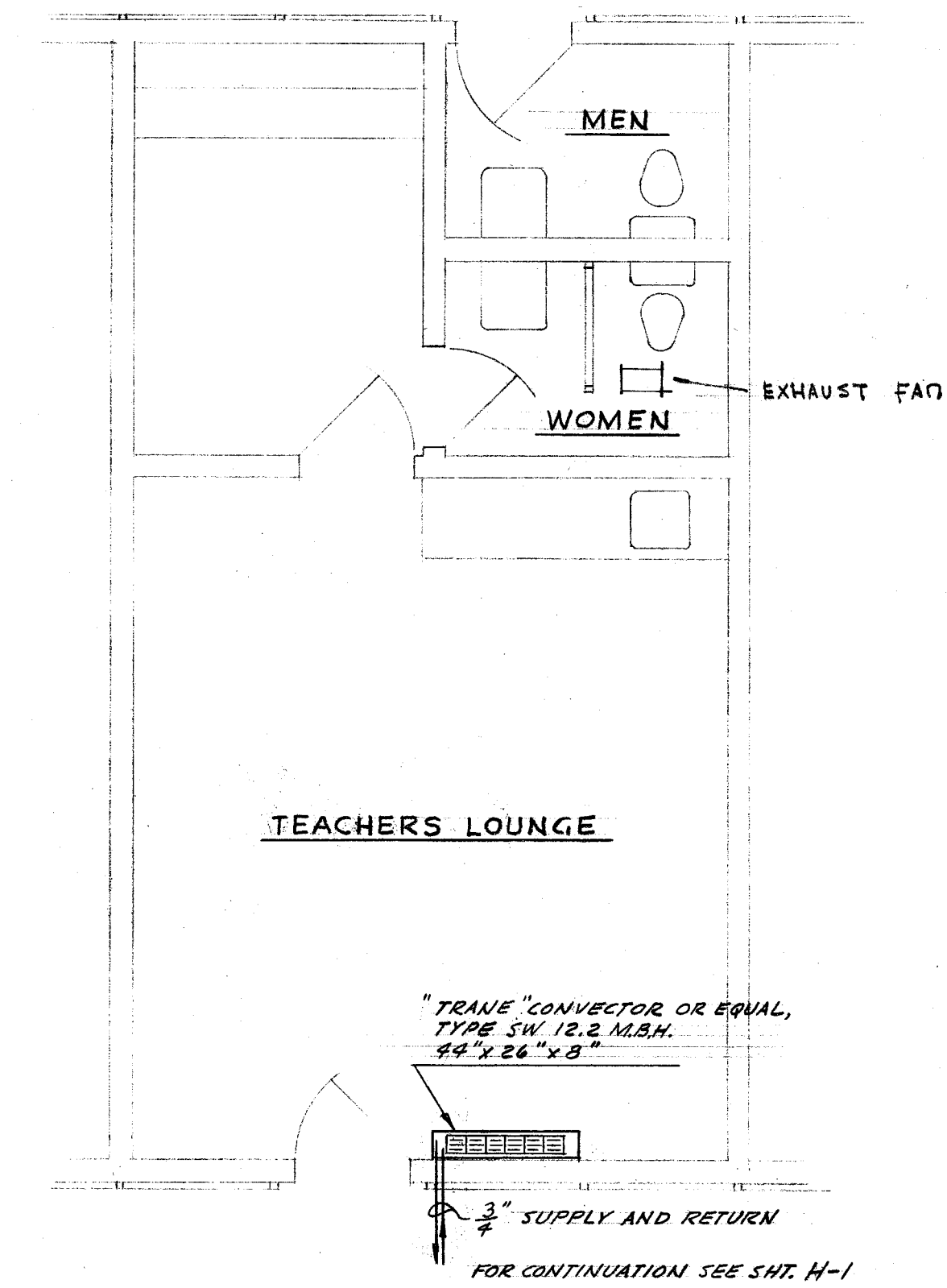
PLAN AT UNIT FOUR SCALE 1/4" = 1'-0"
