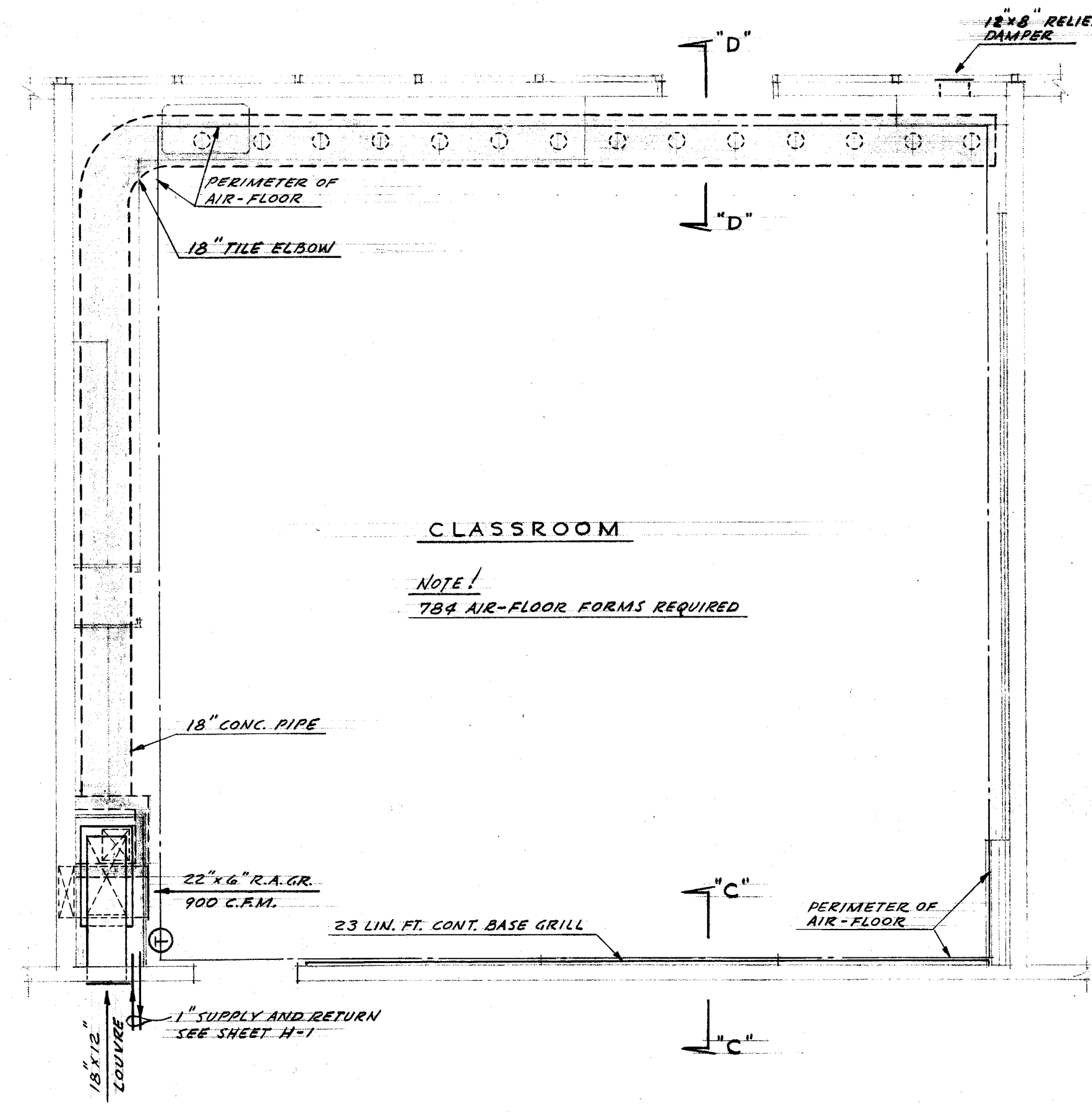
TYPICAL PLAN-INTERMEDIATE GRADES SCALE 1/4" = 1'-0"
