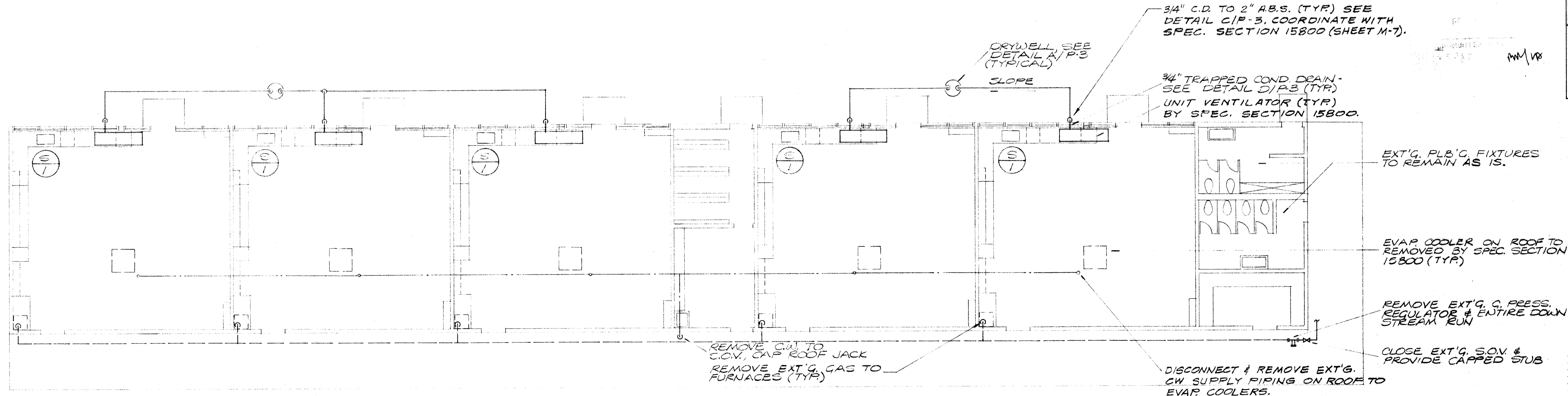
PLUMBING FLOOR PLAN UNIT E SCALE: 1/8" = 1'-0"
