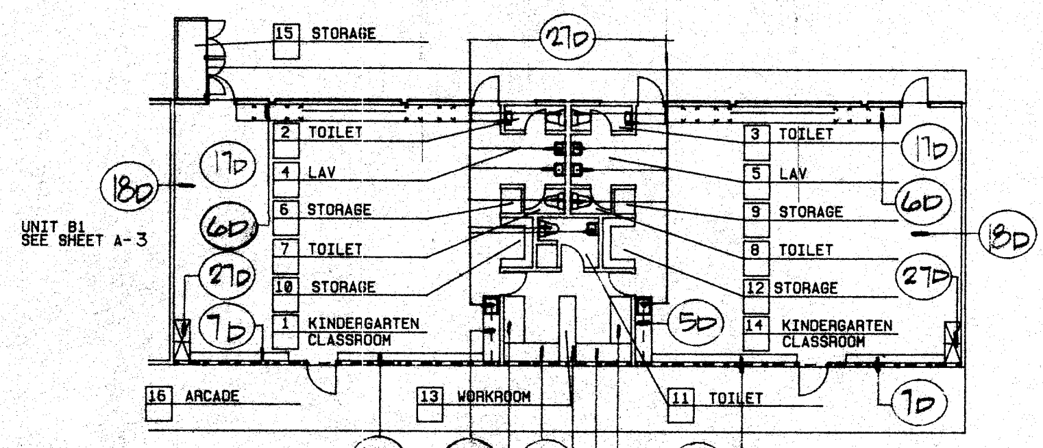
FLOOR PLAN - UNIT 82 (DEMOLITION/EXISTING PLAN) 1/8" = 1'-0"
