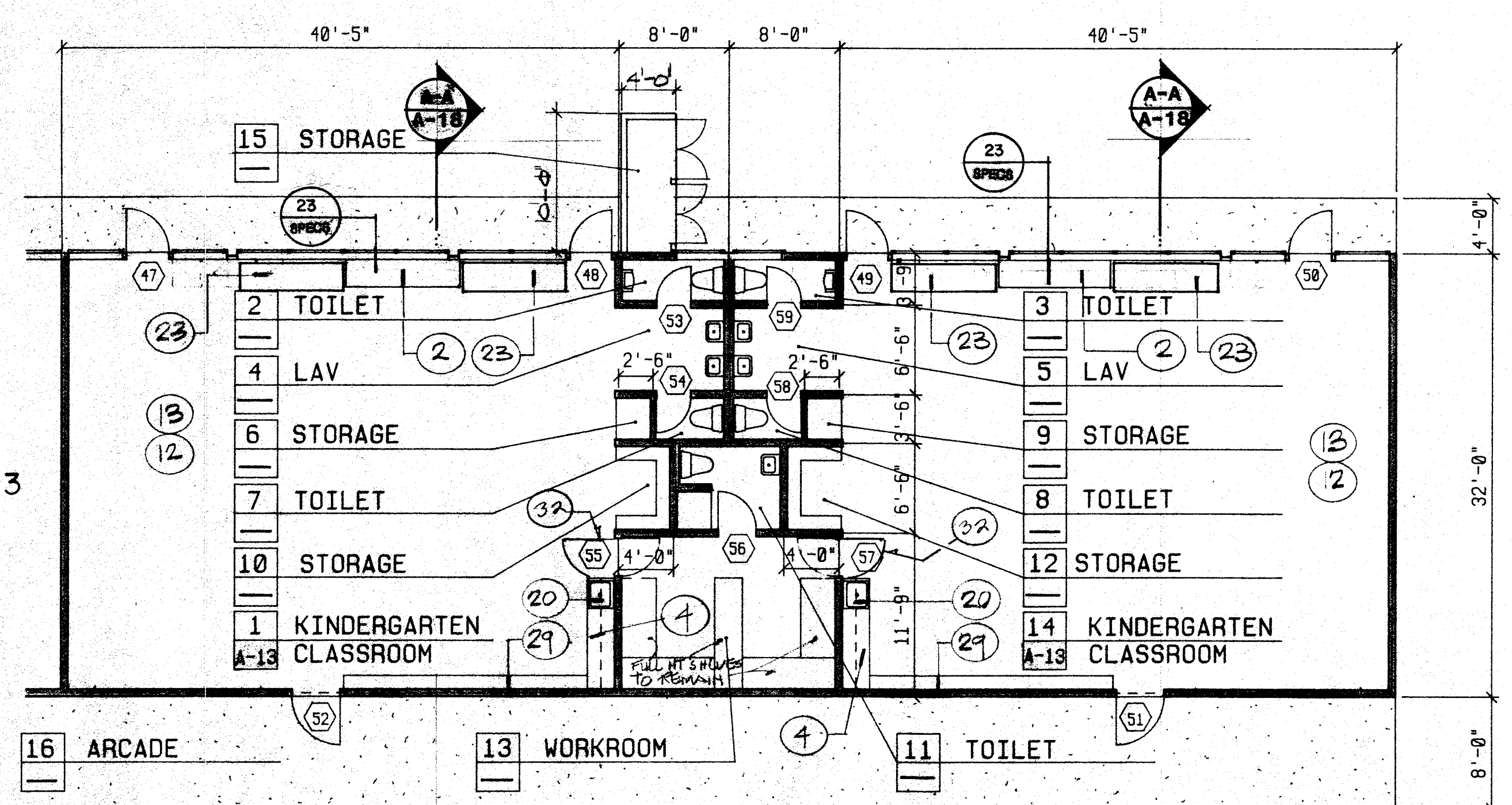
FLOOR PLAN - UNIT 82 (NEW) NOTE 1. FOR DOOR/HARDWARE INFORMATION REFER TO DOOR SCHEDULE. 2. FOR FINISH INFORMATION REFER TO FINISH SCHEDULE. 1/8" = 1'-0"
