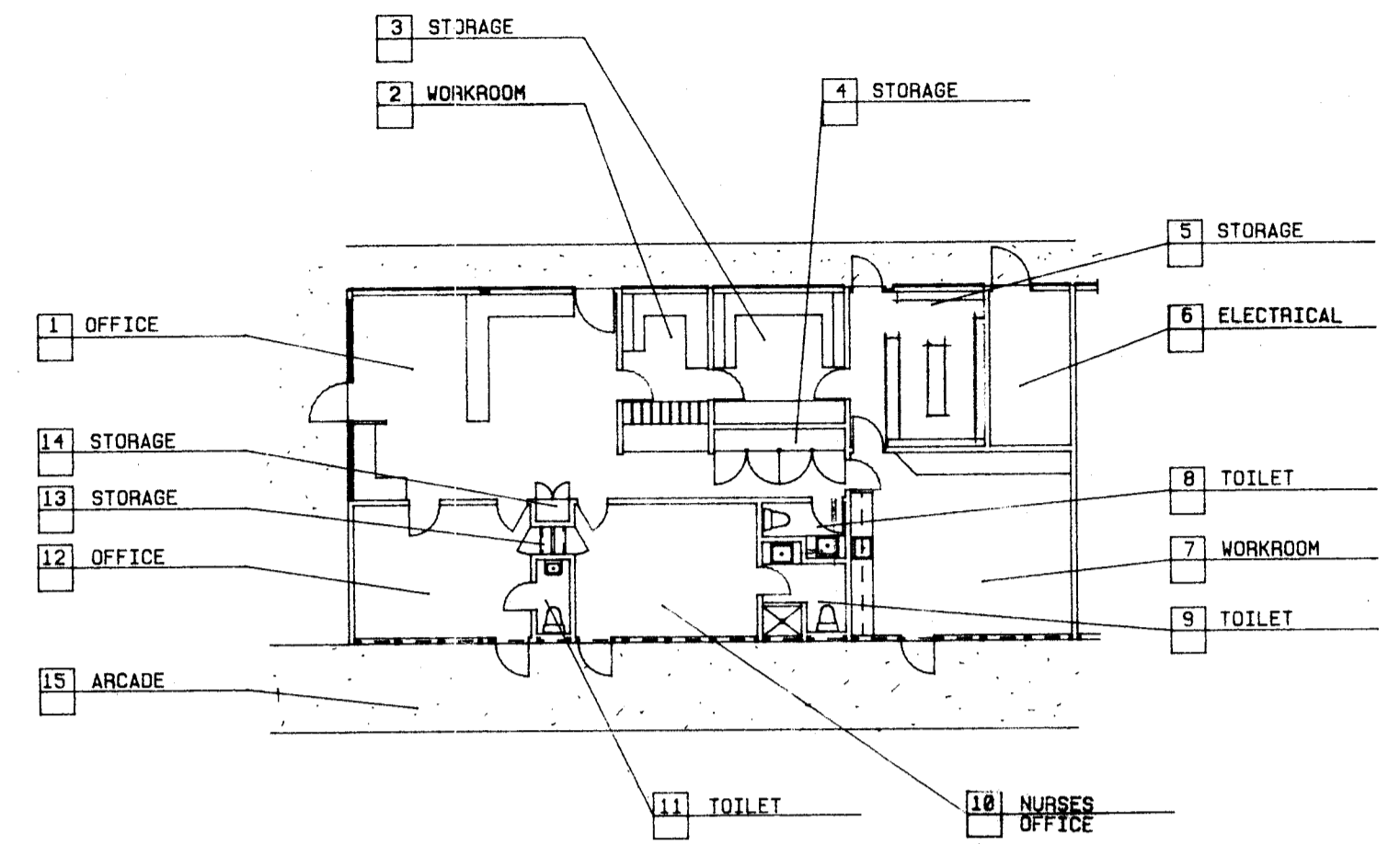
FLOOR PLAN - UNIT B1 (DEMOLITION/EXISTING PLAN) 1/8" = 1'-0"
