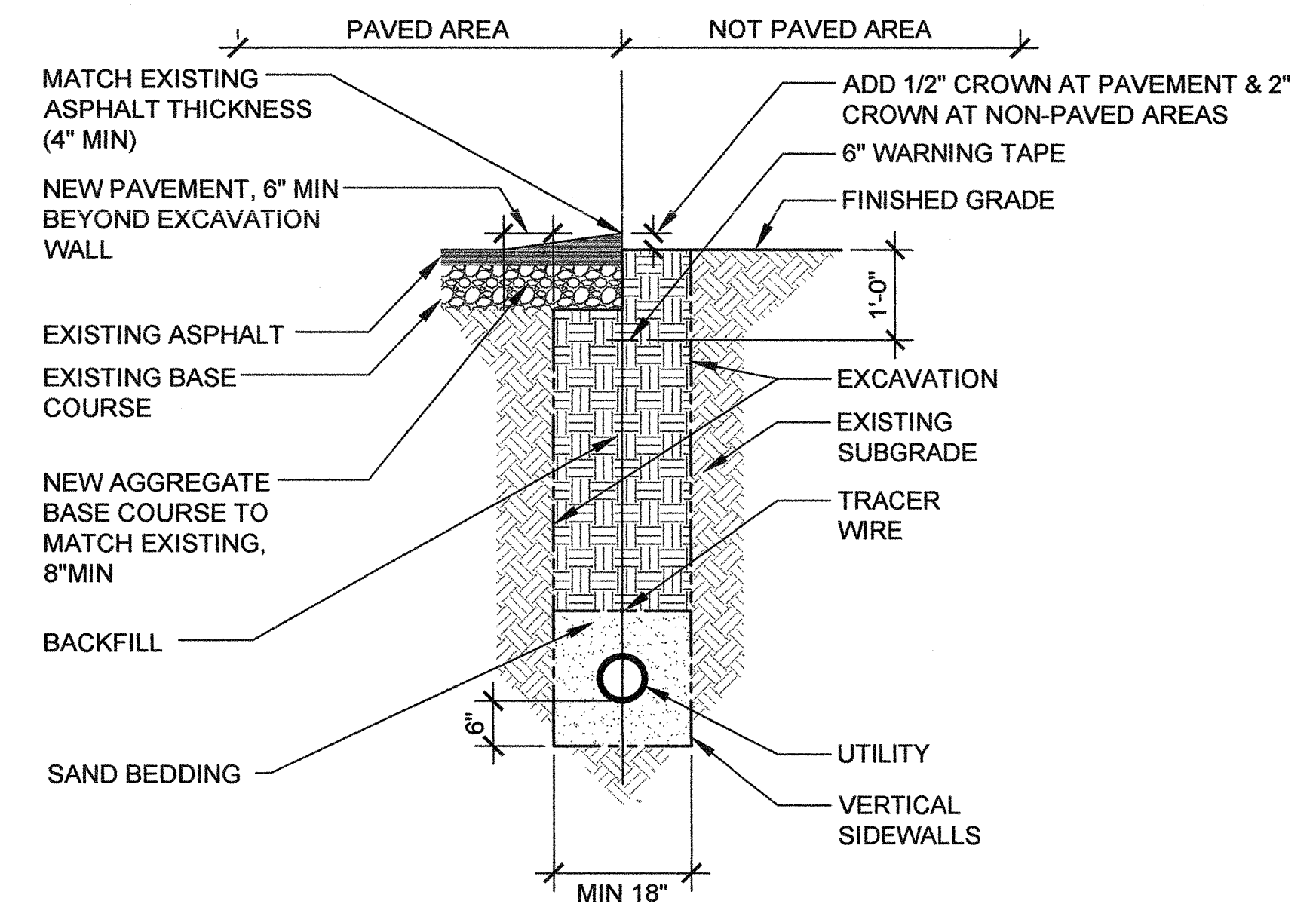
1 TRENCH DETAIL
