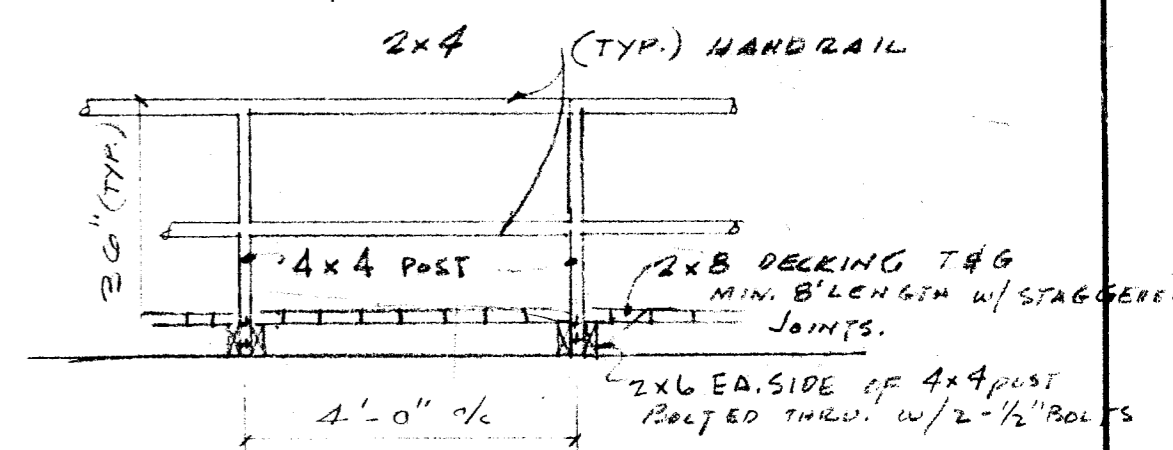
RAILING DETAIL NO SCALE
