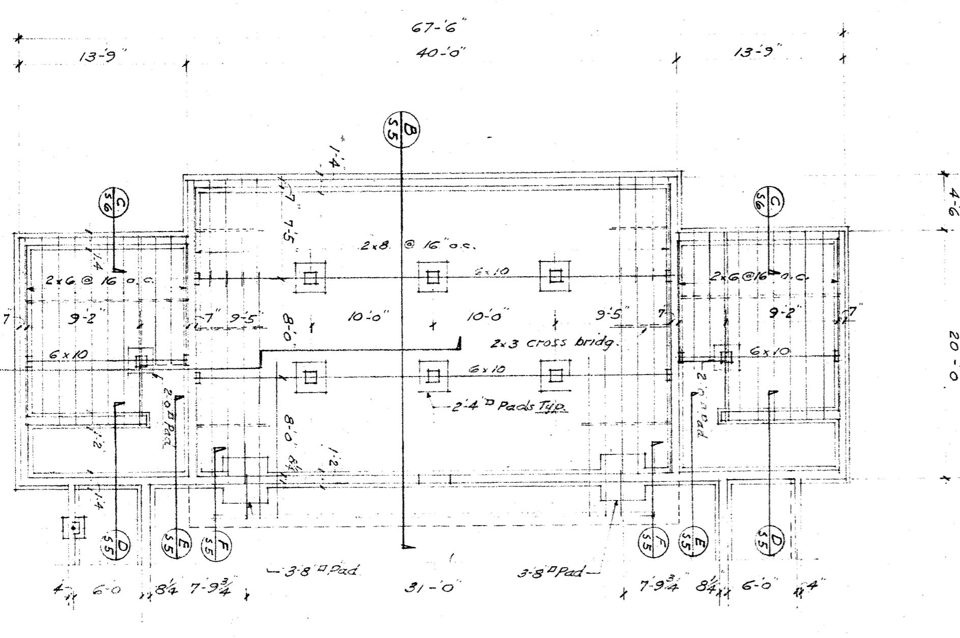
PLATFORM FOUNDATION & FRAMING PLAN
