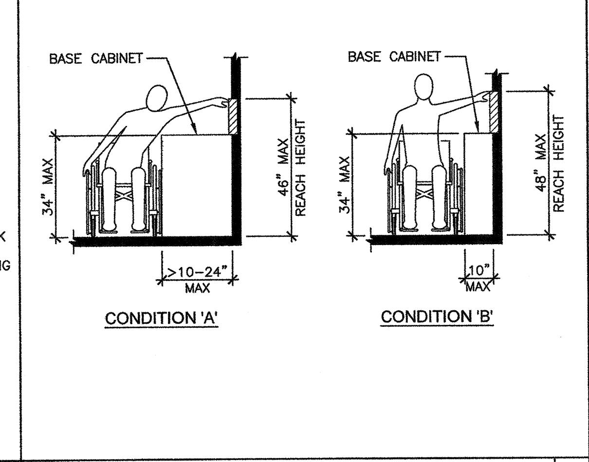
SIDE REACH AT BASE CABINET NOT TO SCALE 13
