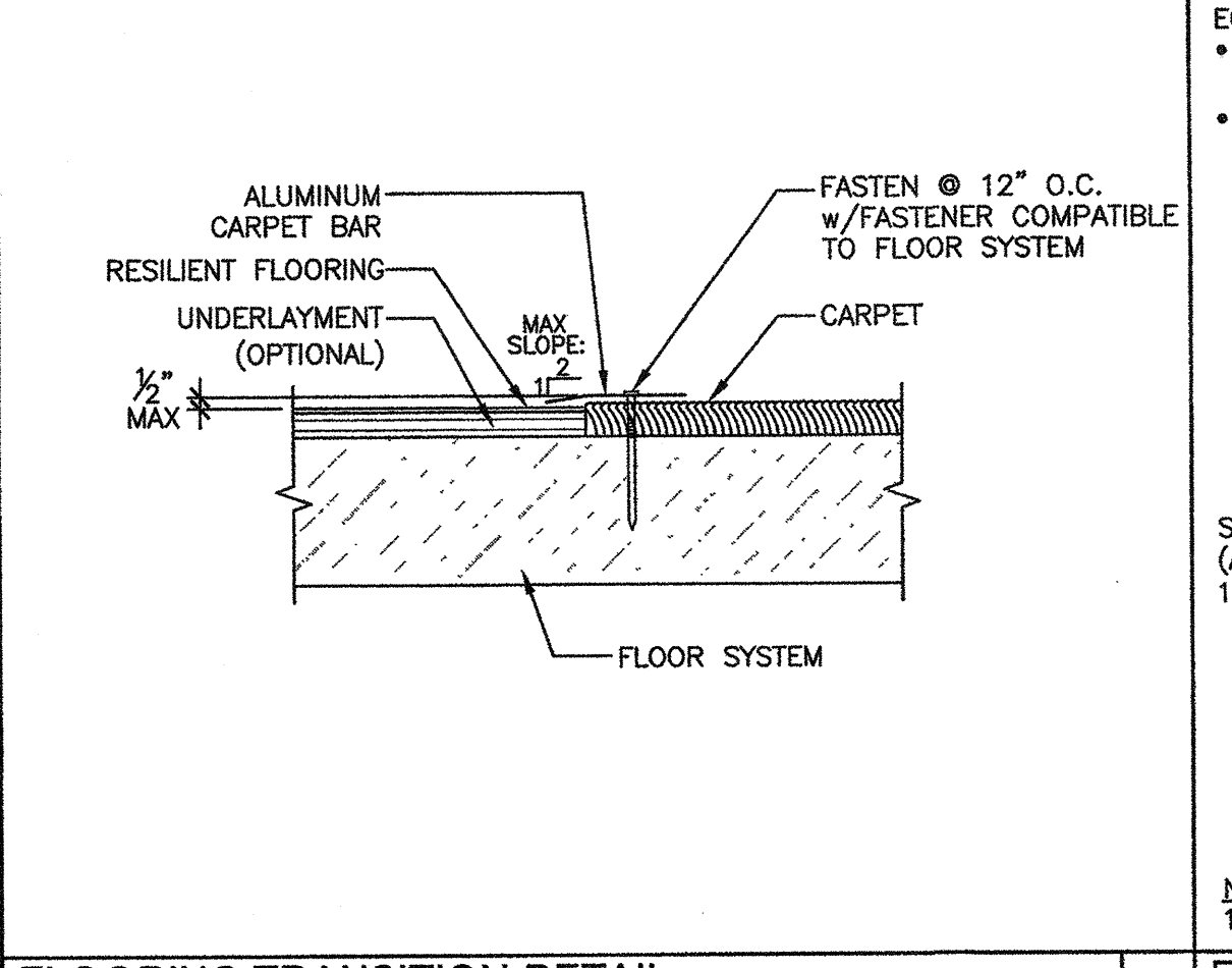
FLOORING TRANSITION DETAIL NOT TO SCALE 14
