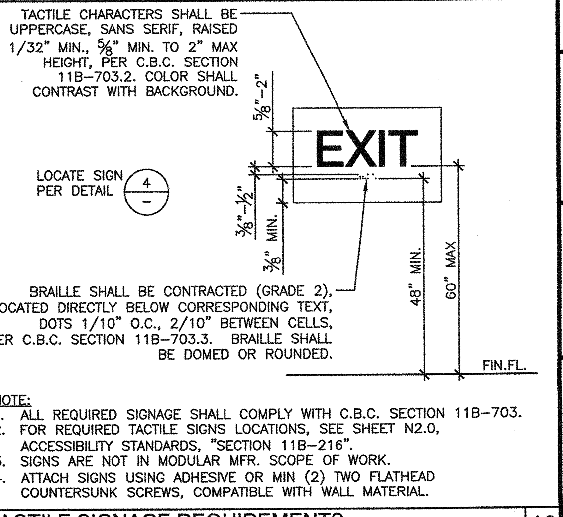
TACTILE SIGNAGE REQUIREMENTS NOT TO SCALE 10
