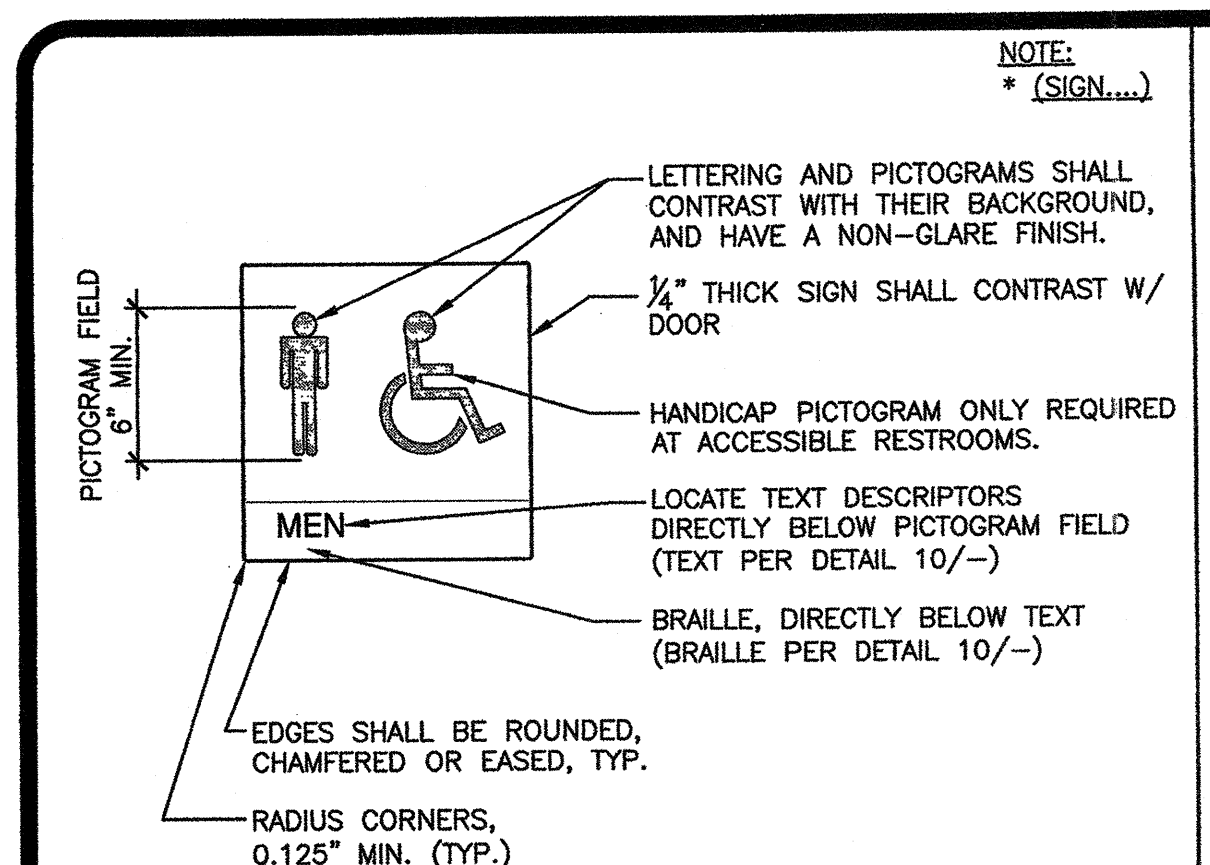
WALL MOUNTED RESTROOM SYMBOLS-MEN NOT TO SCALE 1
