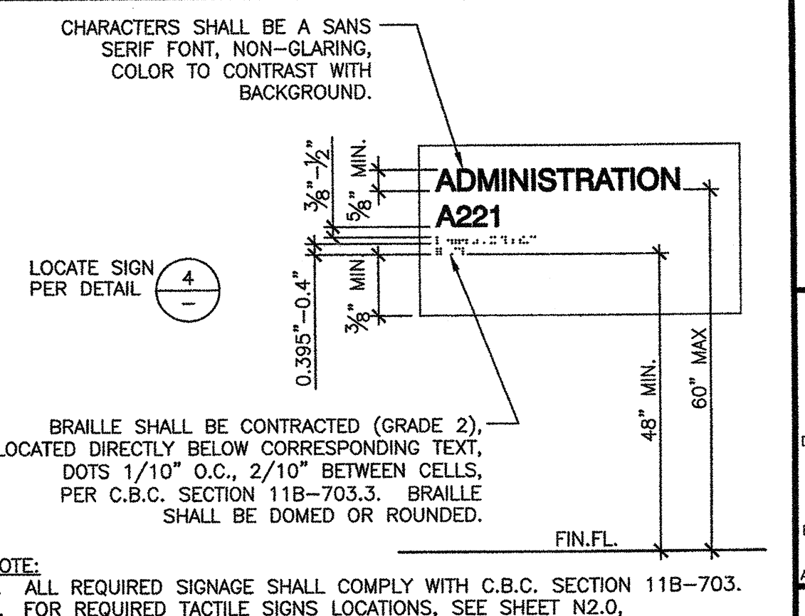
PERMANENT ROOM I.D. SIGNAGE NOT TO SCALE 5
