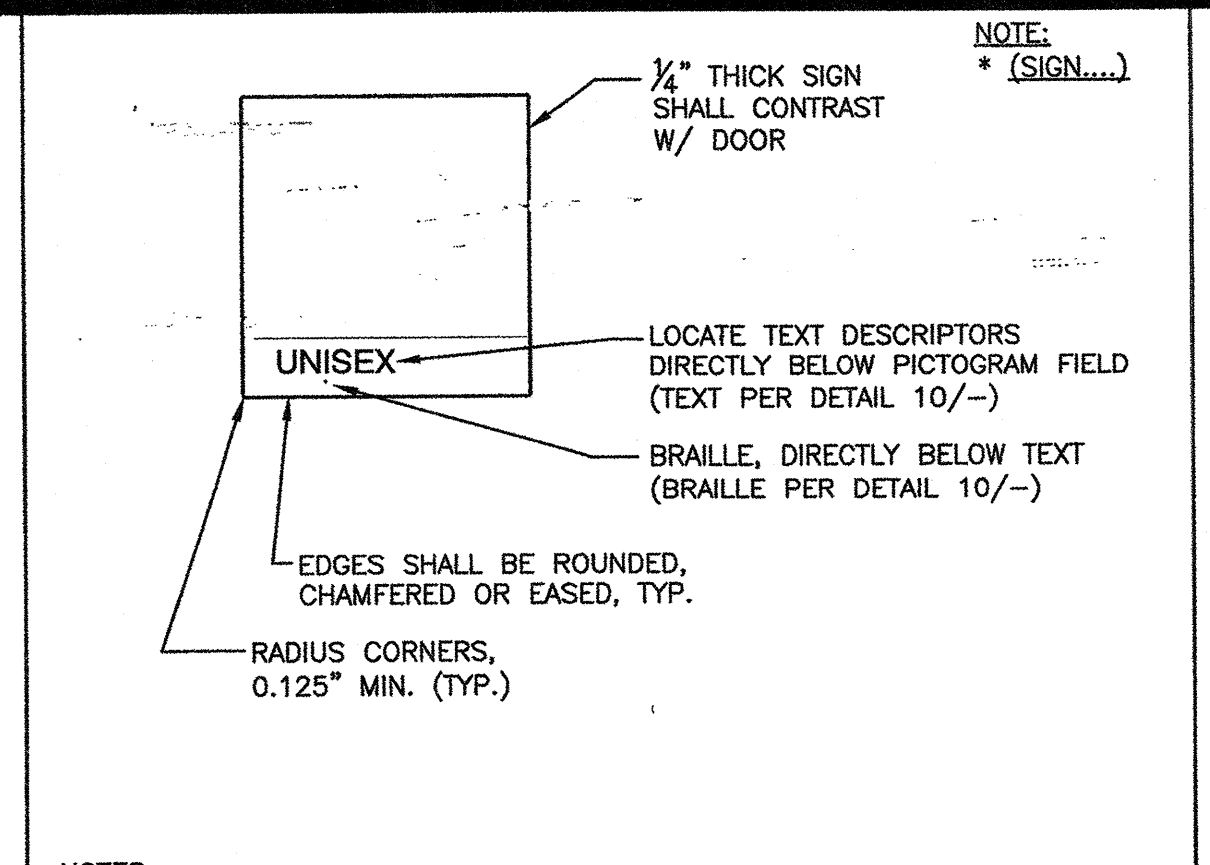
WALL MOUNTED RESTROOM SYMBOLS-UNISEX NOT TO SCALE 3
