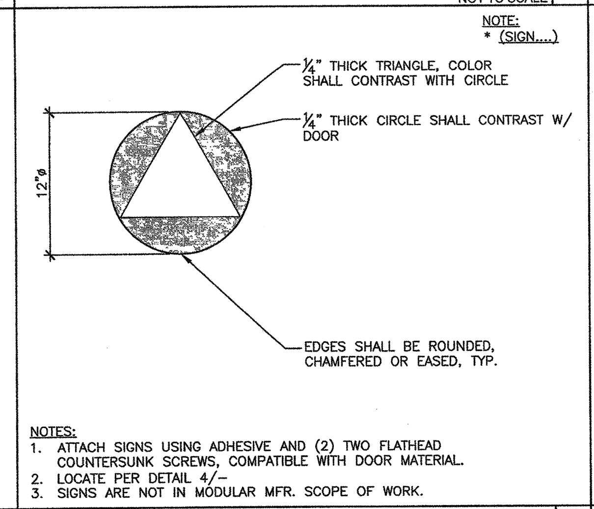
DOOR MOUNTED RESTROOM SYMBOLS-UNISEX NOT TO SCALE 8
