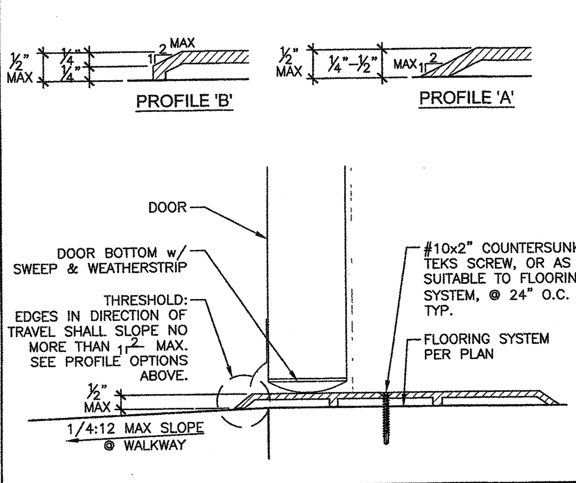
THRESHOLD @ EXTERIOR DOOR NOT TO SCALE 12
