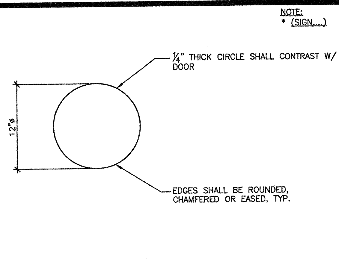
DOOR MOUNTED RESTROOM SYMBOLS-WOMEN NOT TO SCALE 2
