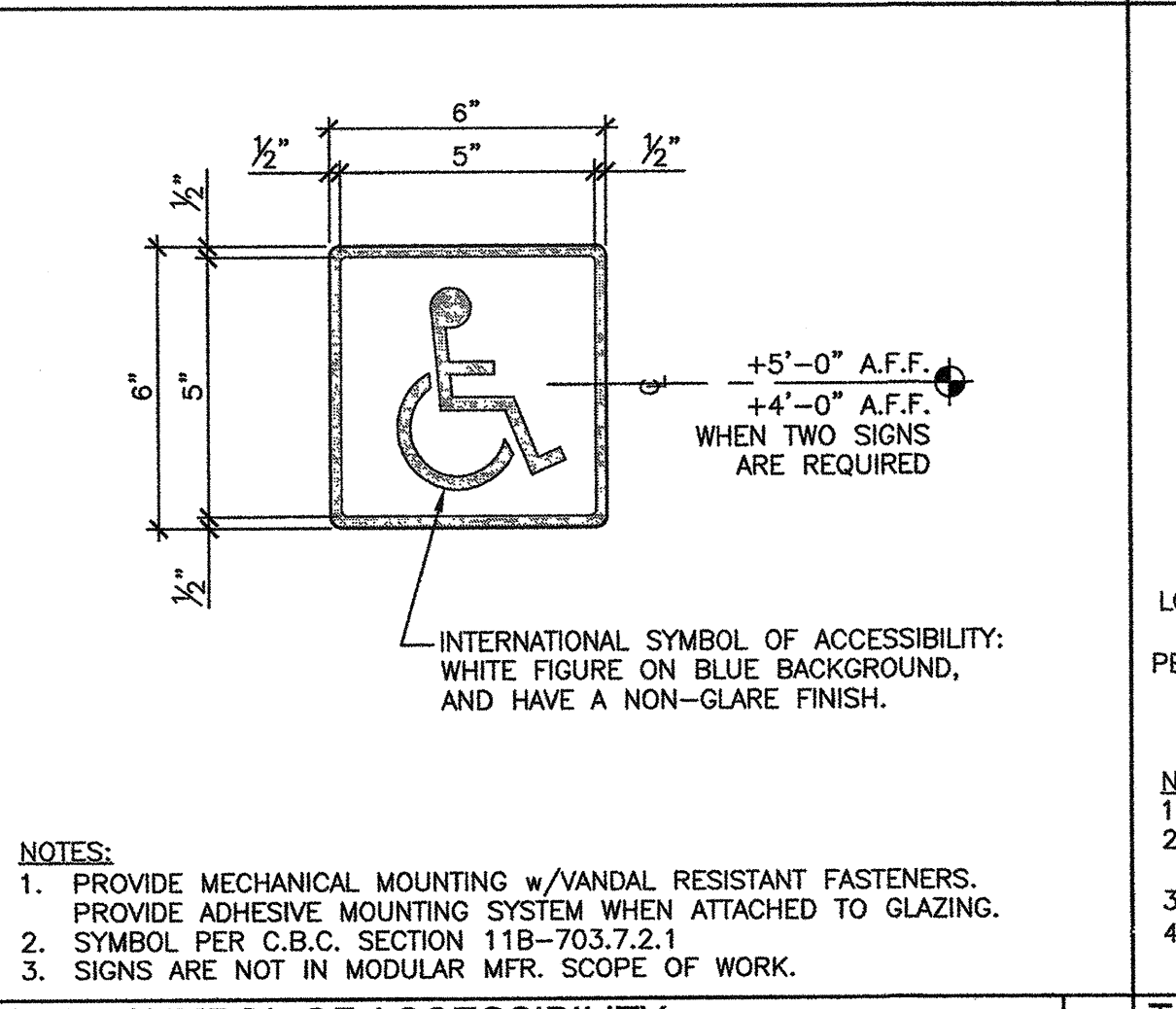
INT'L SYMBOL OF ACCESSIBILITY NOT TO SCALE 9
