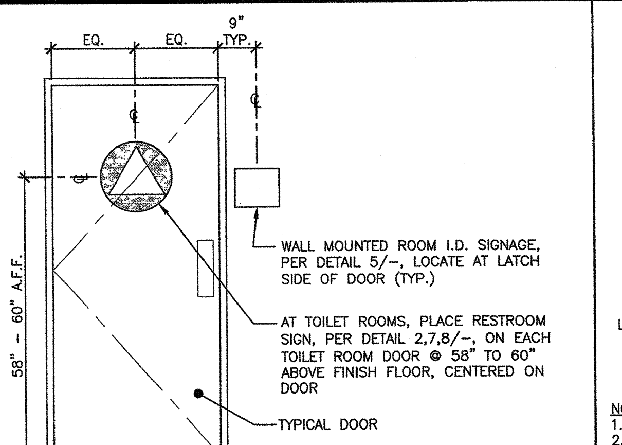
ROOM IDENTIFICATION SIGNAGE NOT TO SCALE 4
