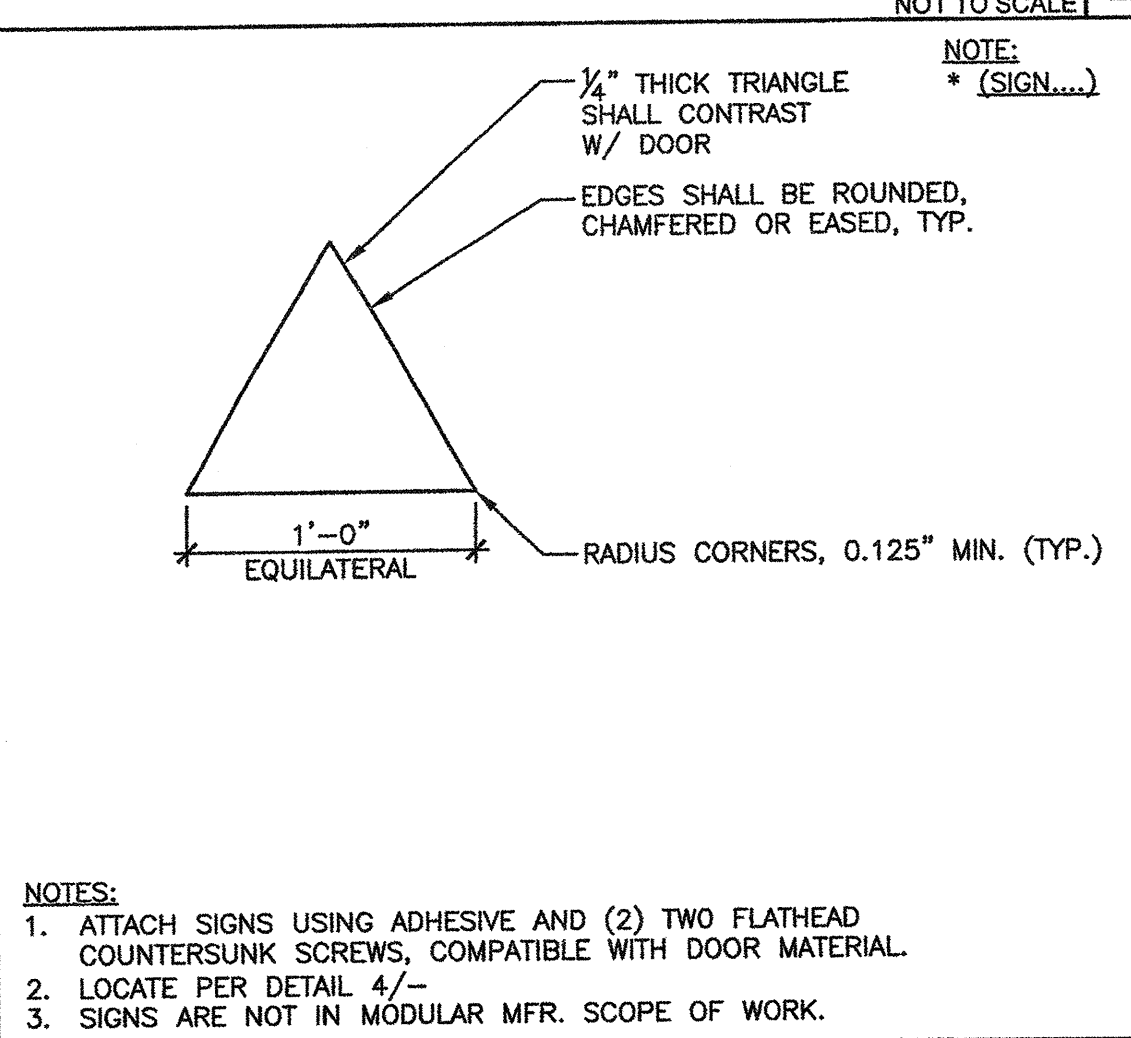
DOOR MOUNTED RESTROOM SYMBOL-MEN NOT TO SCALE 7
