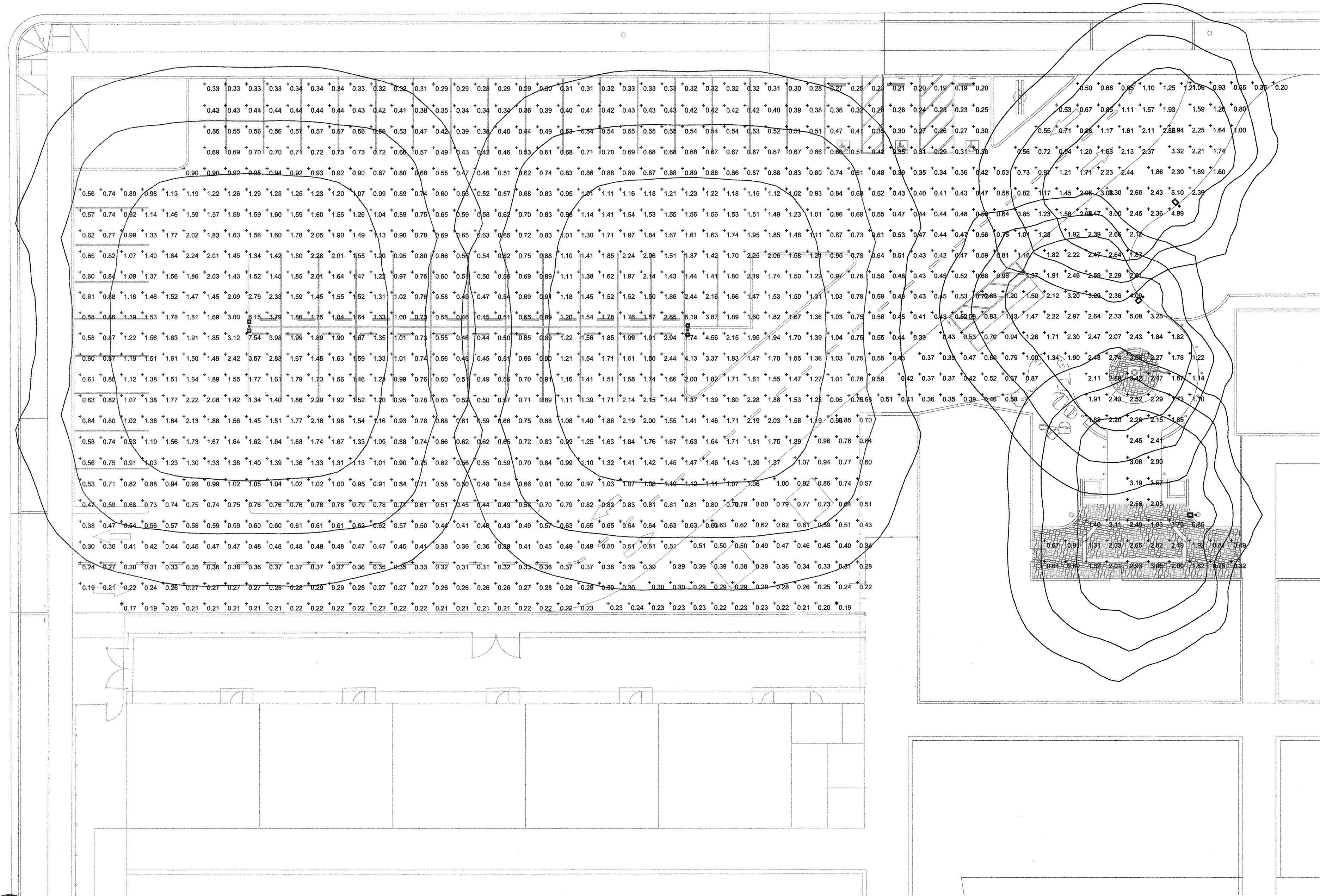
1 SITE PHOTOMETRIC PLAN SCALE: 1"=16'-0"
