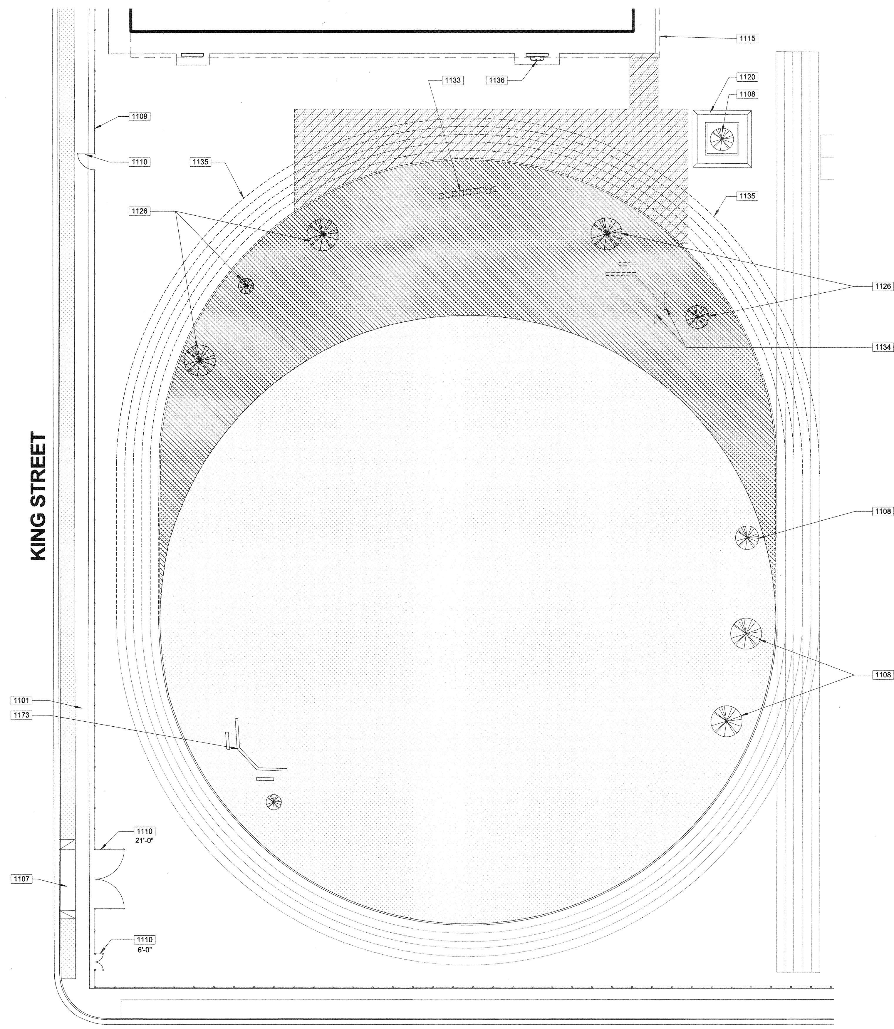
1 PARTIAL DEMOLITION SITE PLAN - TRACK
