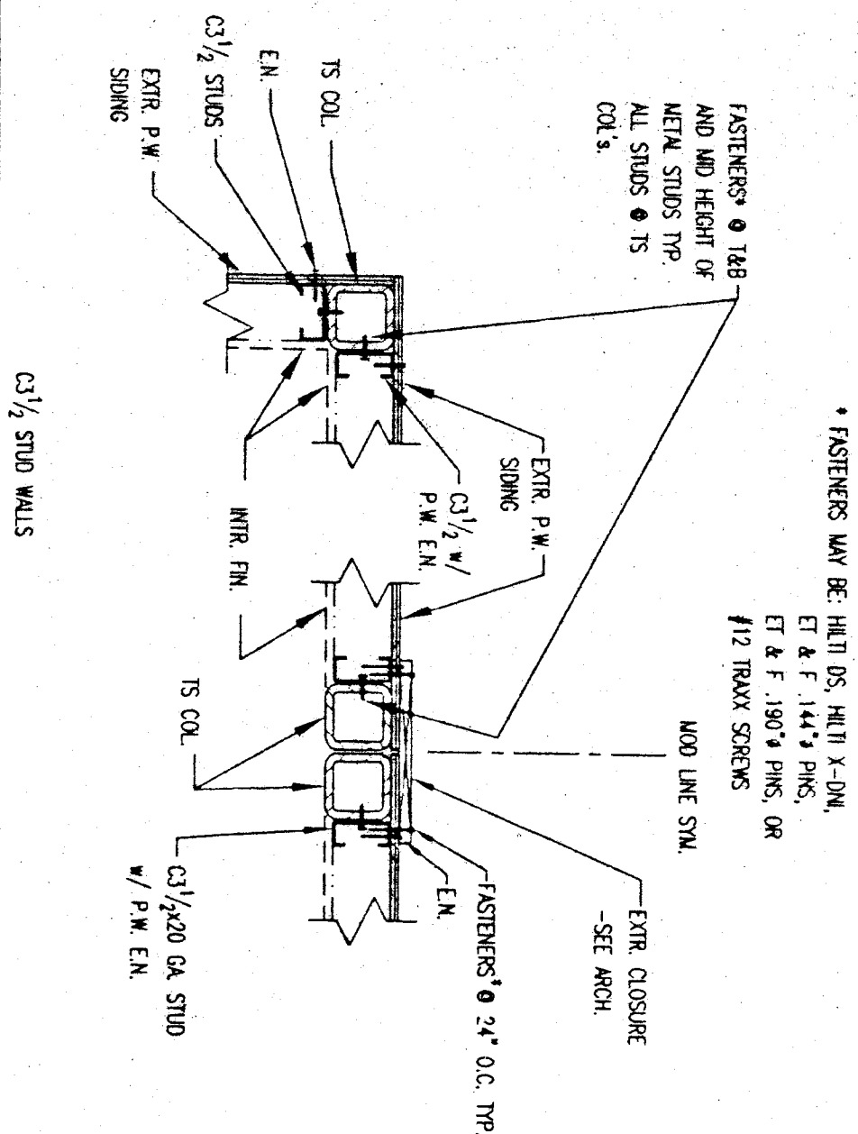
TYPICAL CORNER DETAILS - PLAN VIEW
