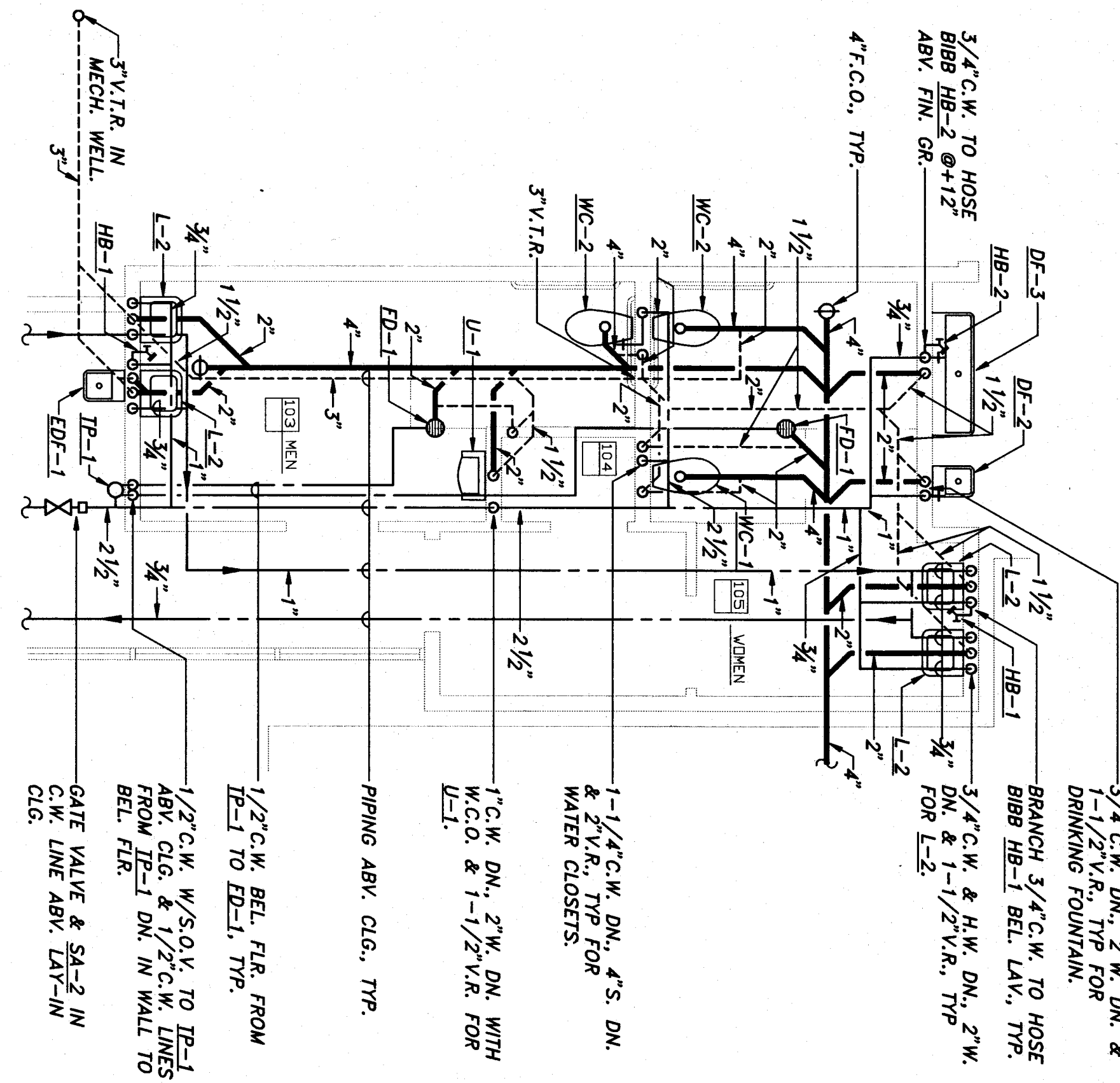
DETAILED PLUMBING PLAN - BLDG. "C" SCALE 1/4"=1'-0" P-6
