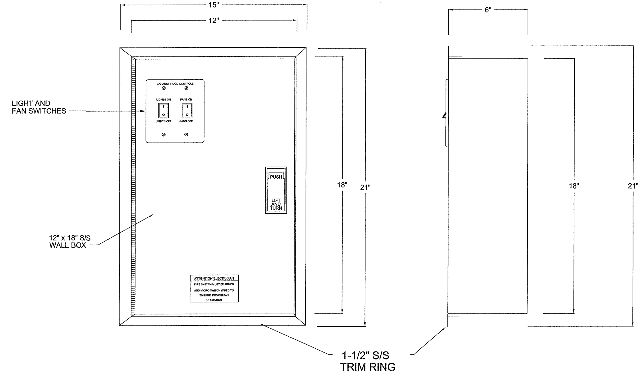
EX. HOOD H-A2 & A3 CONTROL PANEL
