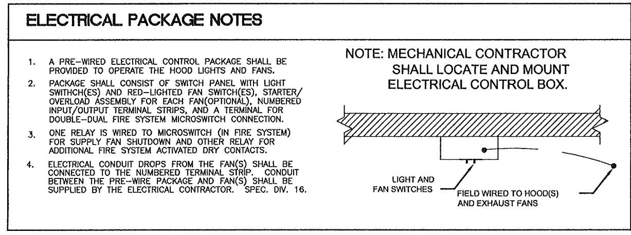
EX. HOOD H-A2 & A3 CONTROL PANEL
