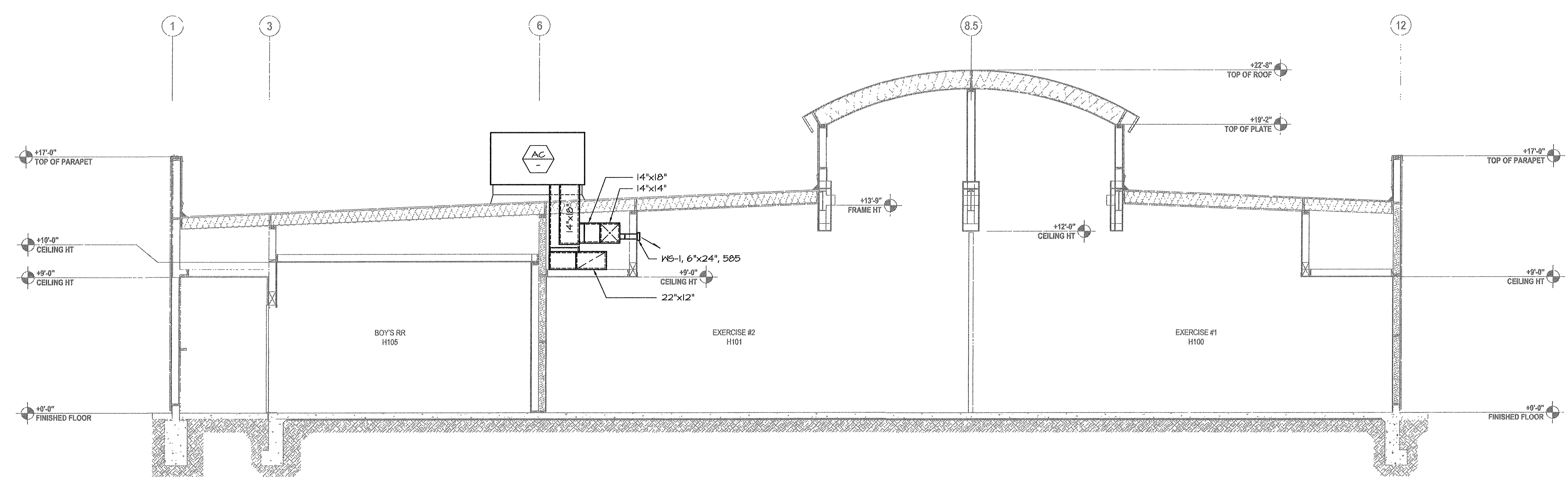
MECHANICAL SECTION - BUILDING H SCALE: 1/4"=1'-0"
