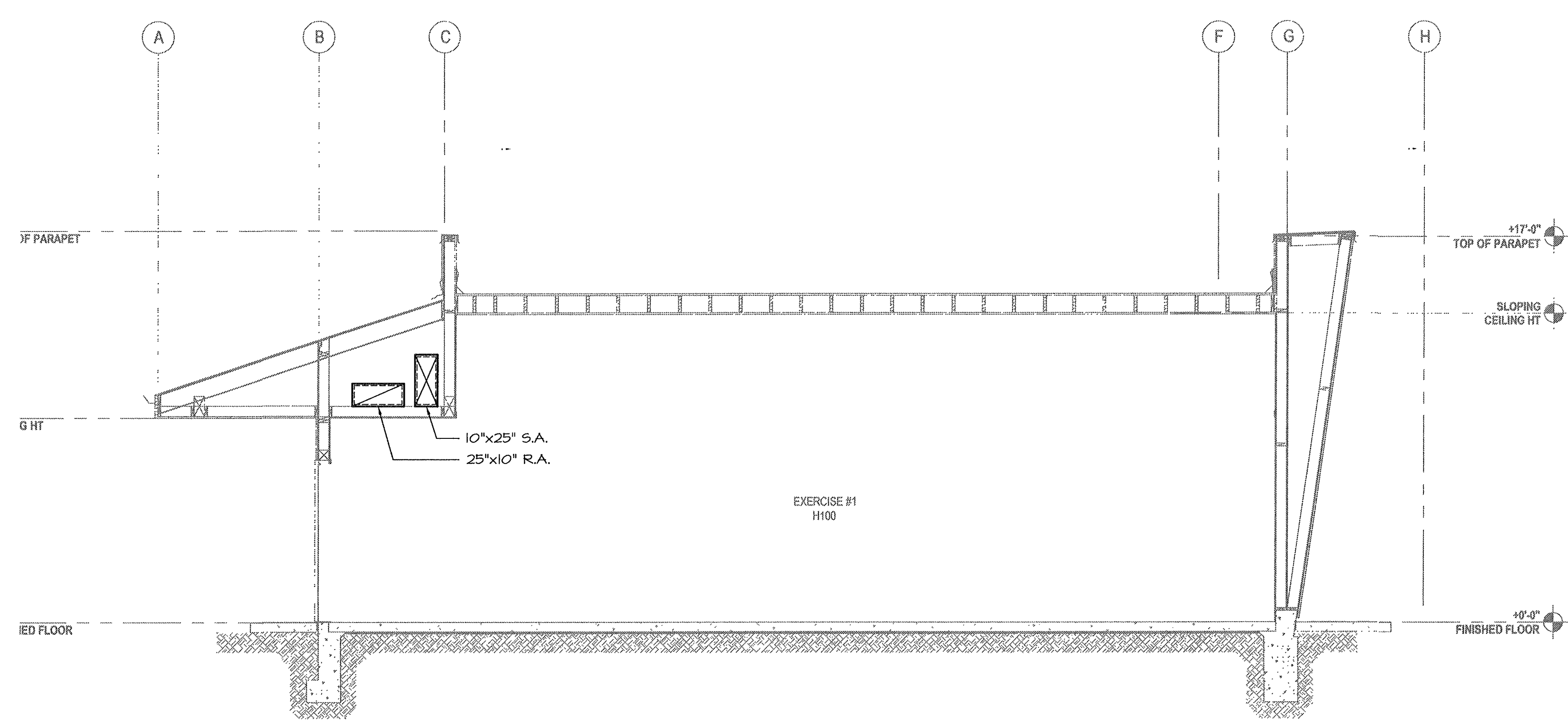
MECHANICAL SECTION - BUILDING H SCALE: 1/4"=1'-0"
