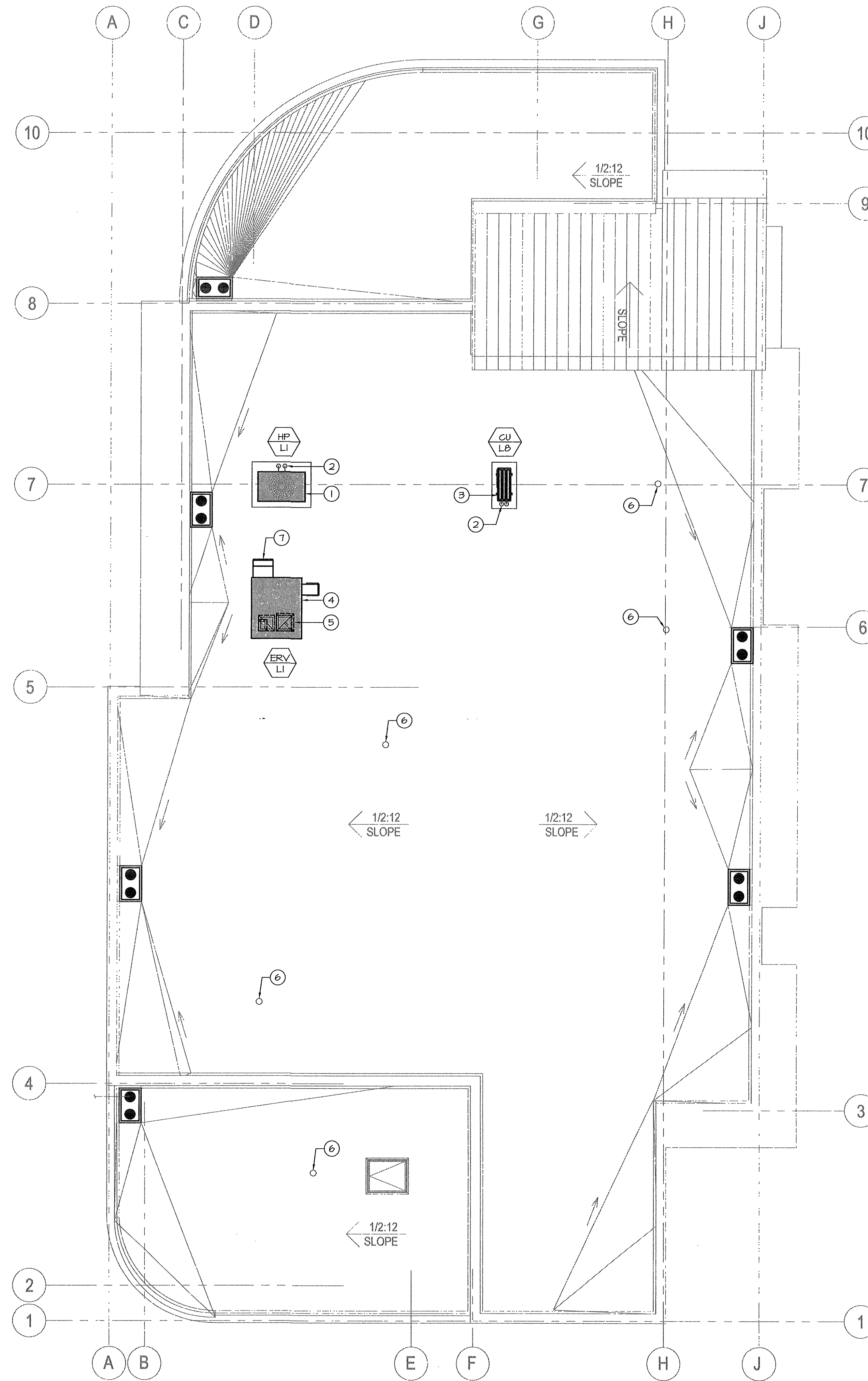
MECHANICAL ROOF PLAN SCALE: 3/16"=1'-0"
