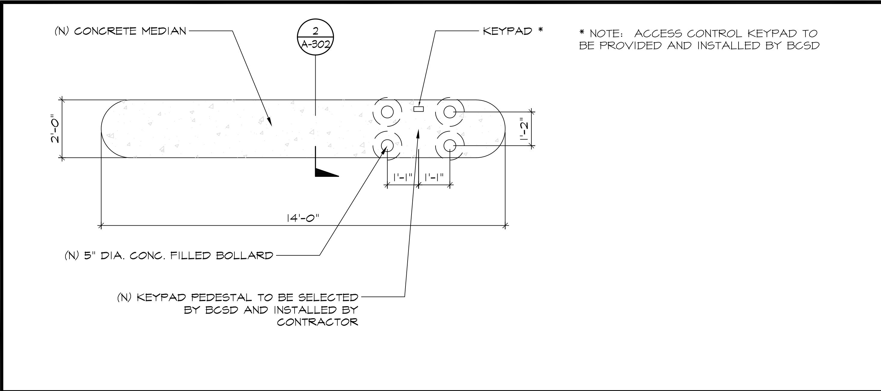
1 KEYPAD MEDIAN AT ENTRY SCALE: 1/2"=1'-0" (IN FEET)
