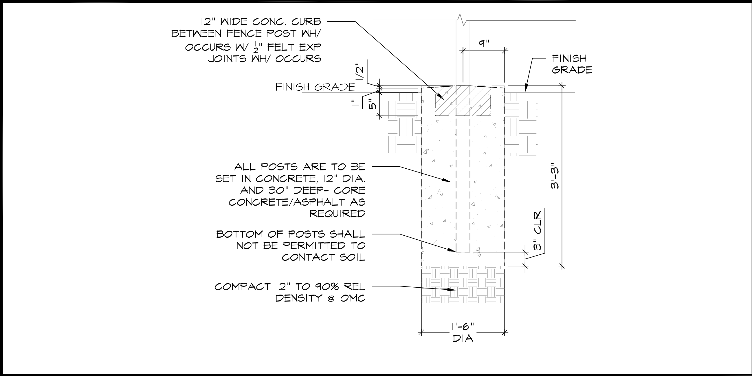
6 FENCING ELEVATION SCALE: 1/8"=1'-0" (IN FEET)
