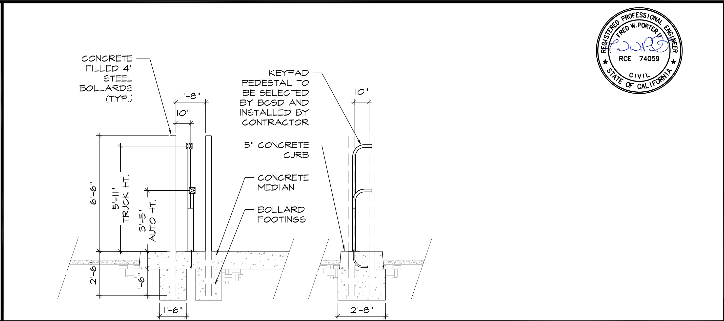
2 PEDESTAL BOLLARD DET. SCALE: 3/8"=1'-0" (IN FT)
