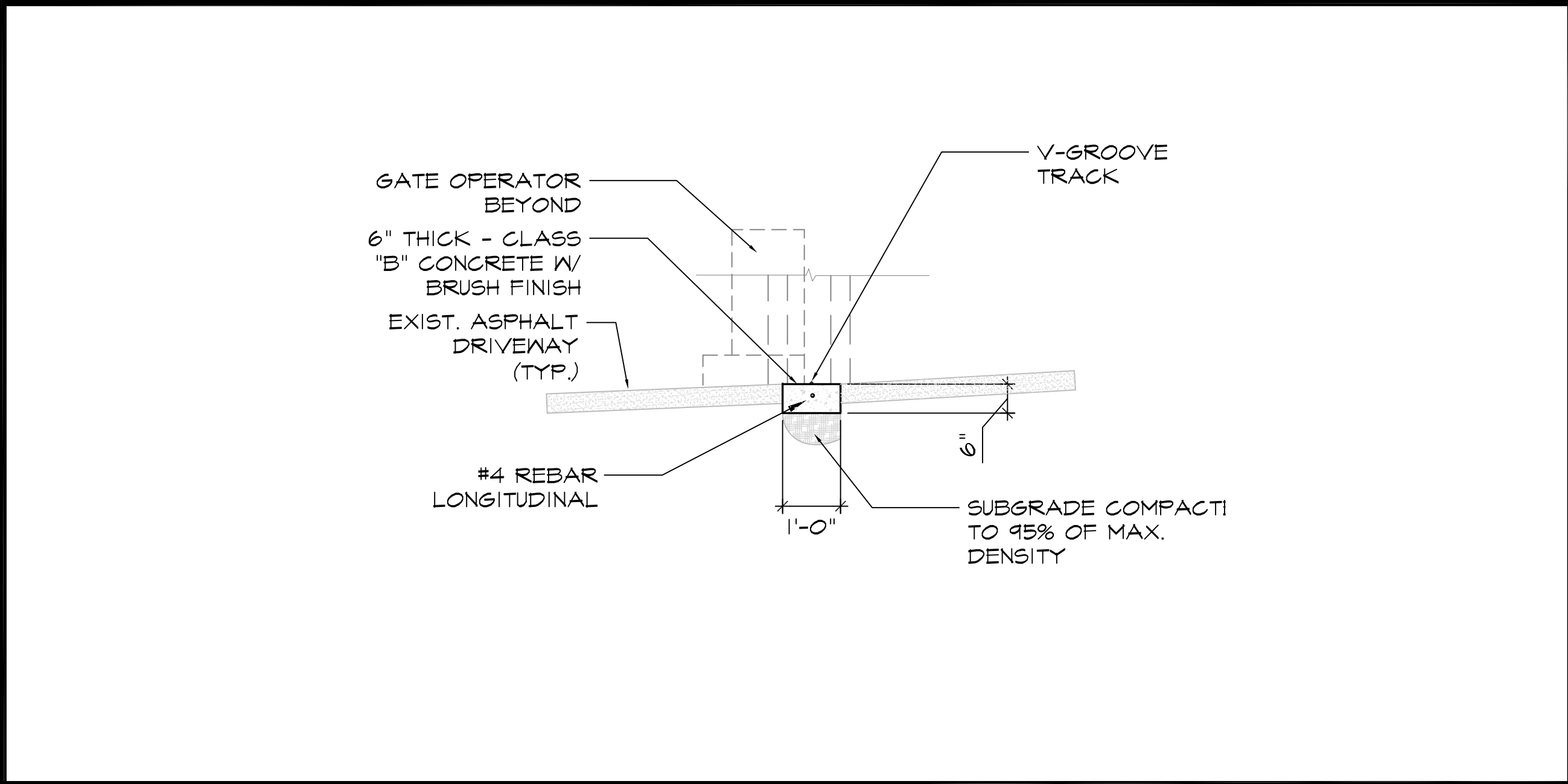
3 GATE TRACK SCALE: 1/2"=1'-0" (IN FEET)
